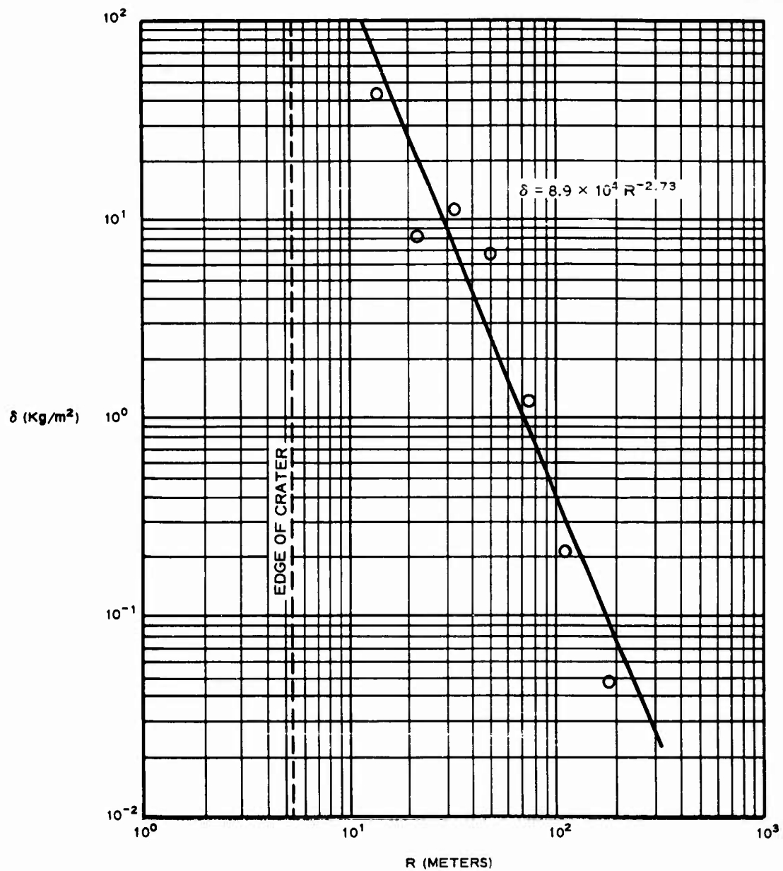
Figure A.7 Mass distribution ( \delta ) versus radial distance from GE ( R ) for the averages of White Tribe data.
