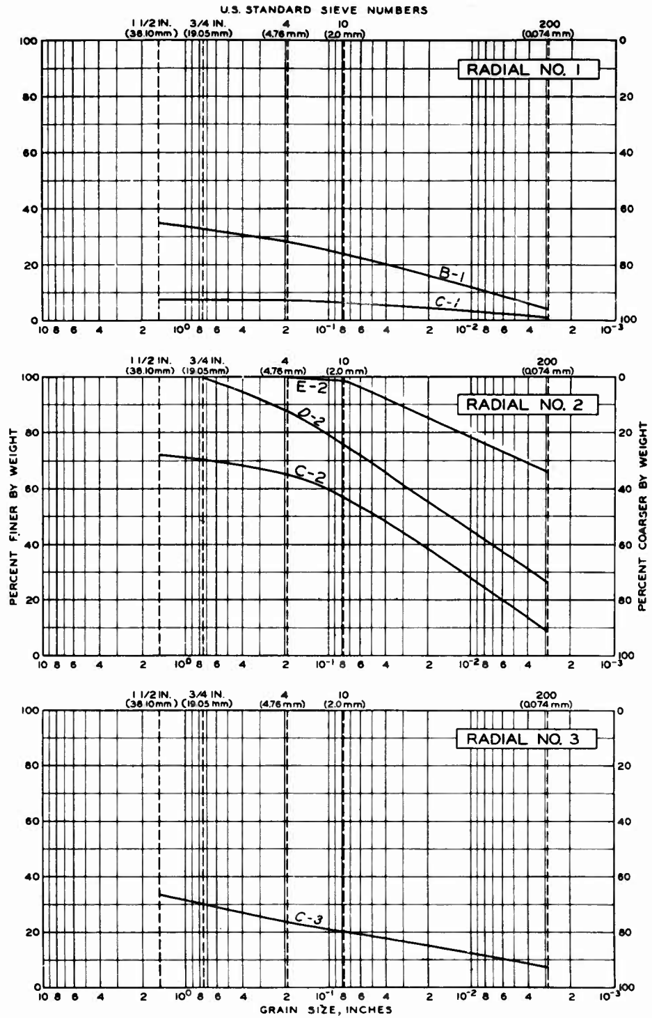
Figure 3.8 Grain-size distribution on radials 1, 2, and 3, Danny Boy.
