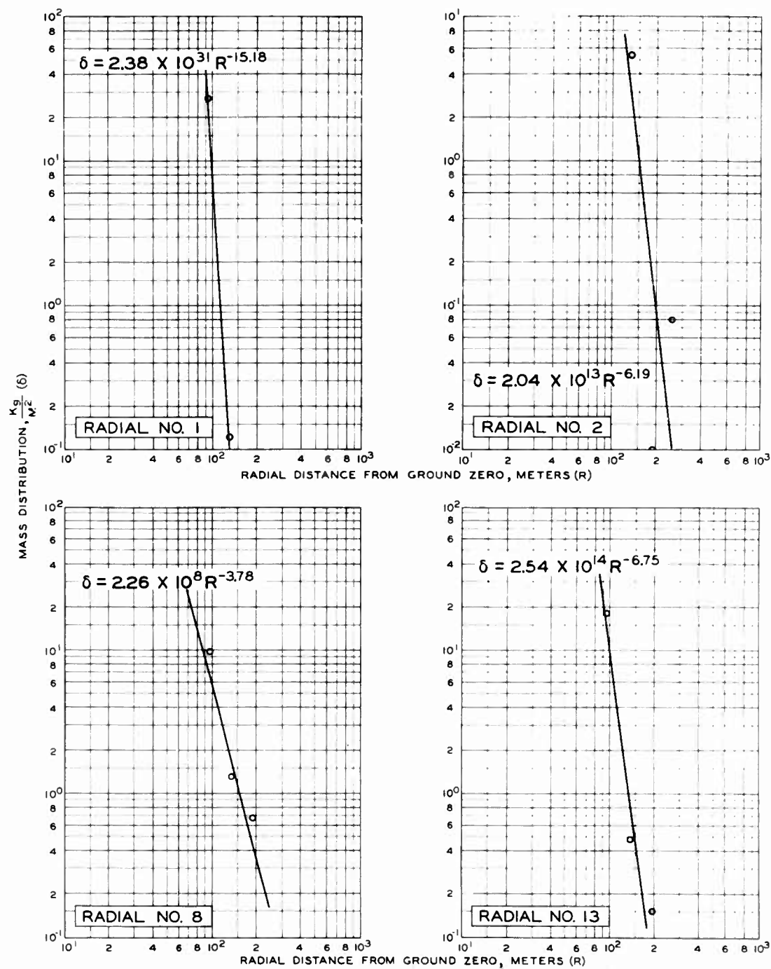
Figure 3.3 Logarithmic graphs of mass distribution versus radial distances from GZ for radials 1, 2, 8, and 13.
