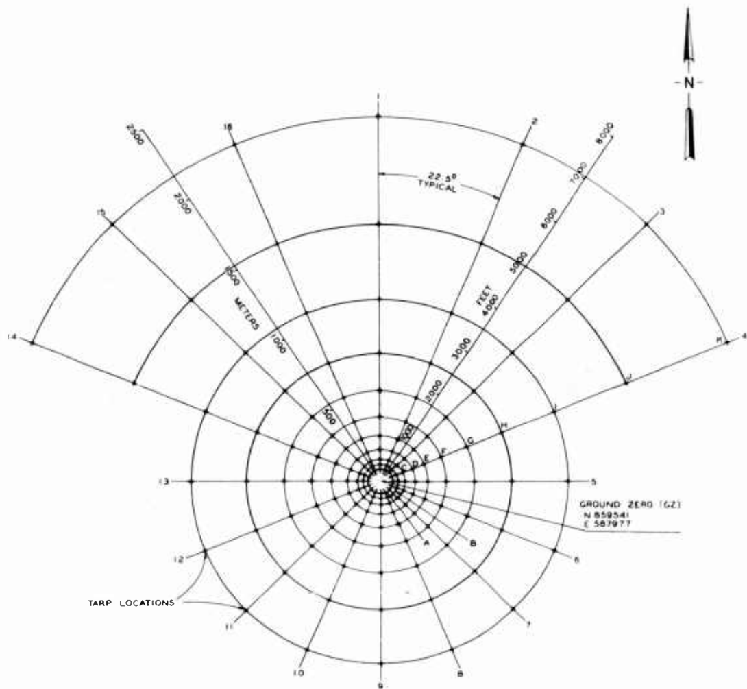
Figure 2.4 Tarpaulin array. Radial distances of rings from GZ are 220, 310, 440, 625, 880, 1250, 1770, 2500, 3540, 5000, and 7080 feet. Angular interval between radii equals 22.5 degrees.
