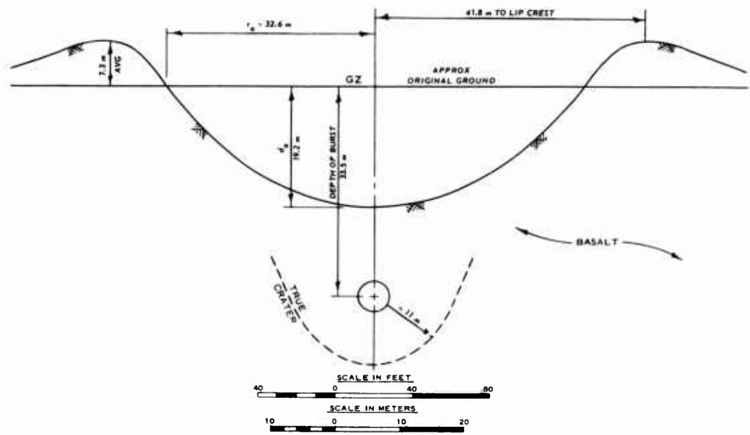
Figure 2.2 Shot geometry and crater dimensions, Danny Boy.
