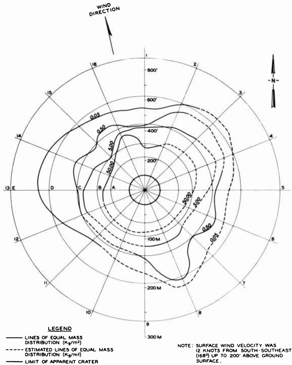
Figure 3.6 Mass distribution contours in \text{kg}/\text{m}^2 , Danny Boy.
