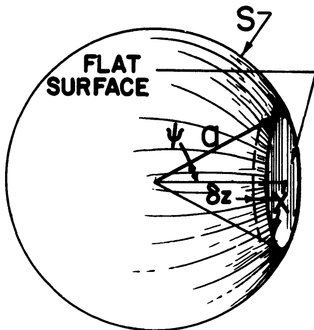
Fig. 1. Growth of circular facet on a spherical surface by removal of material from top of facet.
