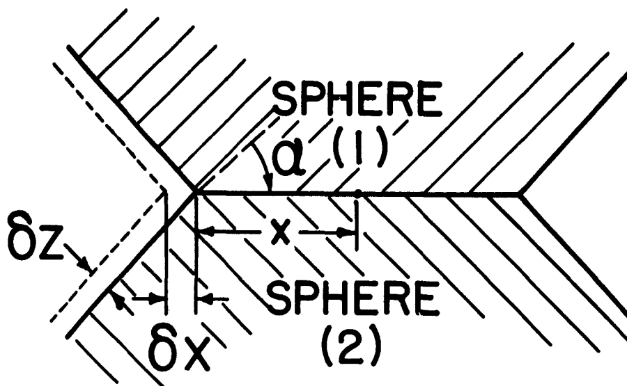
Fig. 2. Contact between spherical surfaces by parallel displacement of facets.
