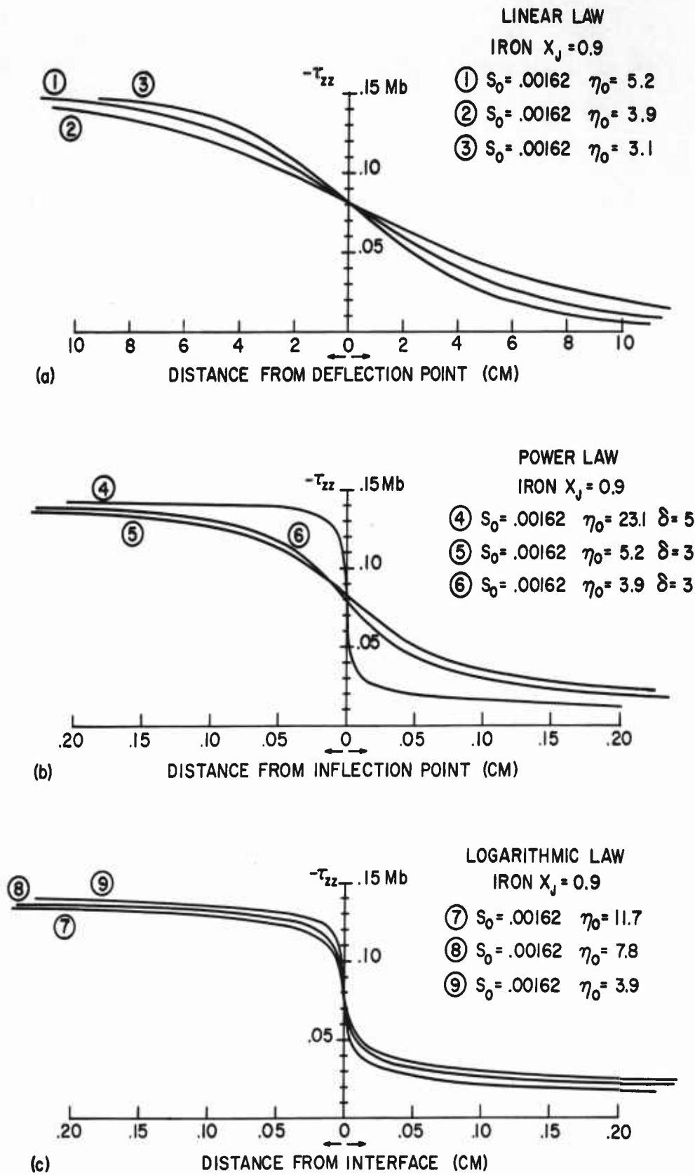
Figure 3. Calculated shock profiles in mild steel for a final compression ratio X_f = 0.9 when \mu is assumed to follow (a) linear law, (b) power law, (c) logarithmic law.
