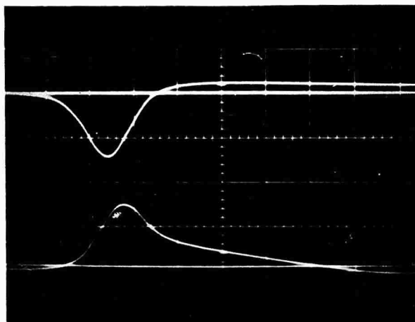
FIGURE 3: Typical h_{FE} of 2N331 response during SPRF Radiation Burst UPPER TRACE: Collector Current 2 ma/cm LOWFR TRACE: Base Current 50 ma/cm. Horizontal Sweep Speed - 50 \mu s/cm.
