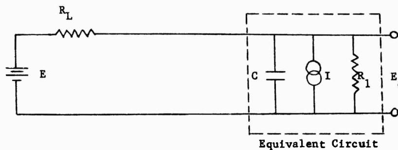
(a) Test Circuit and Equivalent Circuit of Thin Film Capacitor
