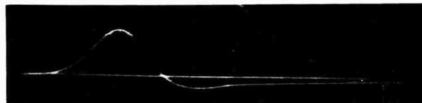
FIGURE 5: Typical I_{CEO} of 2N331 Response during SPRF Burst Collector Current 50 ma/cm with 100 \Omega Load Resistance. Horizontal Sweep Speed 50 \mu s/cm.
