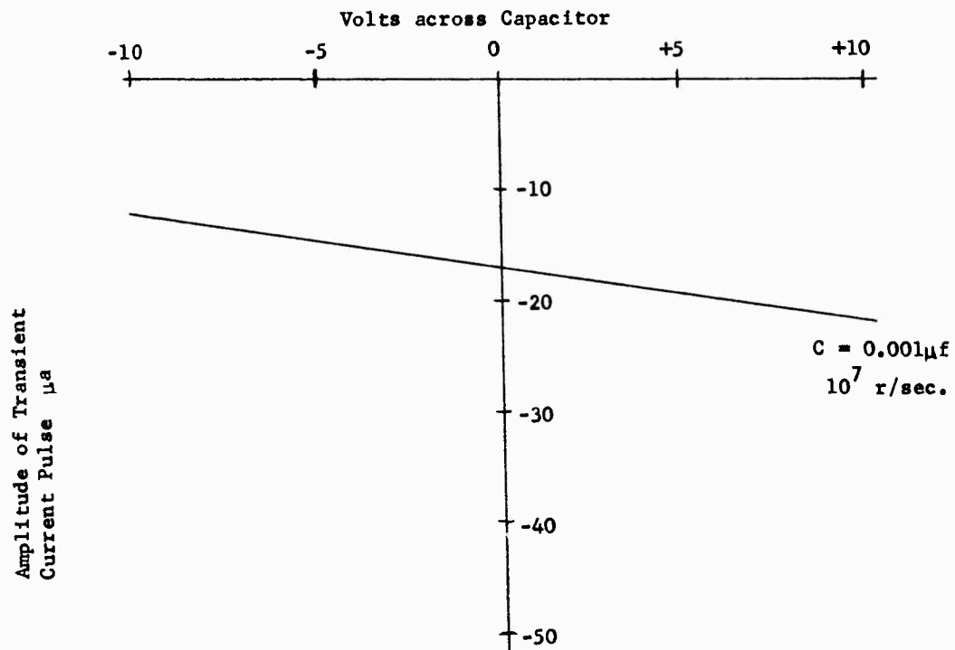
(b) Radiation Response of Thin Film Capacitor
