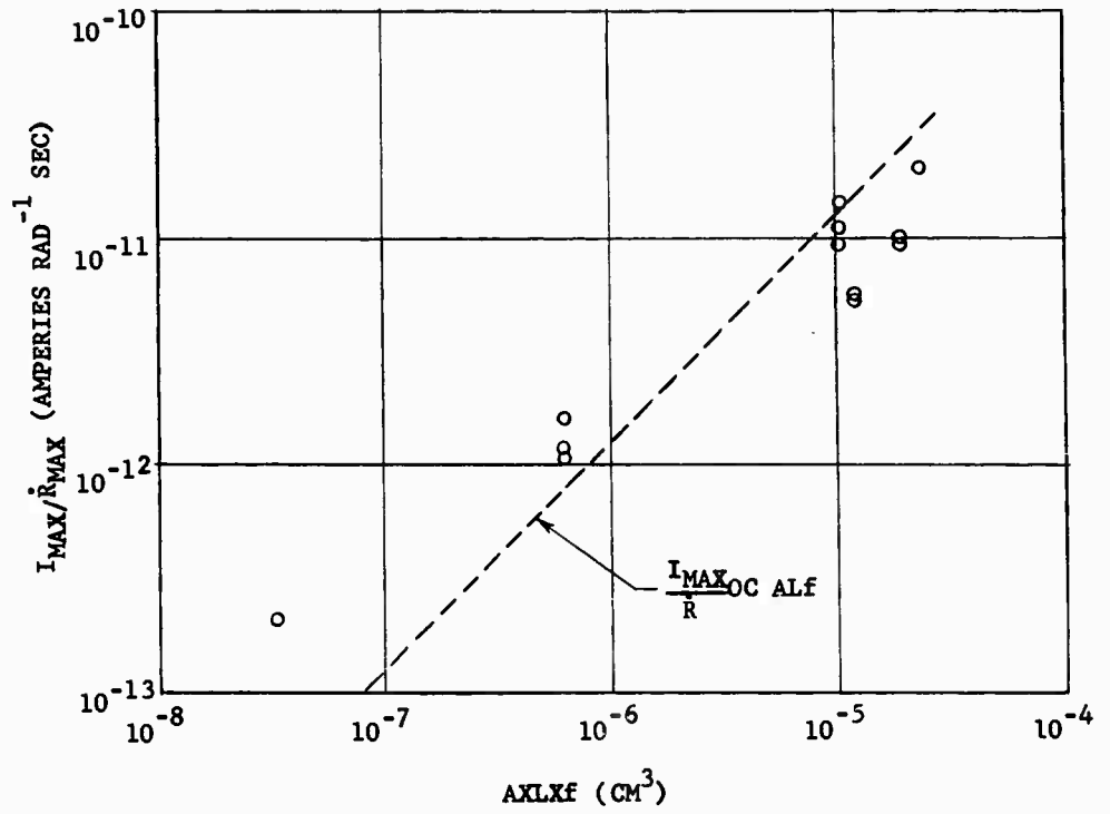
FIGURE 2: NORMALIZED LEAKAGE CURRENT AS A JUNCTION OF EFFECTIVE JUNCTION VOLUME
