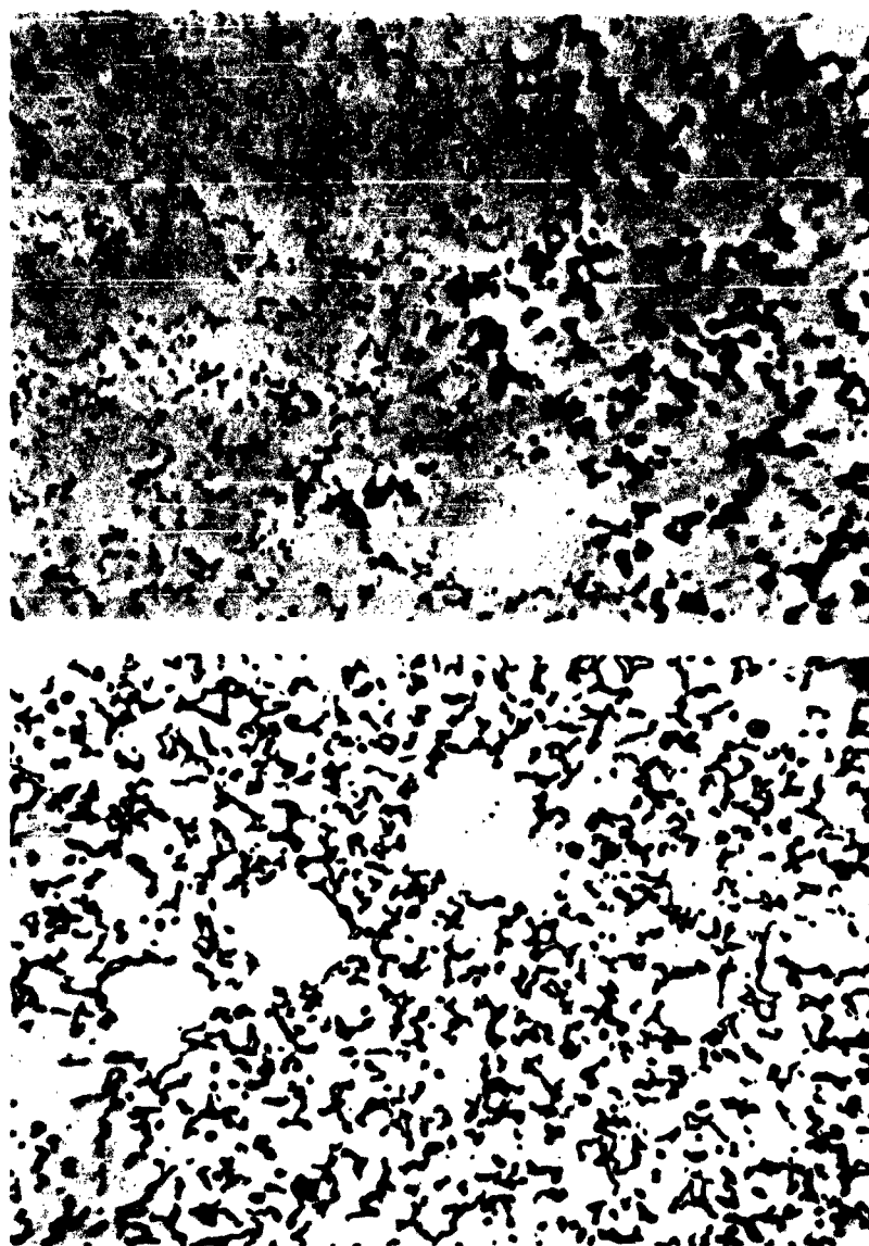
Fig. B8 - Interparticle "porosity" in section A of insert B-1 (CP-4 etch) 500X. (a) Adjacent to \text{Al}_2\text{O}_3 infiltrated region, (b) Interior of uninfiltated region.
