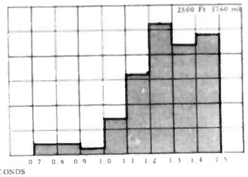
Figure 16. Distribution curves and histograms for the 0.3- to 1.5-sec noise at the surface and at 2500 ft (760 m) in the deep well, Orlando, Florida
