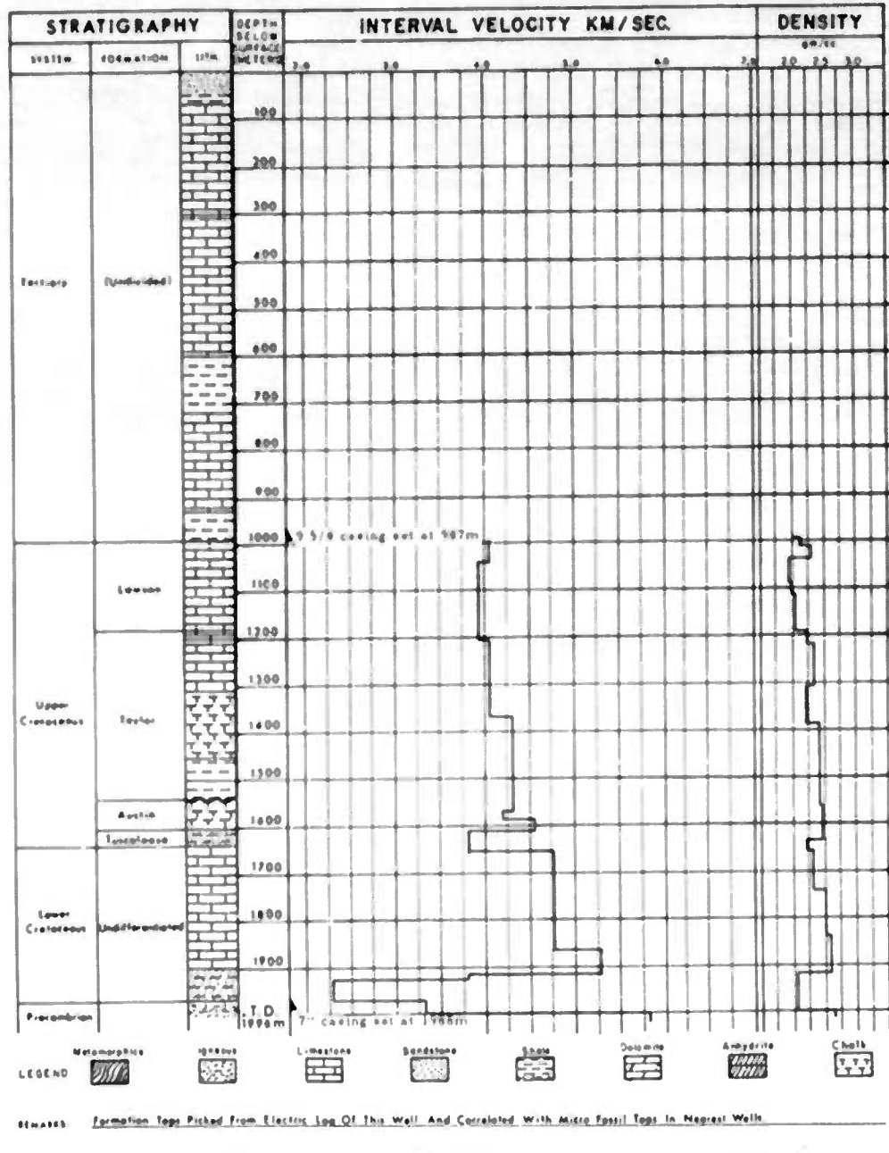
Figure 5. Stratigraphy and velocities (metric), Terry No. 1
