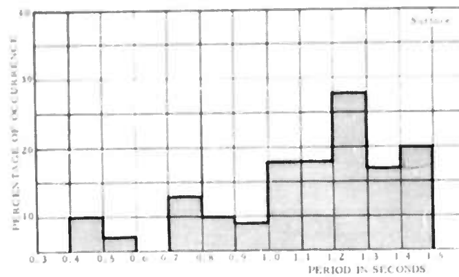
Figure 15. Distribution curves and histograms for the 0.3- to 1.5-sec noise at the surface and at 1500 ft (450 m) in the deep well, Orlando, Florida
