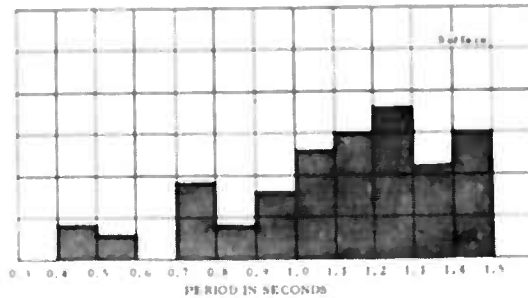
Figure 18. Distribution curves and histograms for the 0.3- to 1.5-sec noise at the surface and at 4181 ft (1270 m) in the deep well, Orlando, Florida
