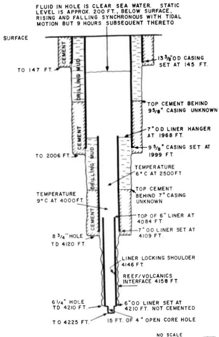
Figure 8. Casing diagram, Eniwetok E-1
