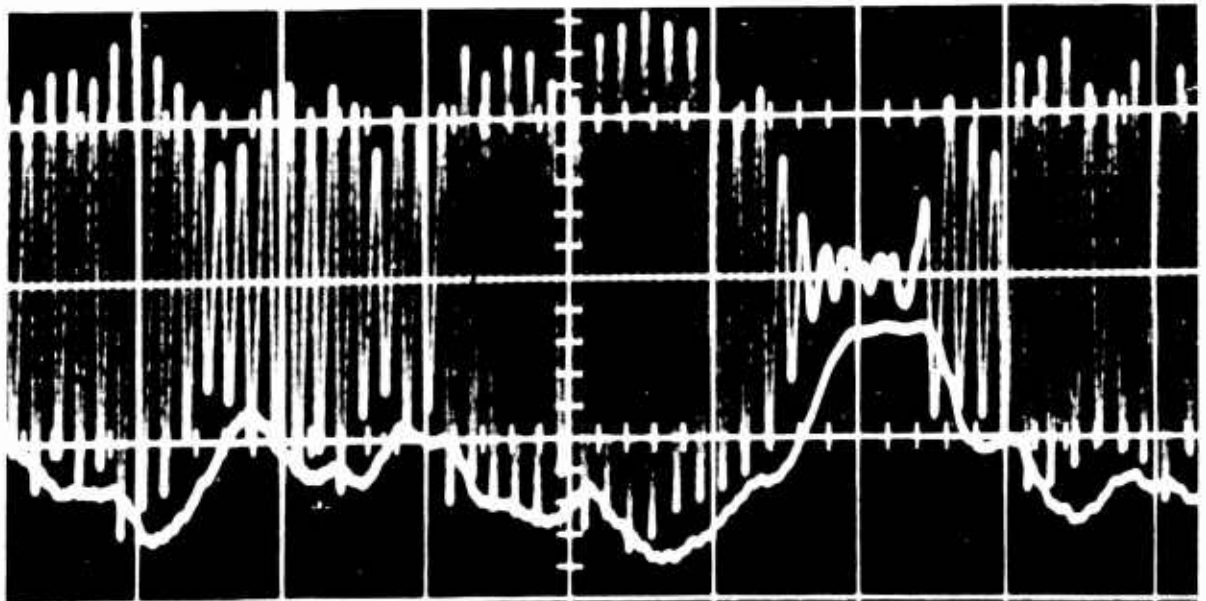
Fig. 14. Oscilloscope traces of the input and output of the envelope circuit shown simultaneously.
