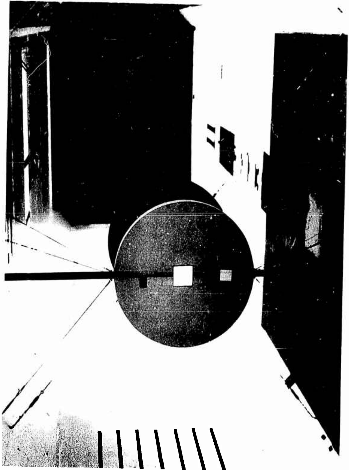
Fig. 7. d = 22 in., h = 2\text{-}5/8 in. Styrofoam disk mounted in tunnel with 22 in. diam plywood disk downstream.
