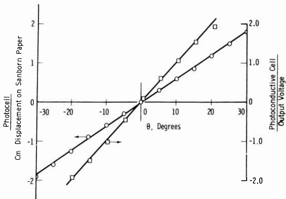
Fig. 4. Typical calibration data for the photocell and photoconductive angular position sensors.
