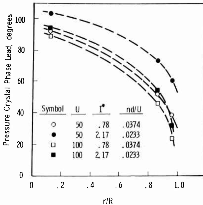
Fig. 27. Pressure phase lead as a function of position of the upstream face of a 0.92 ft diam disk in free oscillation. Pressure ports are located on a diameter normal to the oscillation axis.
