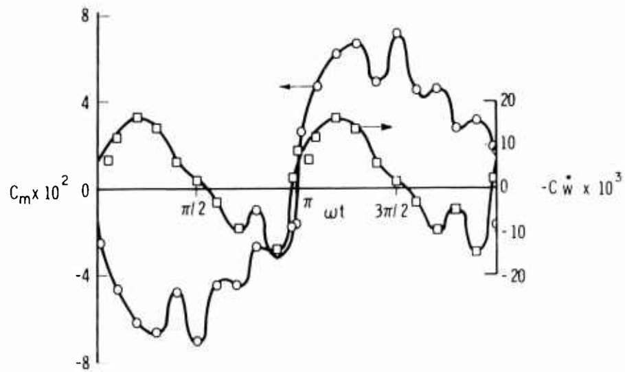
Fig. 22. Aerodynamic moment and work rate coefficients during one cycle of forced oscillation of a Styrofoam disk, d = 22 in., h = 2\text{-}5/8 in., \theta_0 = 0.707 rad, \omega = 12.7 rad/sec, U = 48.4 fps, Re = 5.40 \times 10^5 , nd/U = 7.66 \times 10^{-2} .
