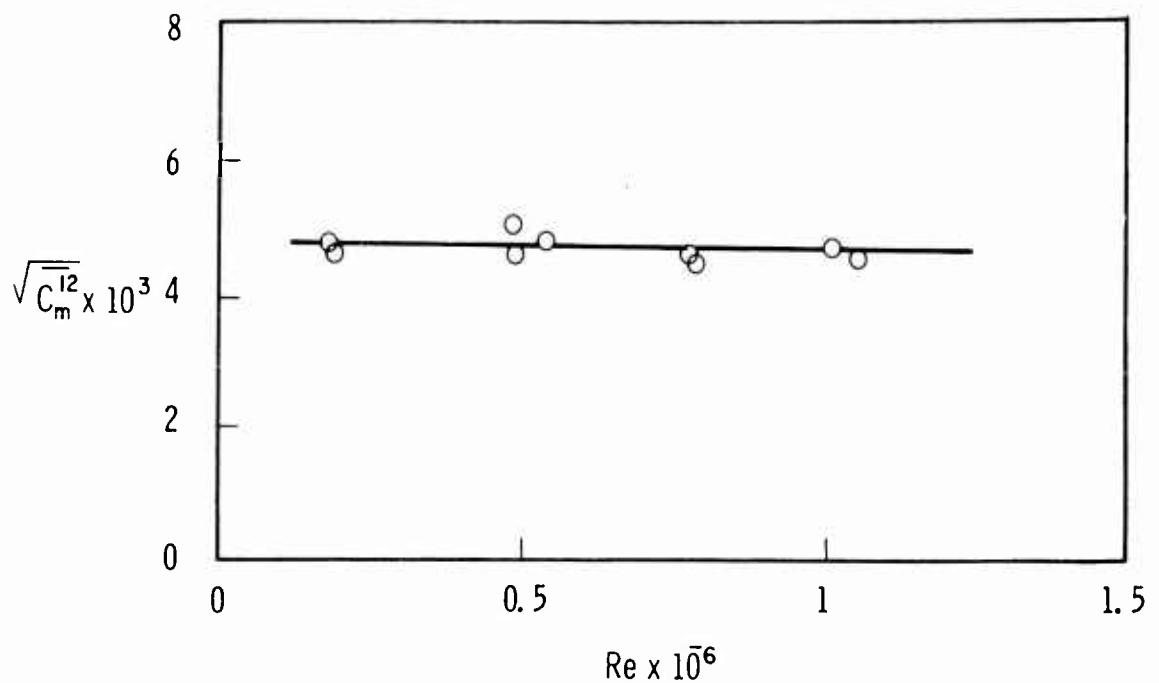
Fig. 40. Root mean square moment coefficient for the Styrofoam disk normal to flow ( \theta = 0 ); d = 22 in., h = 2\text{-}3/8 in.
