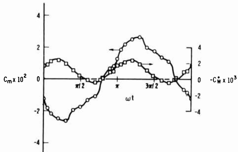
Fig. 23. Aerodynamic moment and work rate coefficients during one cycle of forced oscillation of a Styrofoam disk, d = 22 in., h = 2\text{-}5/8 in., \theta_0 = 0.147 rad, \omega = 37.1 rad/sec, U = 94.5 fps, Re = 10.0 \times 10^5 , nd/U = 11.42 \times 10^{-2} .
