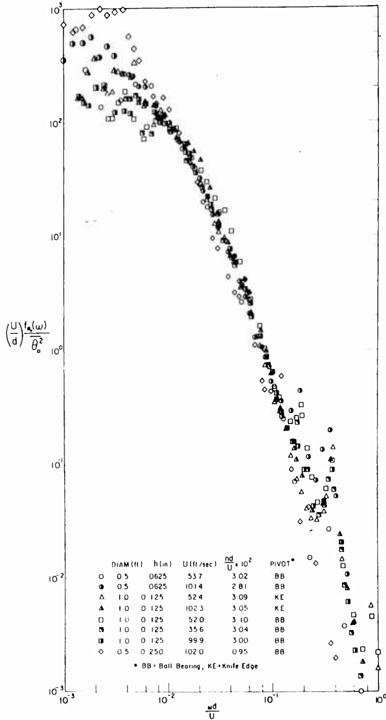
Fig. 18. Power spectra of the envelope amplitude, \theta_0 , for several disks in free oscillation.
