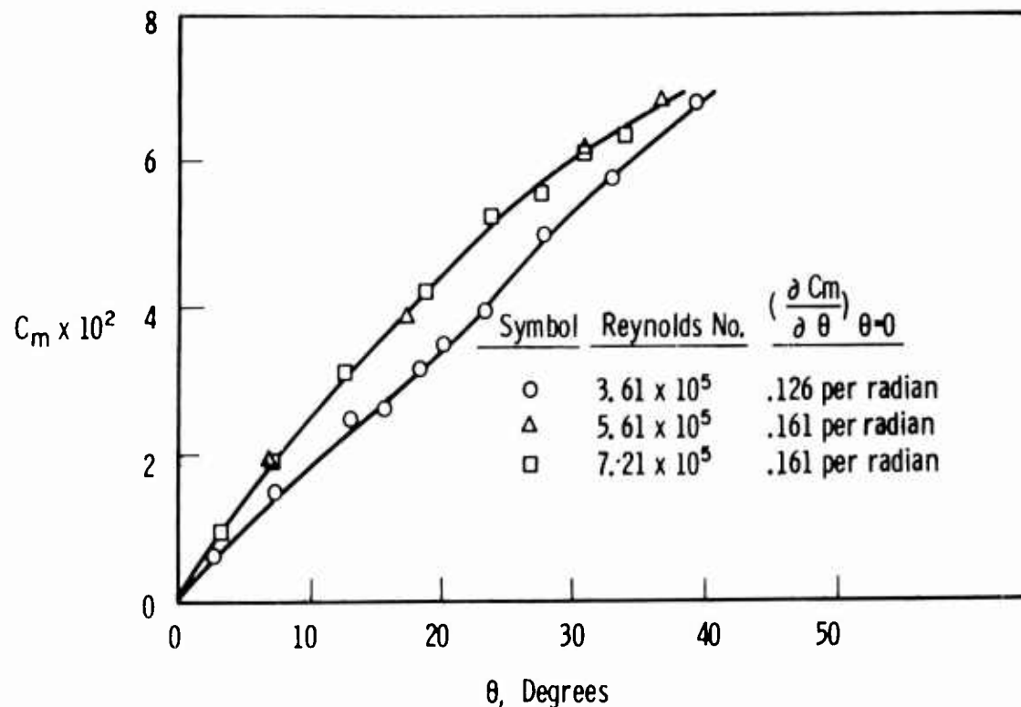
Fig. 9. Static moment coefficient, C_m , vs. disk deflection angle, \theta , Styrofoam disk, d = 22 in., h = 2\text{-}5/8 in.
