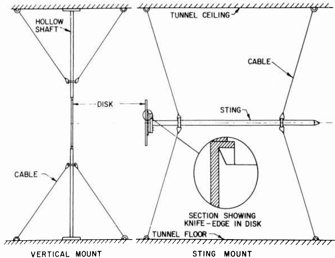
Fig. 2. Sketch showing wind tunnel mounting methods for free oscillation tests.
