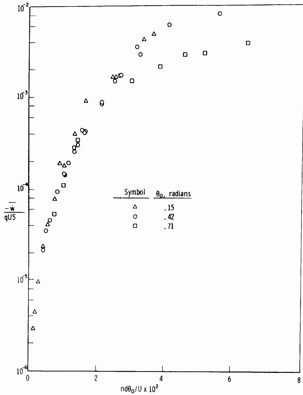
Fig. 28. Dimensionless average work rate as a function of nd\theta_0/U for three amplitudes.
