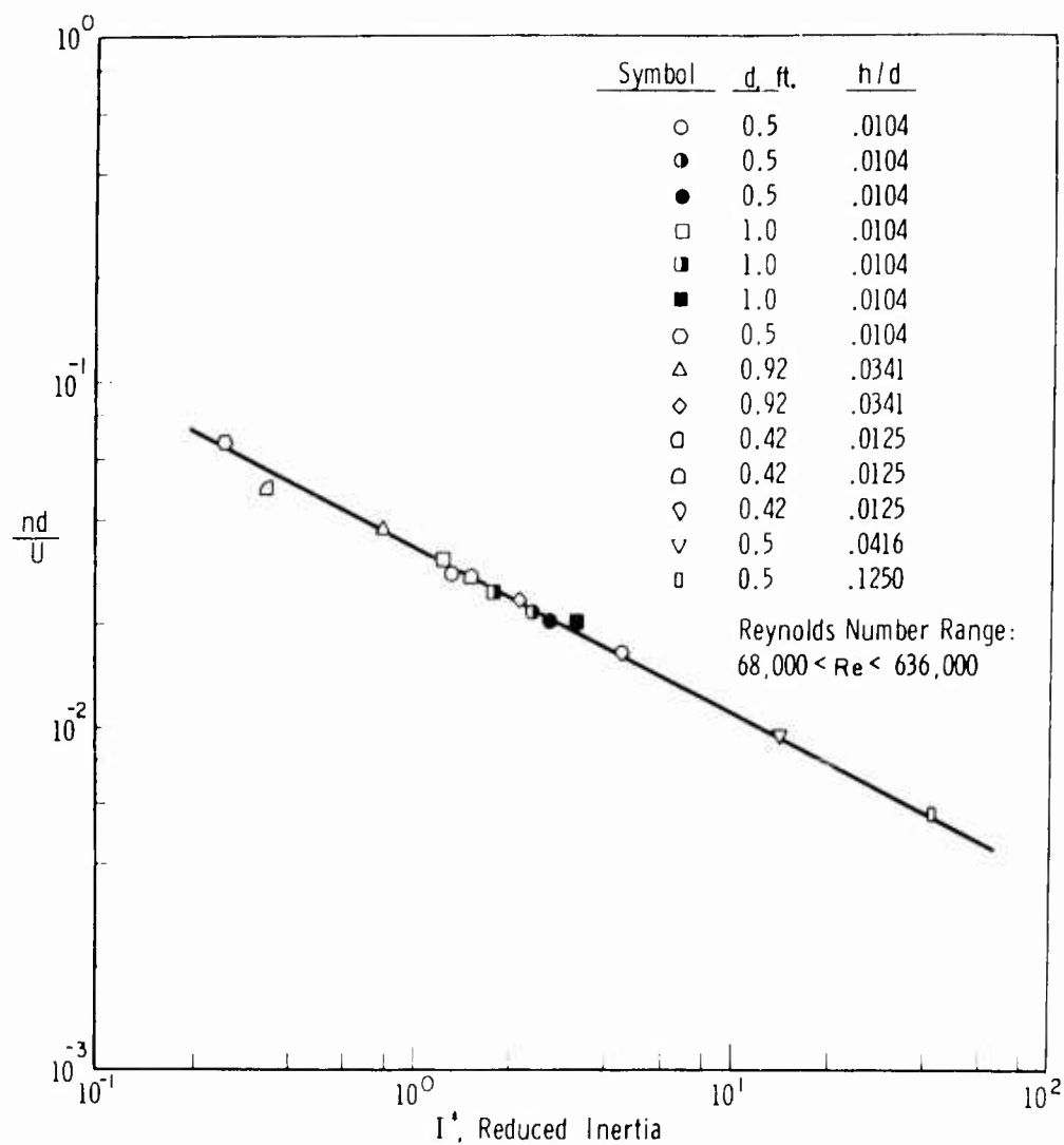
Fig. 8. Reduced frequency, nd/U , vs. reduced inertia, I^* , for free oscillation.
