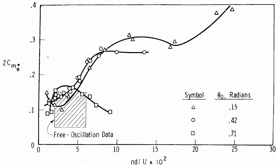
Fig. 29. Forced oscillation damping coefficient vs. nd/U for three amplitudes.
