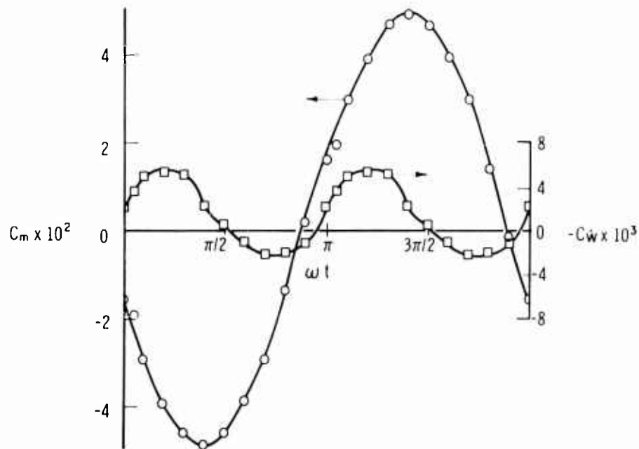
Fig. 24. Aerodynamic moment and work rate coefficients during one cycle of forced oscillation of a Styrofoam disk, d = 22 in., h = 2\text{-}3/8 in., \theta_0 = 0.425 rad, \omega = 20.6 rad/sec U = 95 fps, Re = 9.96 \times 10^5 , nd/U = 6.32 \times 10^{-2} .
