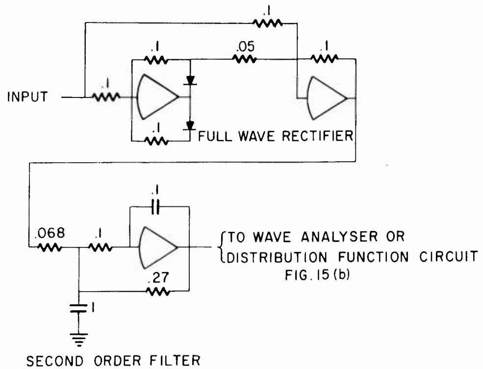
Fig. 13. Analog computer circuit used to obtain the envelope, \theta_0 , of the disk oscillations.
