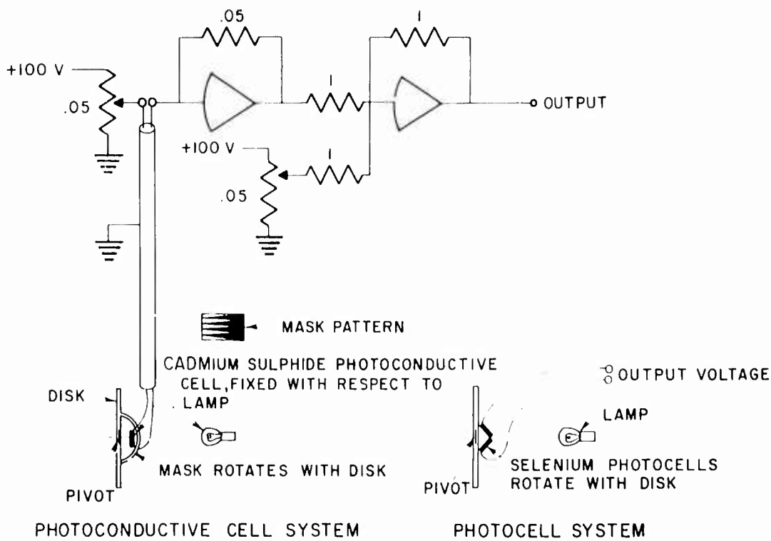
Fig. 3. Photocell and photoconductive cell angular position systems.
