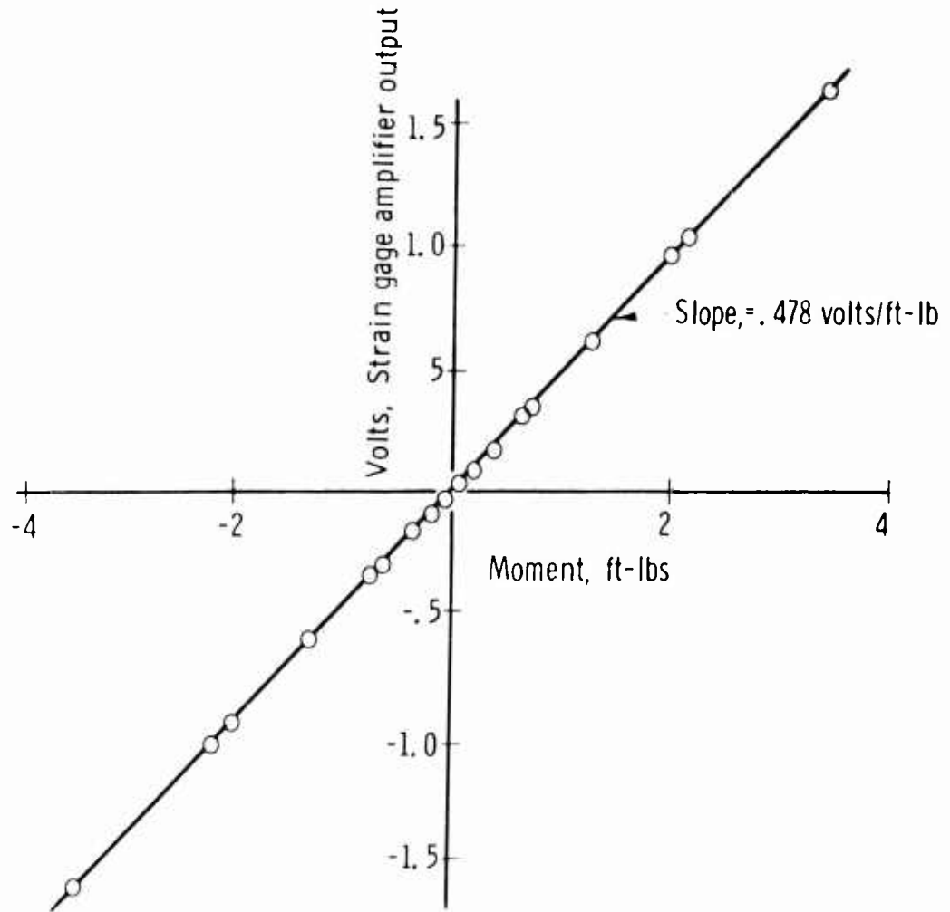
Fig. 6. Calibration of moment balance.
