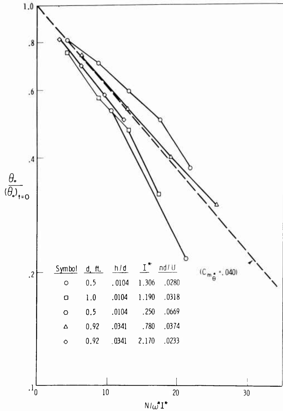
Fig. 10. Average damping for several disks in free oscillation after release from an initial angle.
