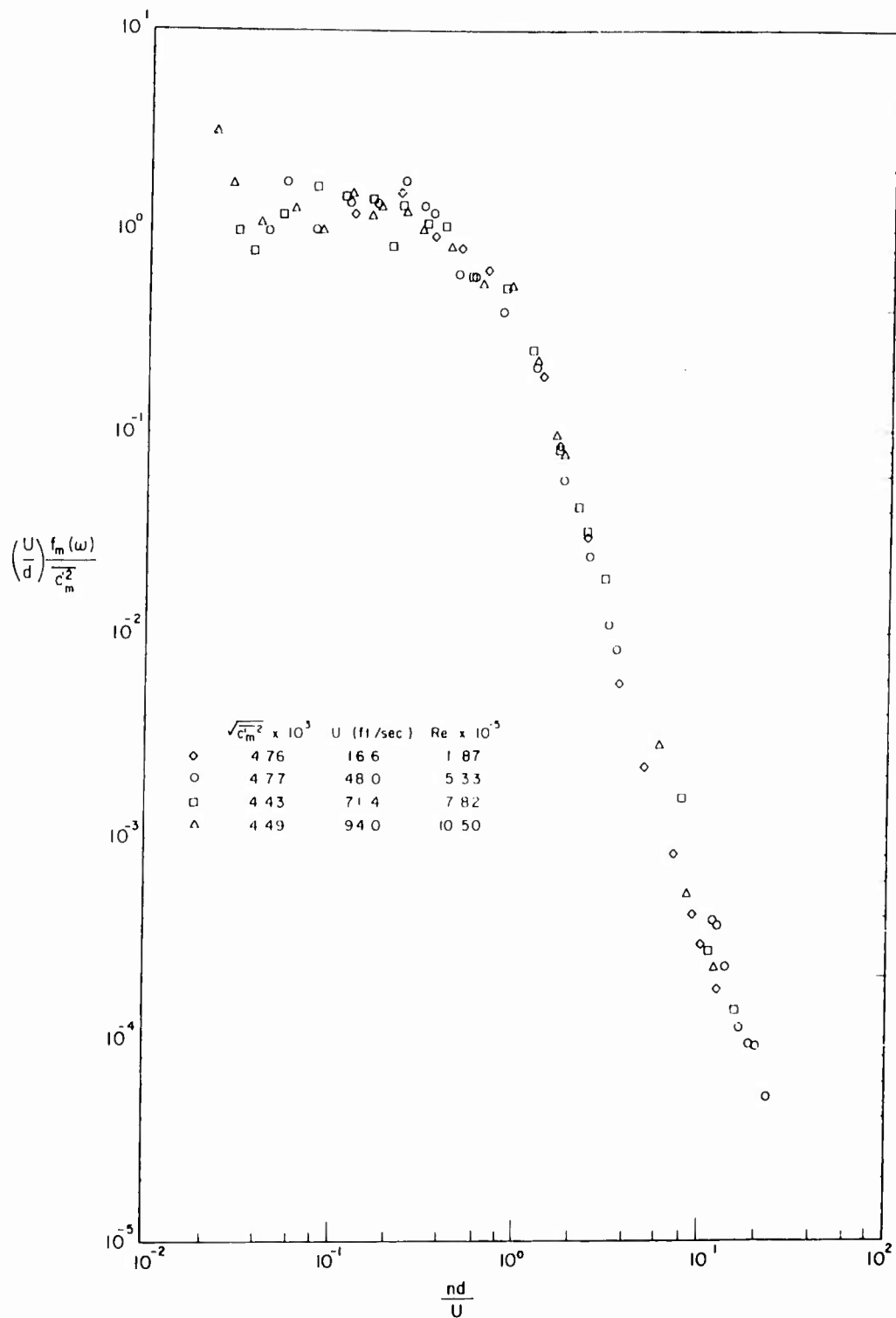
Fig. 51. Power spectra of the fluctuating aerodynamic moment acting on the Styrofoam disk normal to flow ( \theta = 0 ); d = 22 in., h = 2\text{-}3/8 in.
