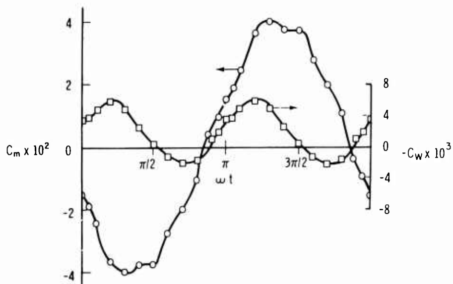
Fig. 24. Aerodynamic moment and work rate coefficients during one cycle of forced oscillation of a Styrofoam disk, d = 22 in., h = 2\text{-}3/8 in., \theta_0 = 0.425 rad, \omega = 20.6 rad/sec U = 95 fps, Re = 9.96 \times 10^5 , nd/U = 6.32 \times 10^{-2} .
