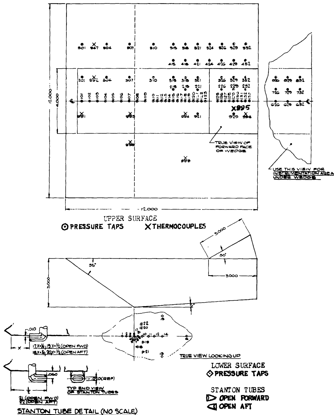
Fig. 4 Model Instrumentation
