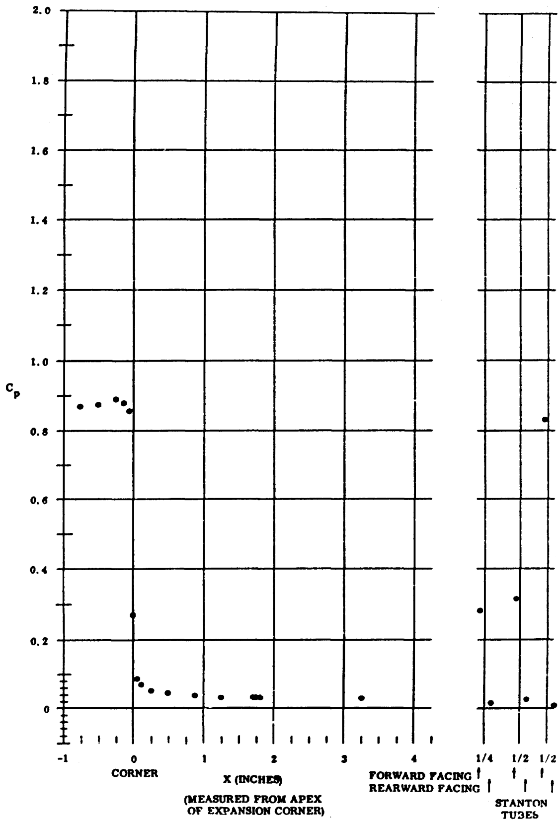
Fig. 48 Pressure Coefficient Data Plots (maximum coolant flow rate for upper surface); \alpha \approx 0^\circ and Re_{\infty}/ft = 3,300,000
