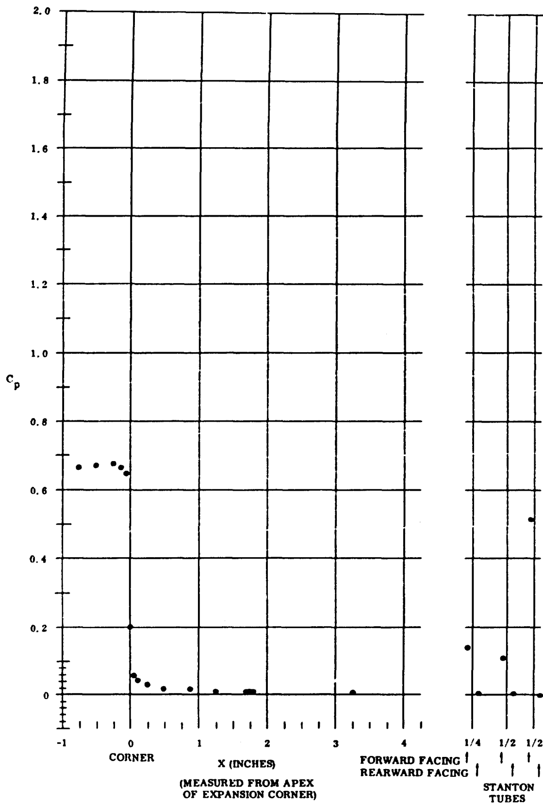
Fig. 40 Pressure Coefficient Data Plots (medium coolant flow rate for upper surface); \alpha = -5^\circ and Re_\infty/ft = 3,300,000
