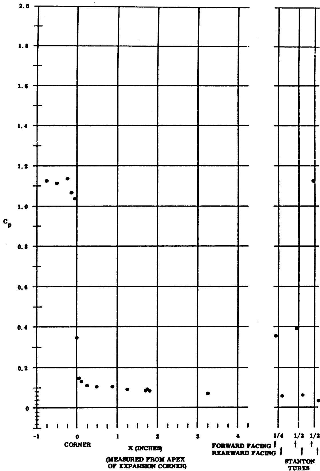
Fig. 50 Pressure Coefficient Data Plots (maximum coolant flow rate for upper surface); \alpha = +5^\circ and Re_{in}/ft = 1,100,000
