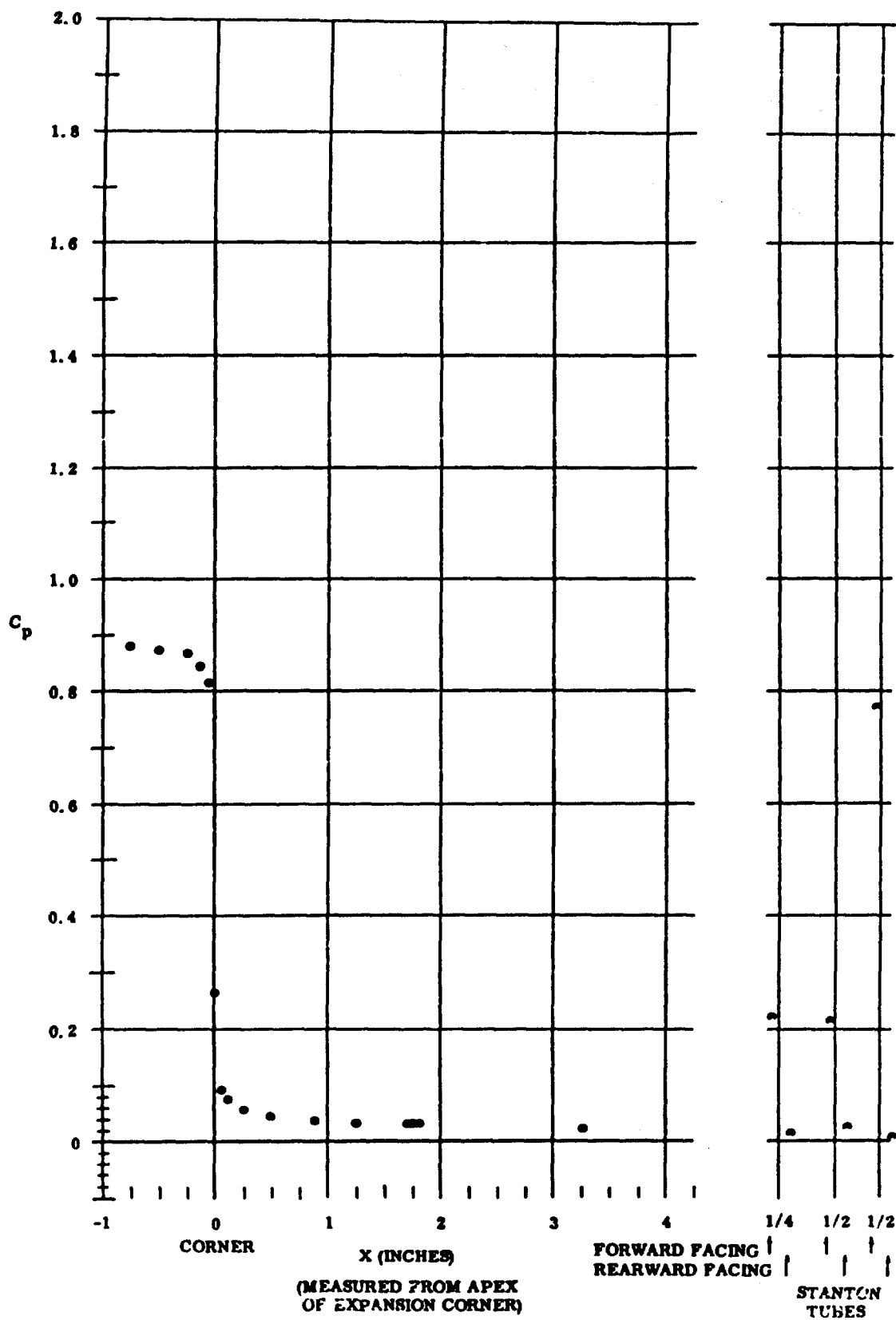
Fig. 44 Pressure Coefficient Data Plots (no coolant flow for upper surface); \alpha = 0^\circ and Re_{\mu}/ft = 2,200,000
