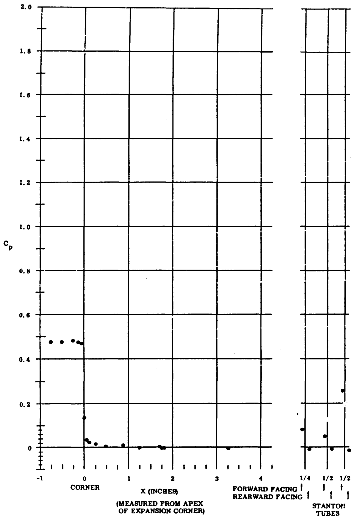
Fig. 36 Pressure Coefficient Data Plots (maximum coolant flow rate for upper surface); \alpha = -10^\circ and Re_{\mu}/ft = 3,300,000
