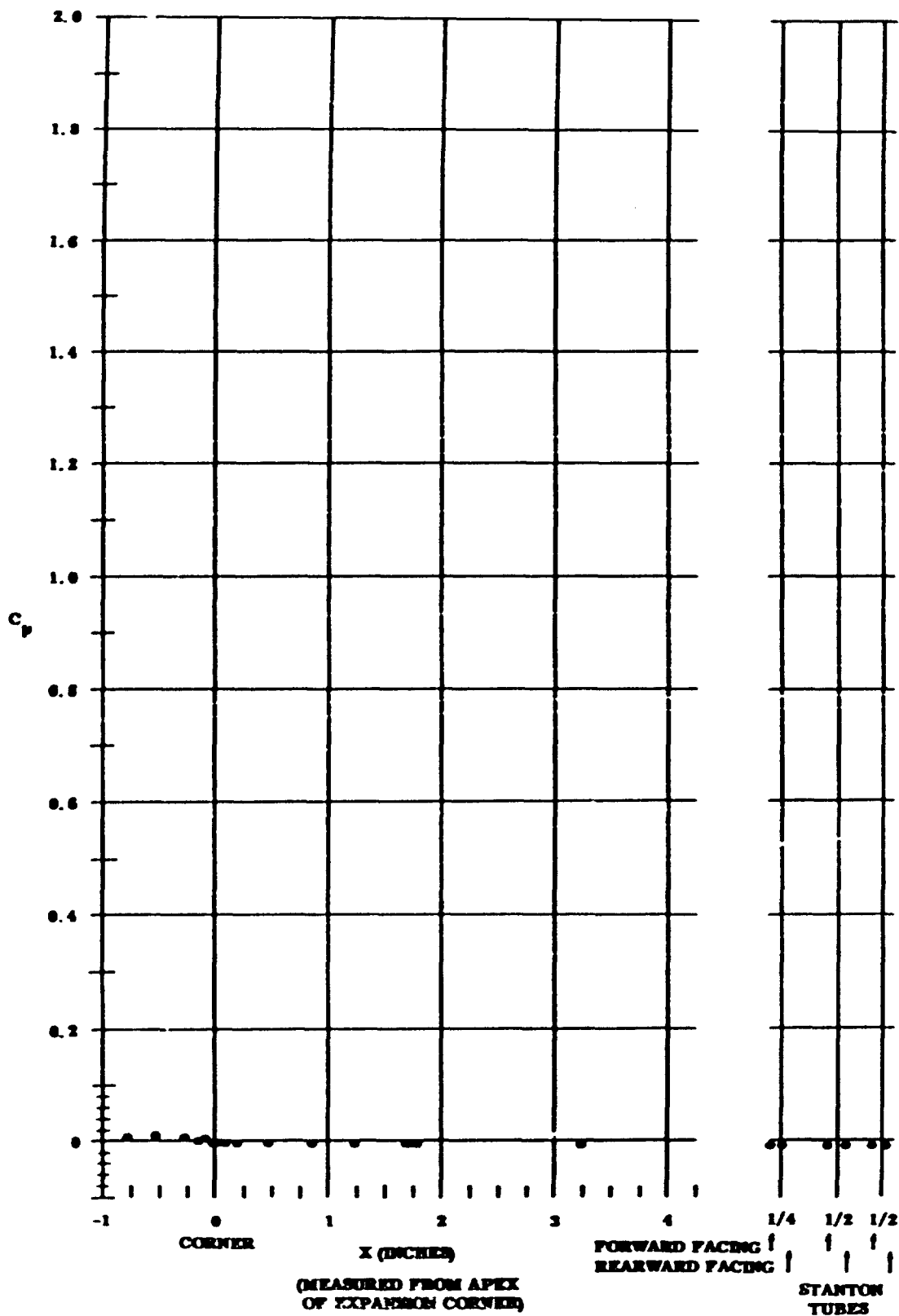
Fig. 19 Pressure Coefficient Data Plots (no coolant flow for upper surface); \alpha = -35^\circ and Re_{\infty}/ft = 3,300,000
