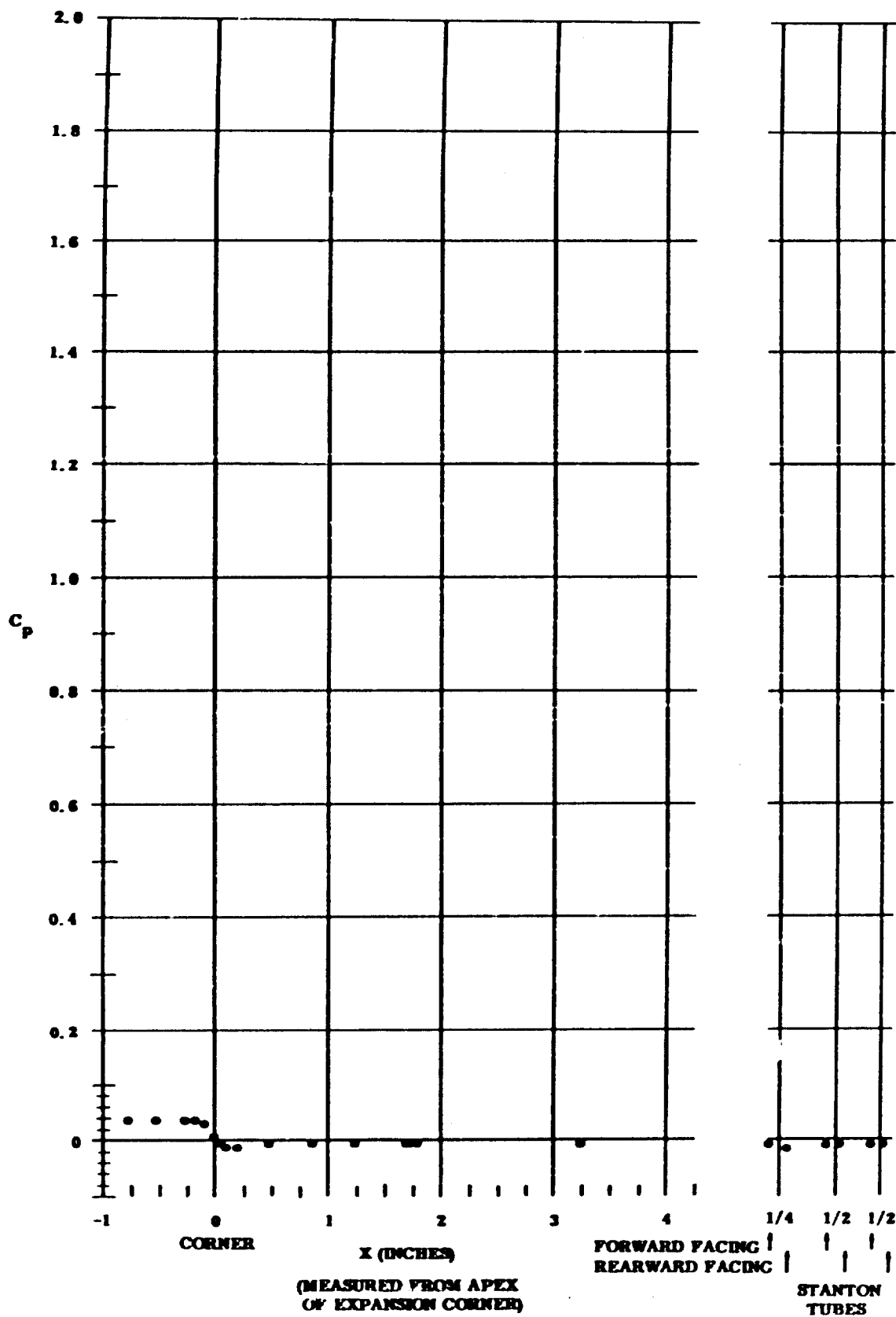
Fig. 23 Pressure Coefficient Data Plots (maximum coolant flow rate for upper surface); \alpha = -30^\circ and Re_{\rho}/ft = 3,300,000
