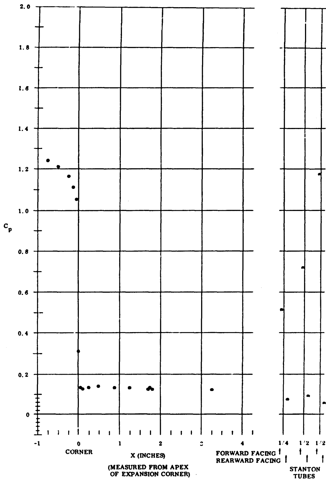
Fig. 53 Pressure Coefficient Data Plots (maximum coolant flow rate for upper surface); \alpha = +10^\circ and Re_{in}/ft = 3,300,000
