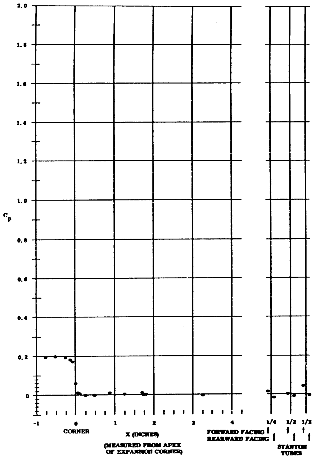
Fig. 26 Pressure Coefficient Data Plots (no coolant flow for upper surface); \alpha = -20^\circ and Re_{\text{ft}} = 1,100,000
