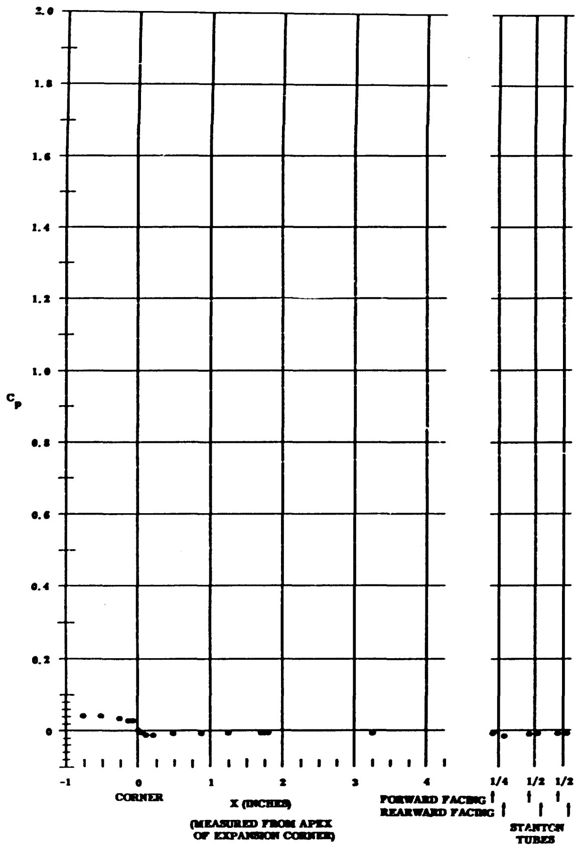
Fig. 22 Pressure Coefficient Data Plots (no coolant flow for upper surface); \alpha = -30^\circ and Re_{\text{ft}} = 3,300,000
