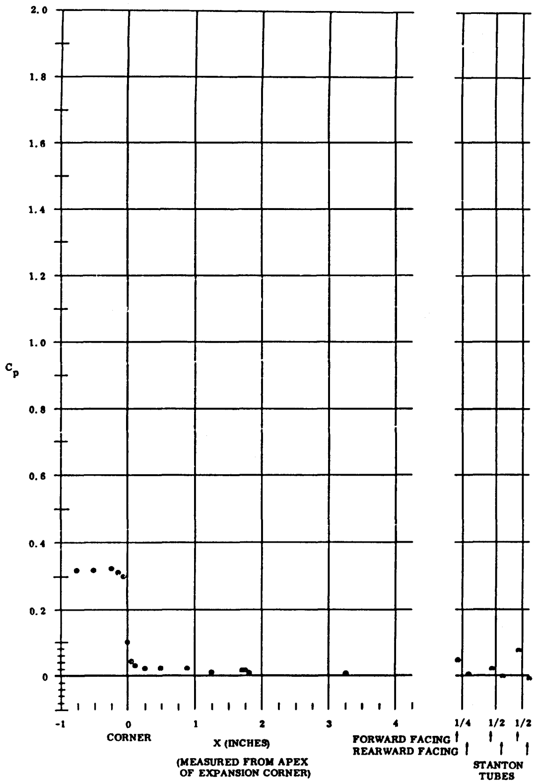
Fig. 29 Pressure Coefficient Data Plots (maximum coolant flow rate for upper surface); \alpha = -15^\circ and Re_\infty/ft = 1,100,000
