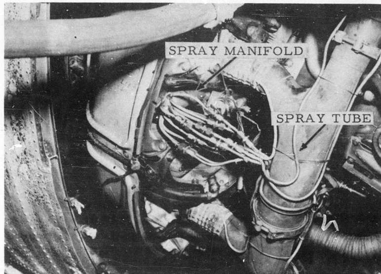
Figure 1A. Spray Distribution Tube Layout With the shroud removed, the spray tube layout and spray manifold are visible on the actual test aircraft (postcrash photo).
