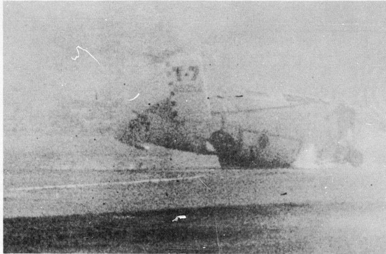
23K Burning fuel vapors in the forward portion of the plenum chamber and fuel tank area are starting to spout from the access doors and the skin rupture. Time: 1.5652 seconds after impact.
