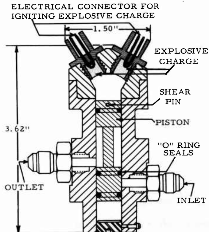
Figure 5. Explosive-Operated Valve.
