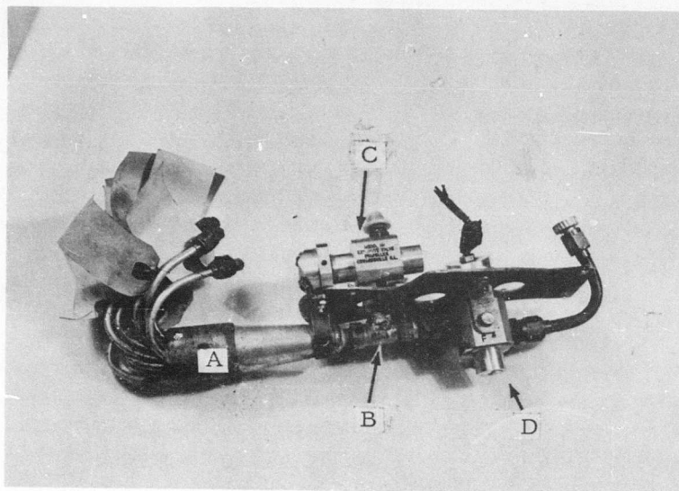
Figure 3A. Spray Distribution Manifold. Details identified by arrows are (A) aspirator (B) mixing chamber (C) explosive-actuated valve for the water (D) explosive-actuated valve for nitrogen.
