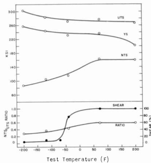
Figure 2. 600 F Temper
