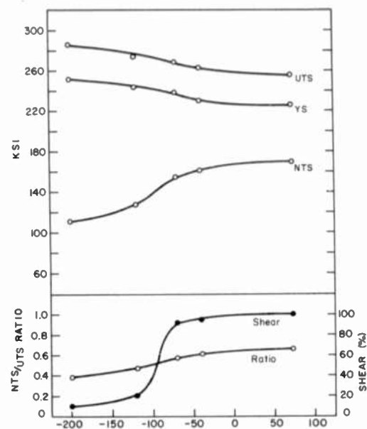
Figure 3. 800 F Temper
