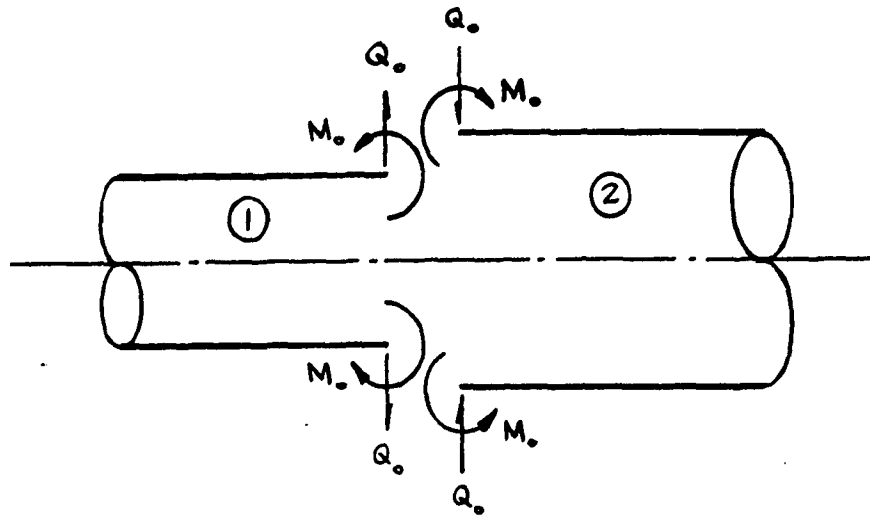
Fig. 4.1.2. Forces and Moments at the Junction of the Two Long Unequal Thickness Circular Cylindrical Shells.
