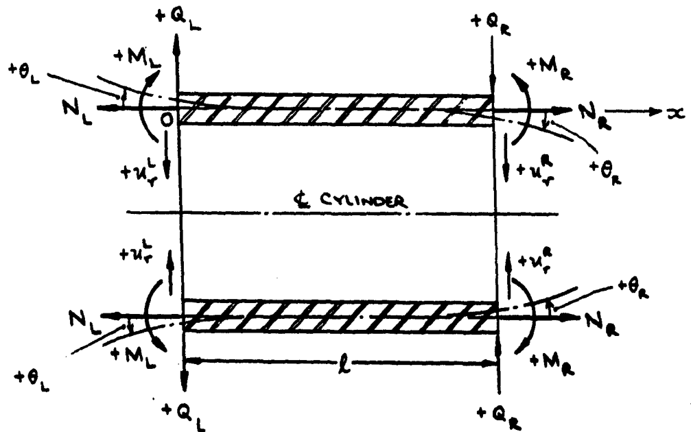
Fig. A.2.1 - Coordinate System and Signs Convention
