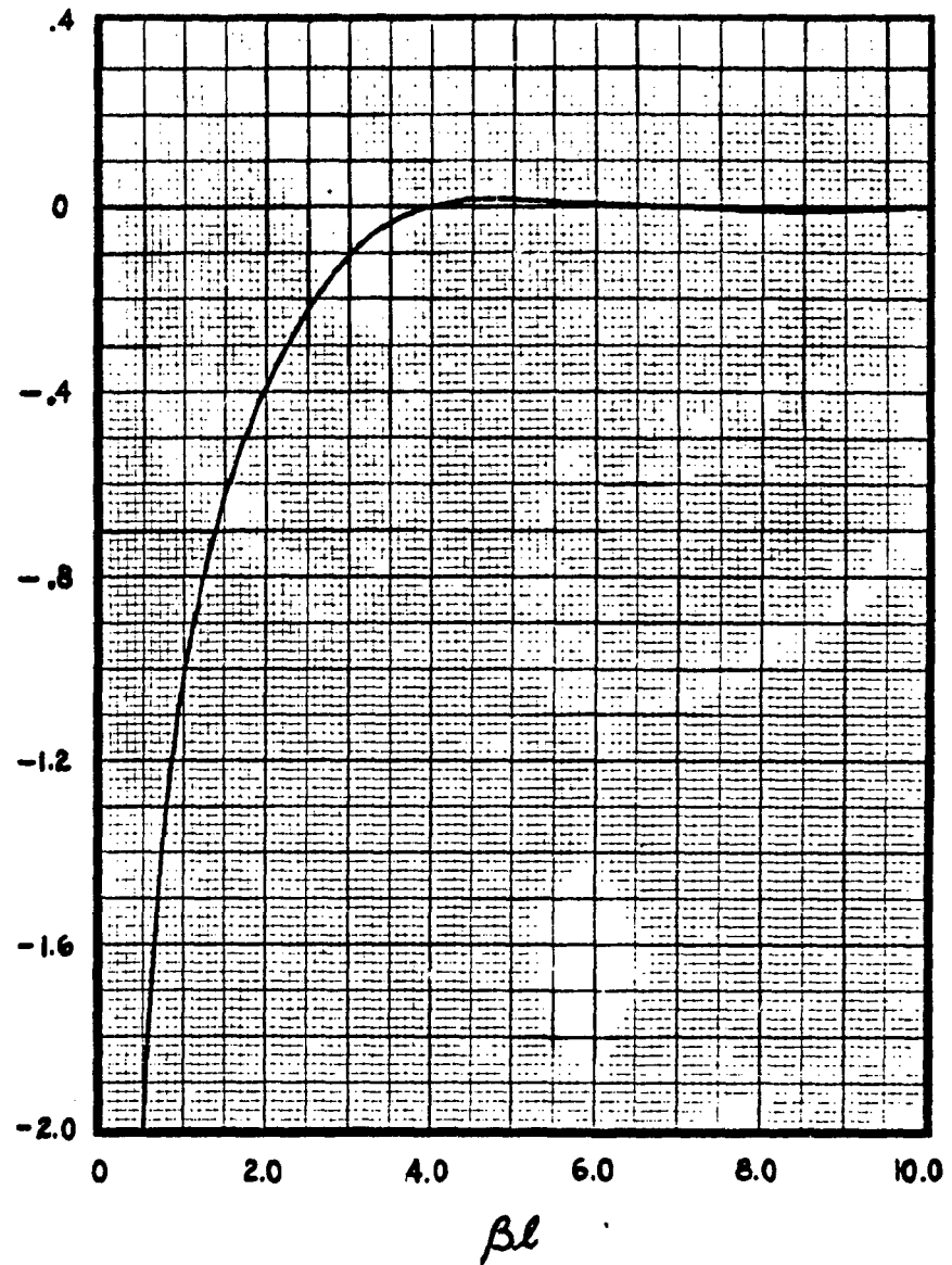
Fig. 5.22 Variation of \Omega_{18} with \beta l
