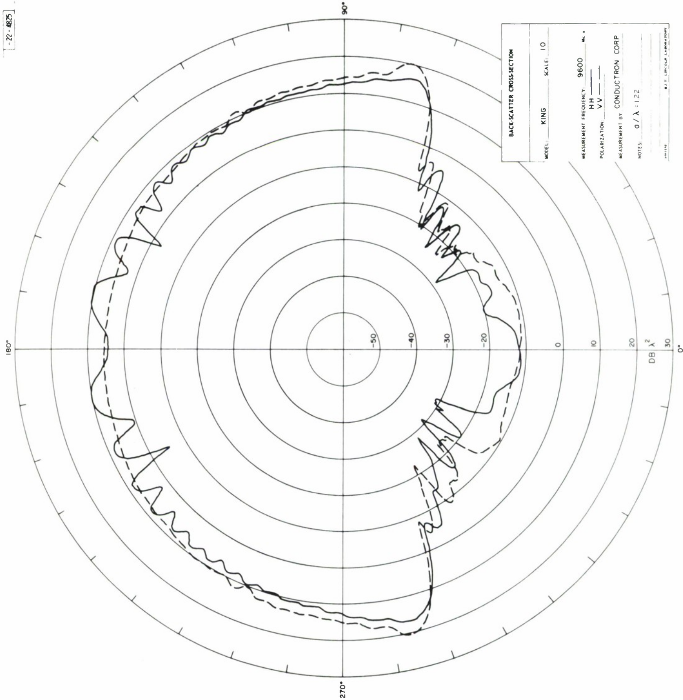
Figure 18: Backscattering Pattern, Model KING, a/\lambda = 1.22 (Cont.)
