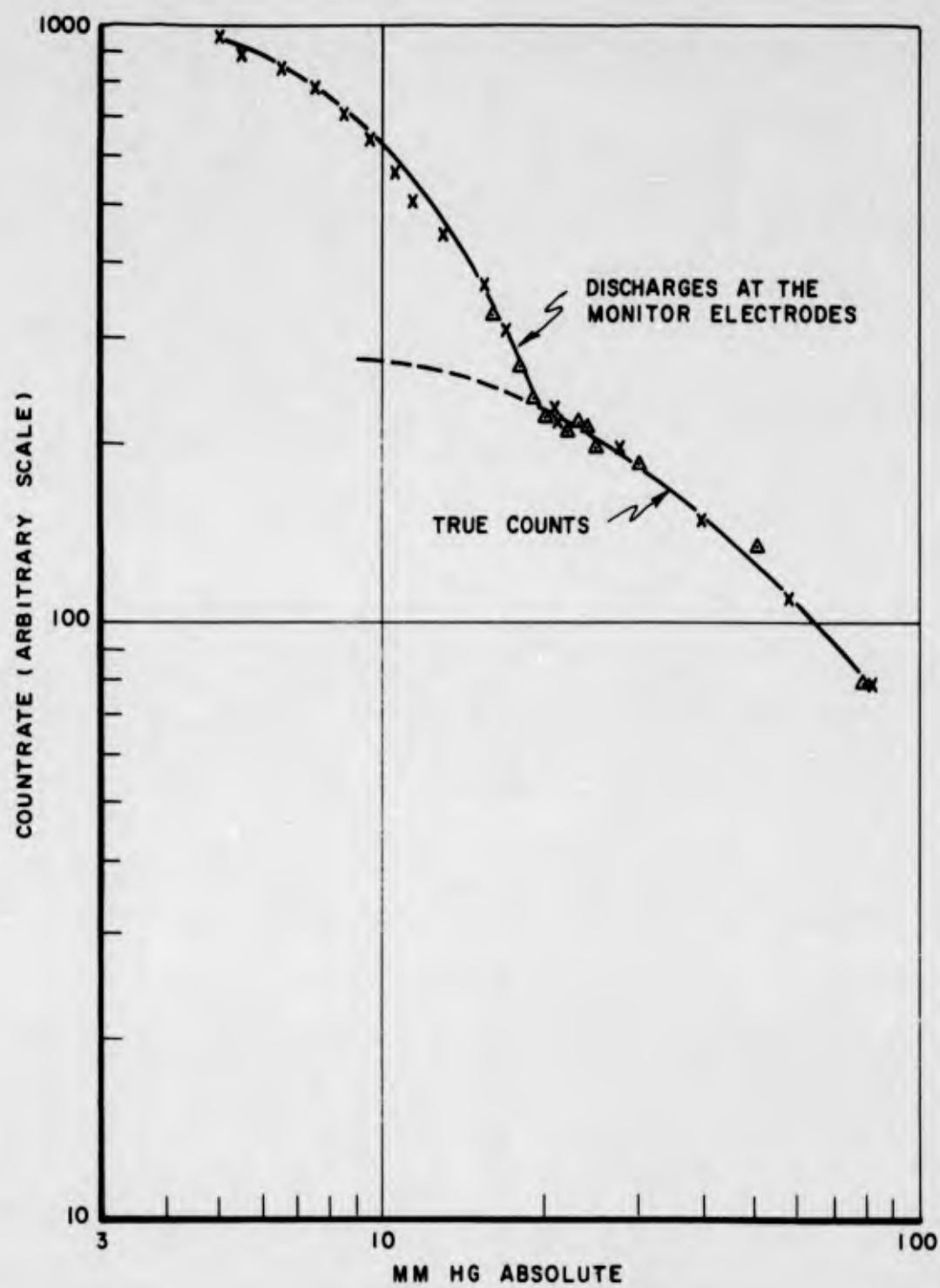
Figure 6.7 Count rate measured by monitor as a function of air pressure 2.725 meters from magnet.
