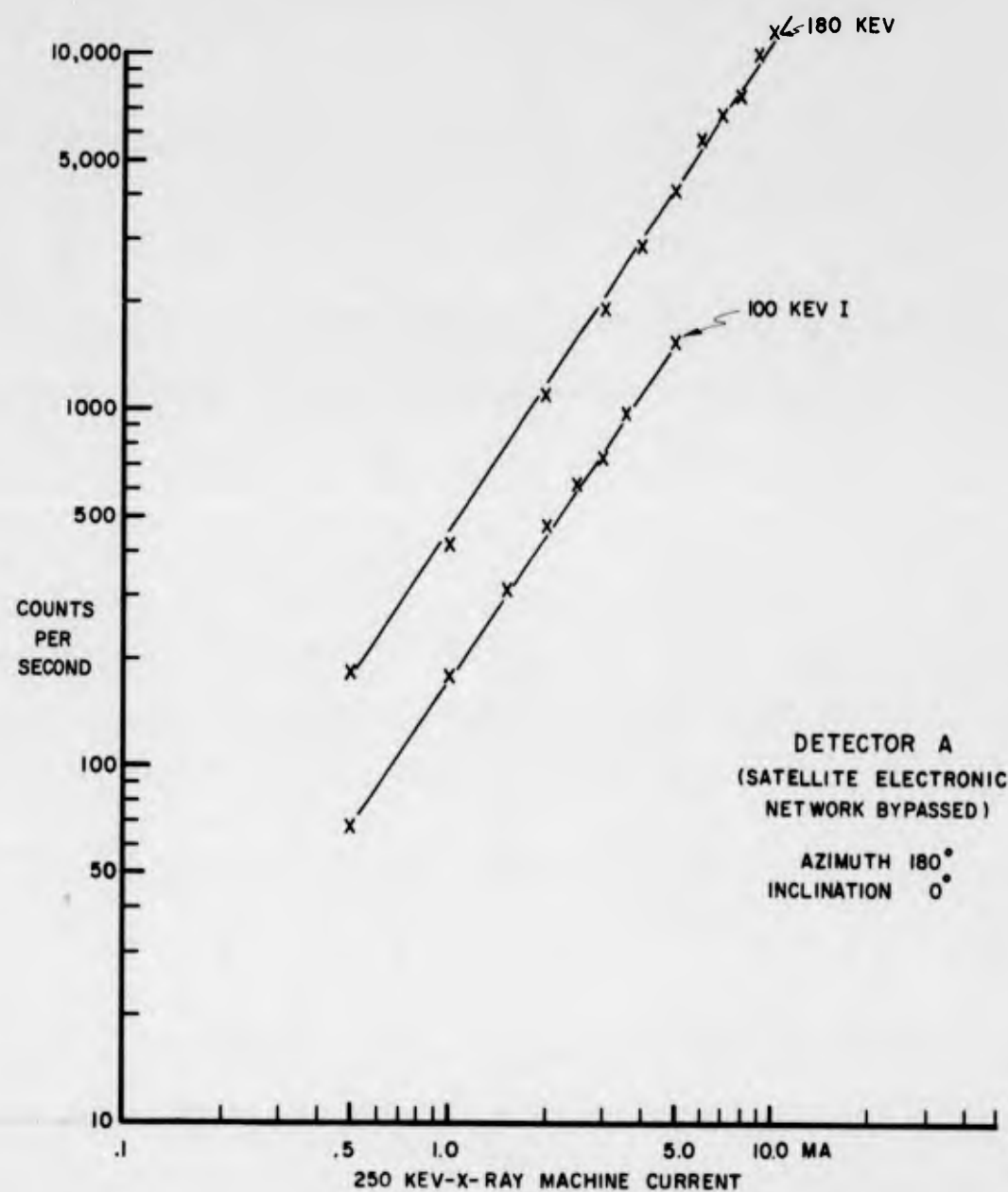
Figure 5.3 Response of Detector A to current variation.
