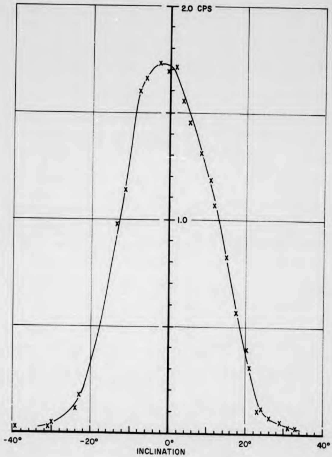
Figure 6.17 Detector A window characteristics, 180° azimuth, 2.685 meters, 2.4 amperes, 20 Oct 61.
