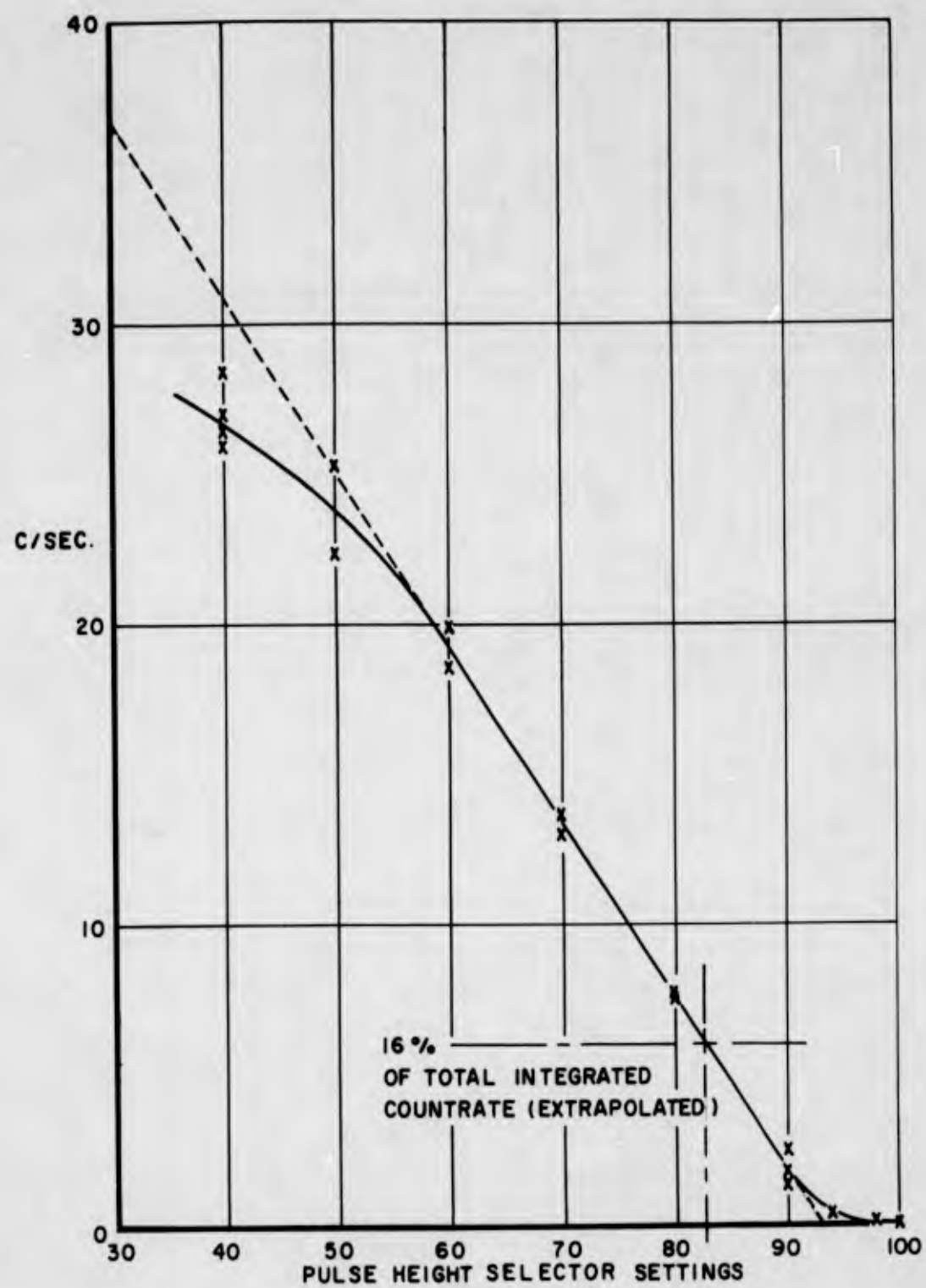
Figure 1.3 Integrated Tl^{204} spectrum for Discriminator A adjustment.
