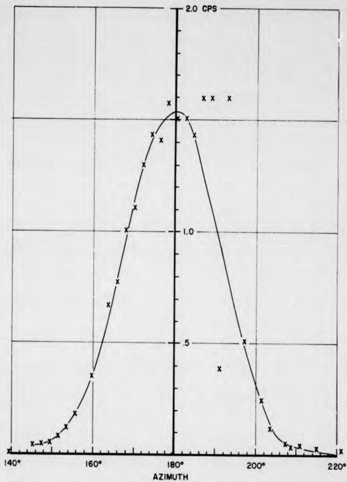
Figure 6.16 Detector A window characteristics, 0° inclination, 2.685 meters, 2.4 amperes, 24 Oct 61.
