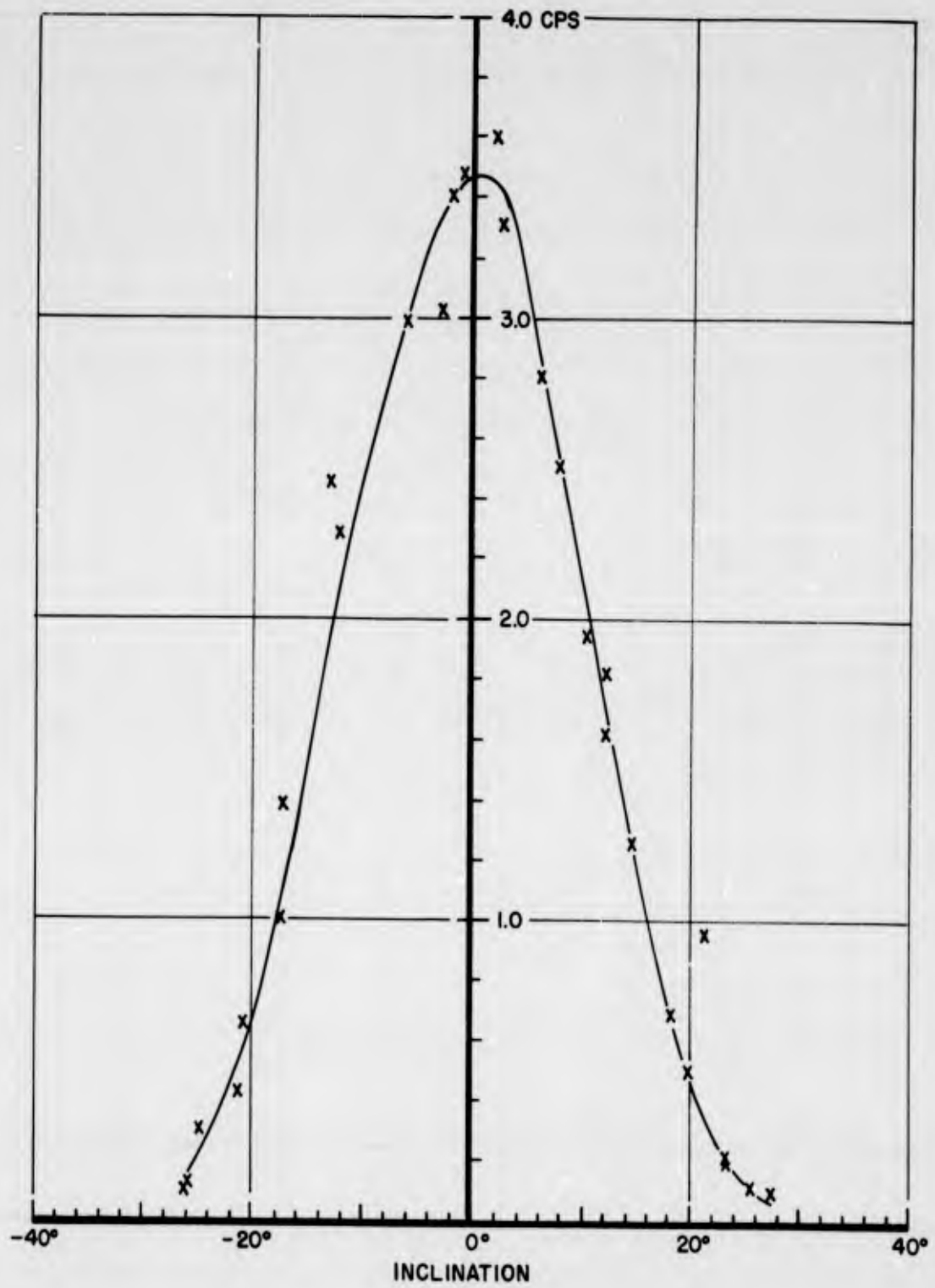
Figure 6.15 Detector A window characteristics with discriminator effective, 180° azimuth, 2.685 meters, 1.8 amperes, 25 Oct 61.
