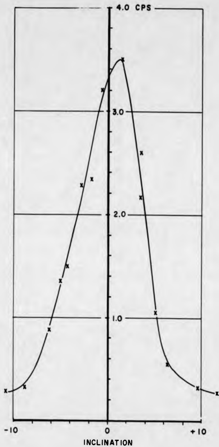
Figure 6.9 Electron scatter characteristics, Detector A with directional collimator, 180° azimuth, 2.685 meters, 1.6 amperes, 31 Oct 61.
