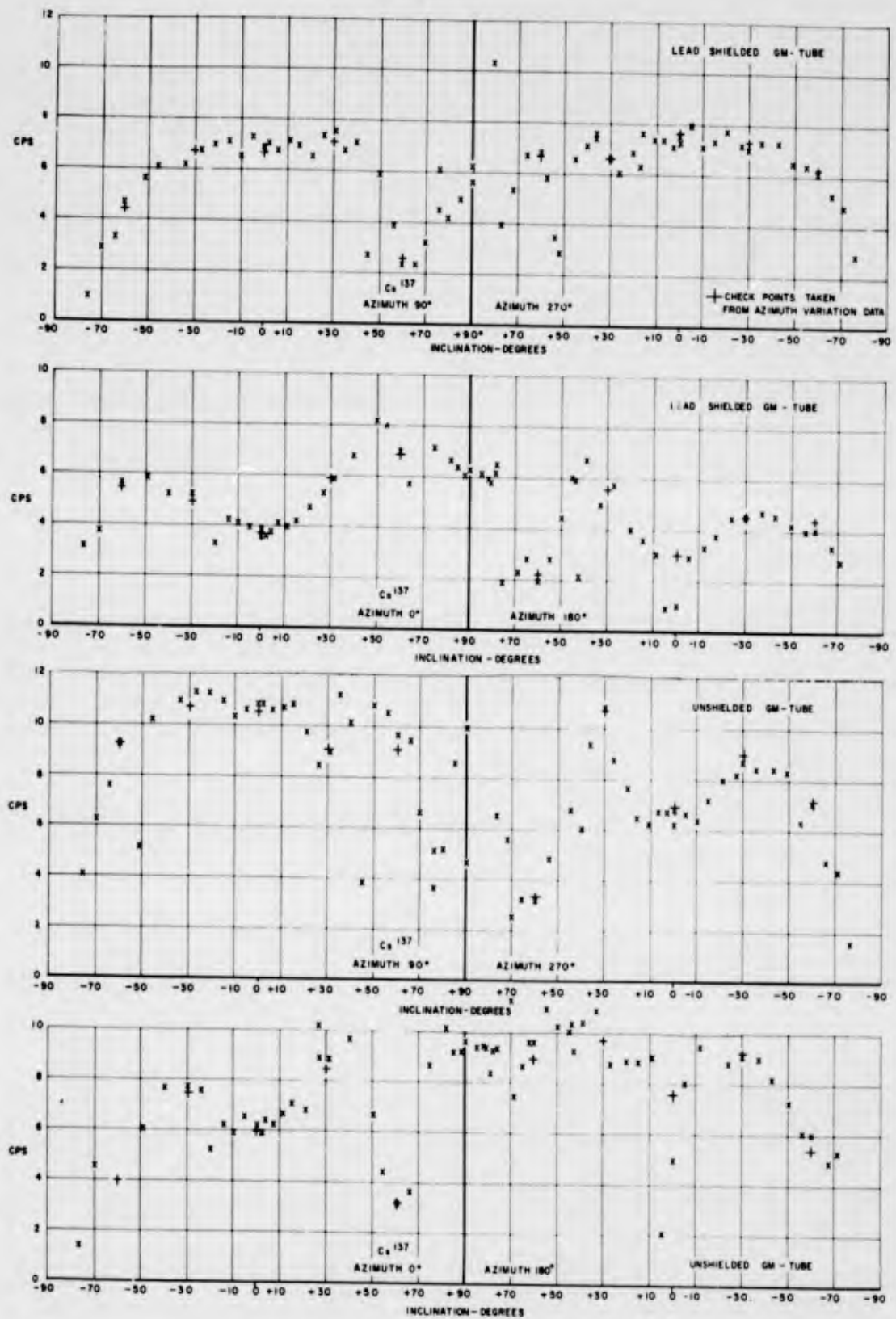
Figure 4.6 Response, Detectors C and D, 0.66-Mev gammas.
