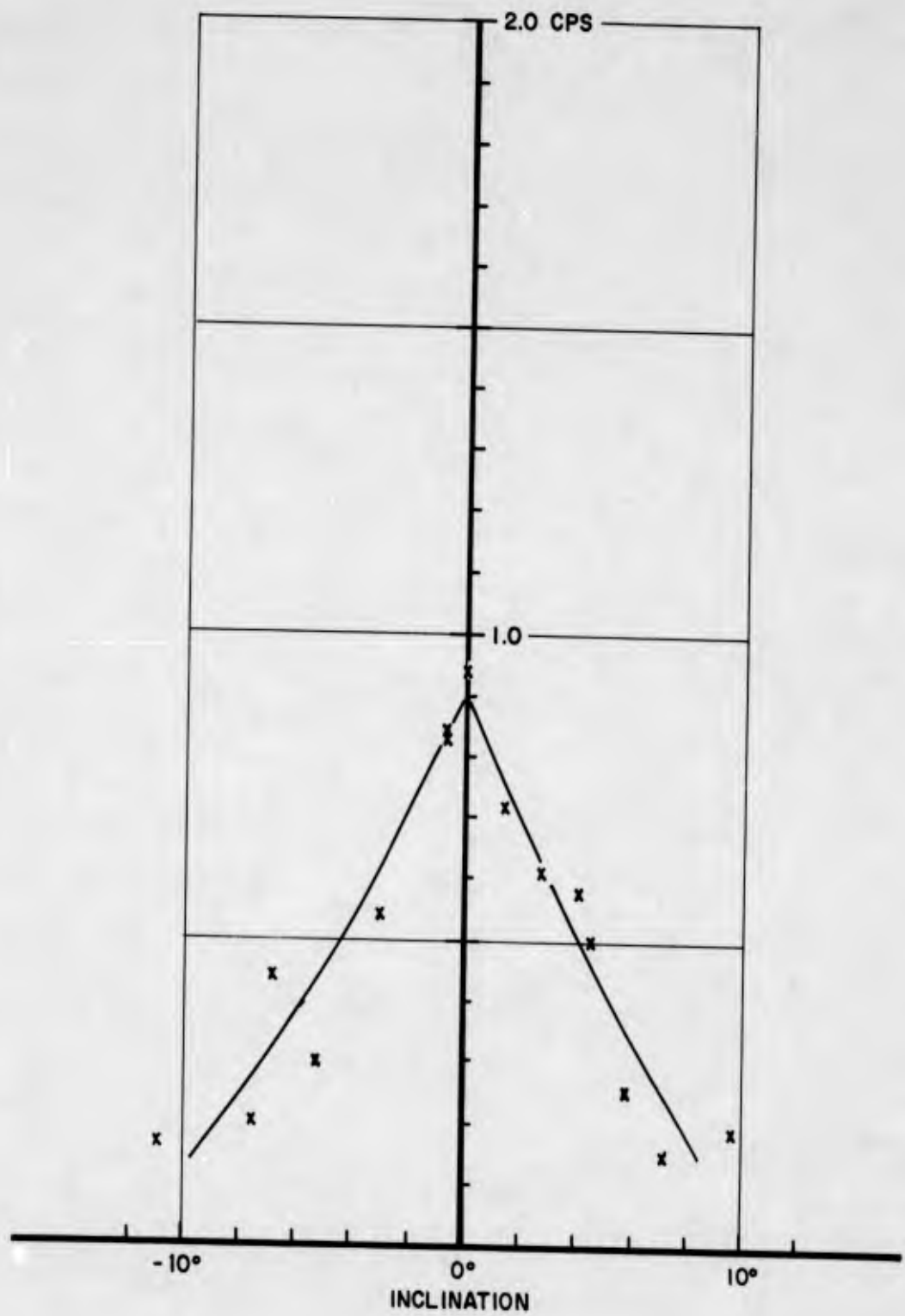
Figure 6.10 Electron scatter characteristics, Detector A with directional collimator, 180° azimuth, 2.685 meters, 2.4 amperes, 31 Oct 61.
