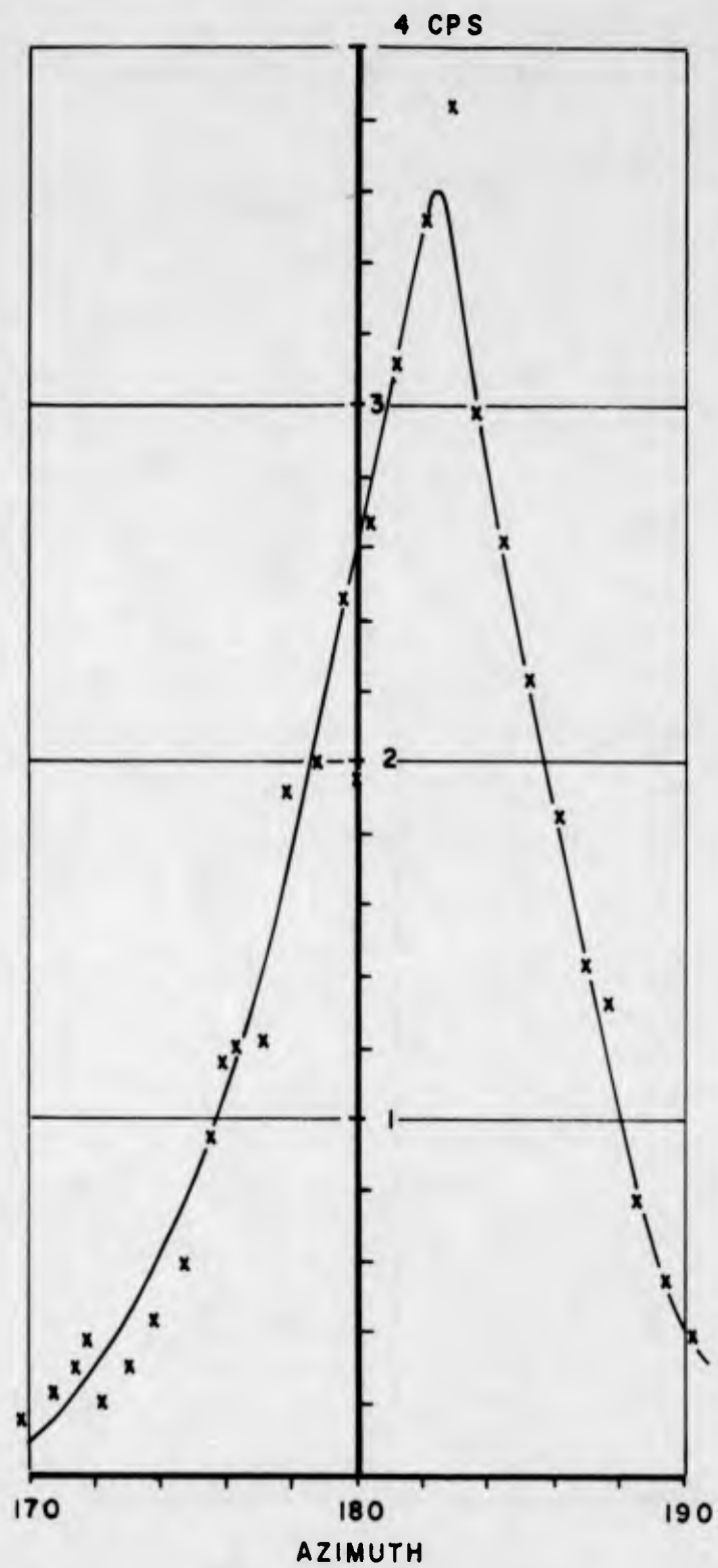
Figure 6.8 Electron scatter characteristics, Detector A with directional collimator, 0° inclination, 2.685 meters, 1.6 amperes, 30 Oct 61.
