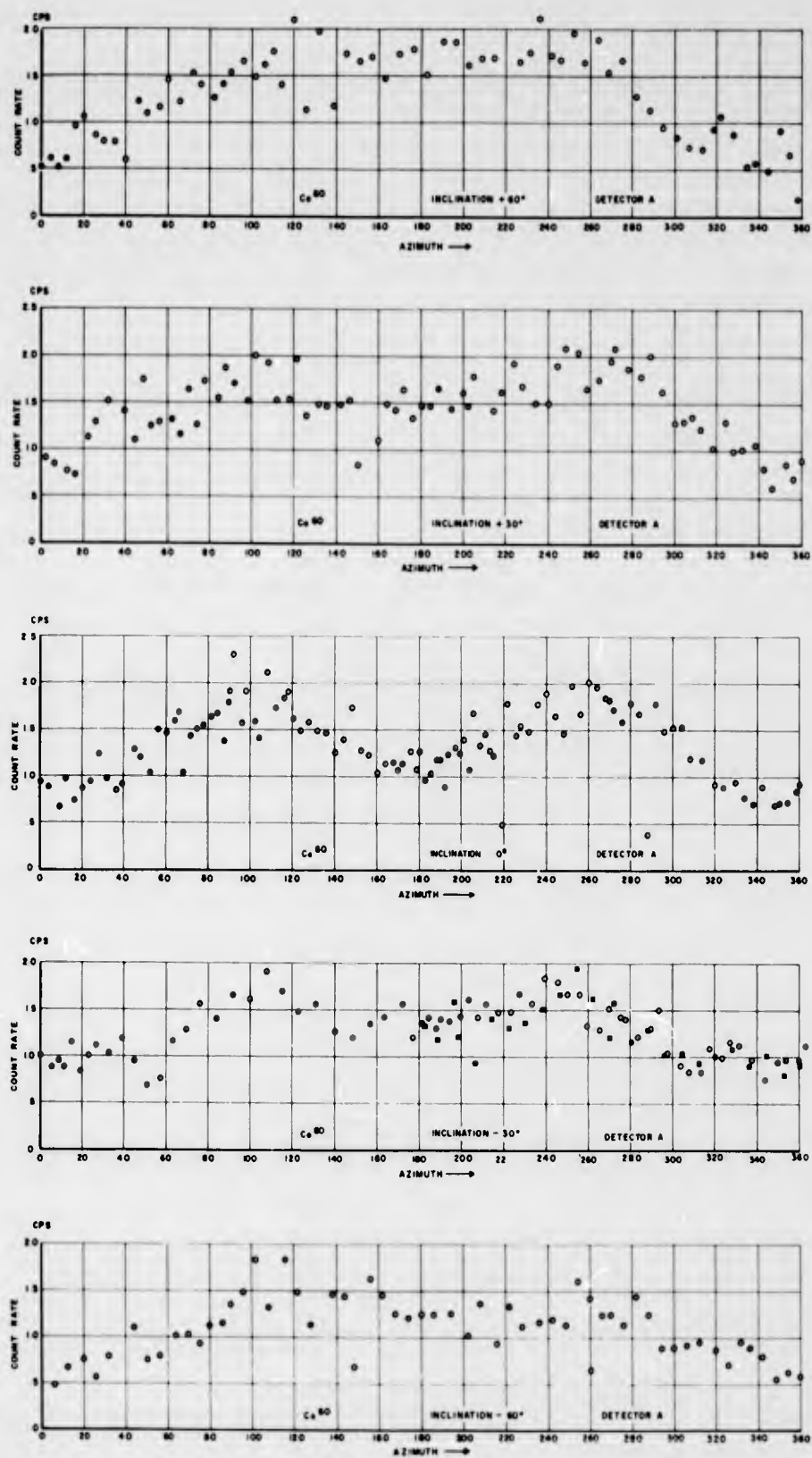
Figure 4.1 Response, Detector A, 1.17- and 1.33-Mev gammas.
