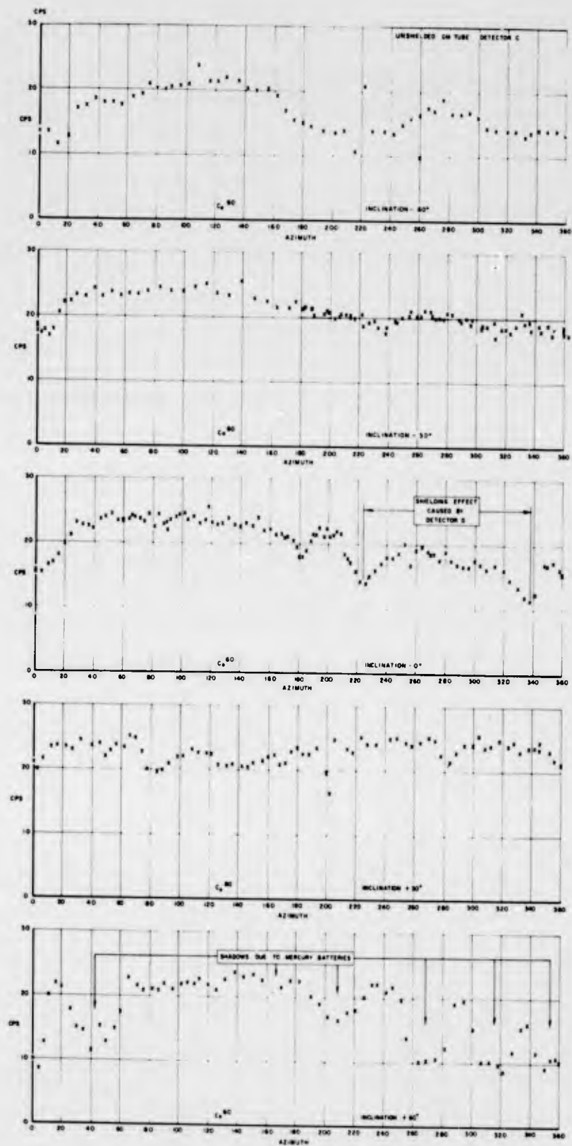
Figure 4.4 Response, Detector C, 1.17- and 1.33-Mev gammas.
