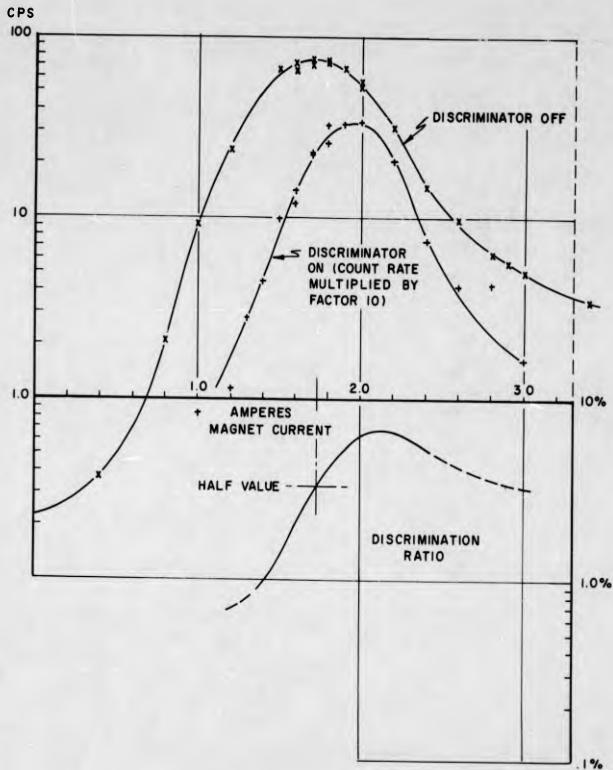
Figure 6.20 Response of Detector A to analyzed Y^{91} spectrum, 2.685 meters.
