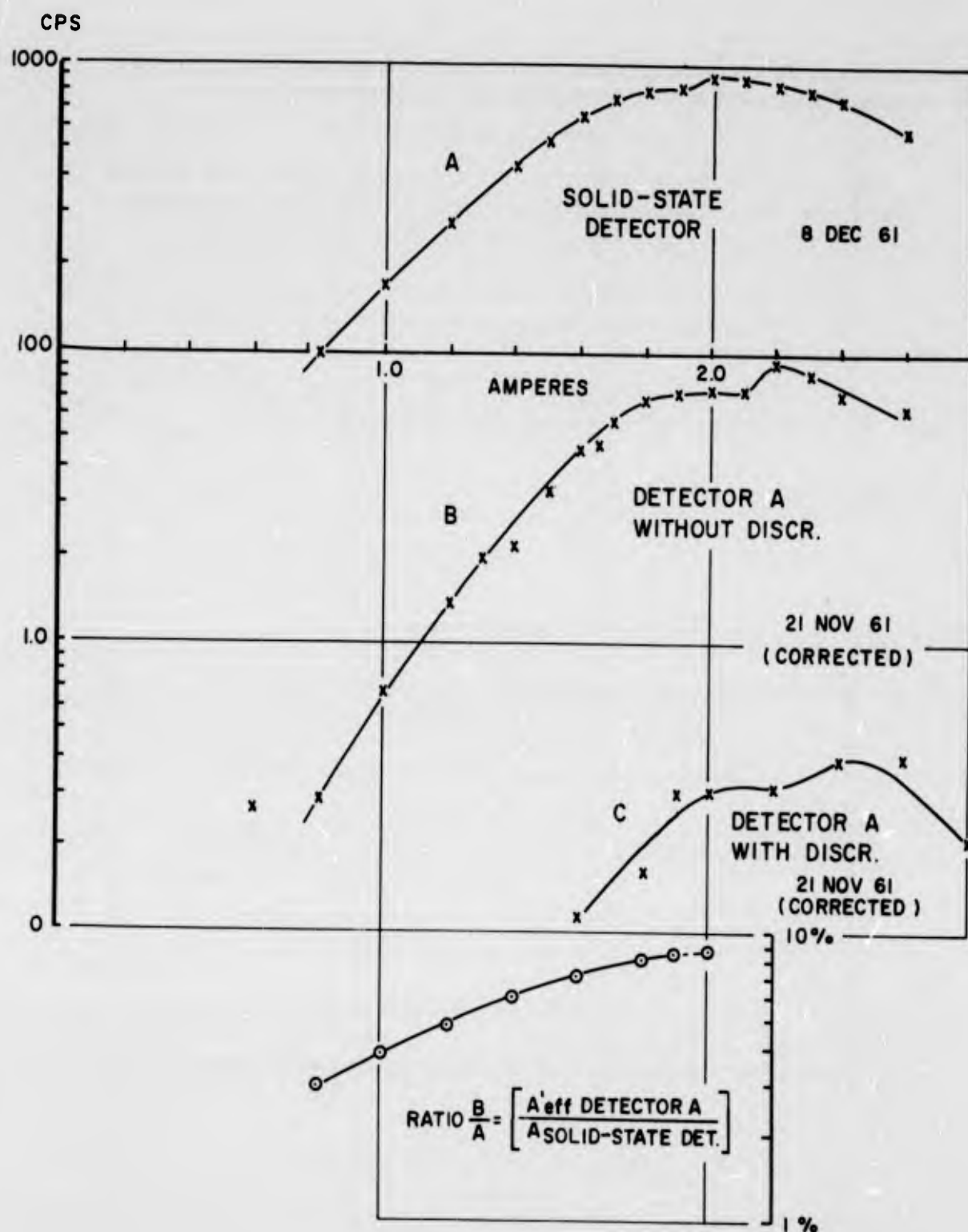
Figure 7.1 Determination of effective area of Detector A by comparison with the count rate of a highly sufficient solid-state detector with defined area.
