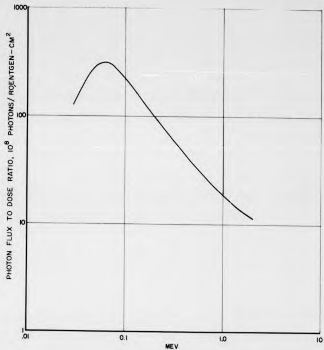
Figure 5.2 Photon flux per dose as a function of energy.
