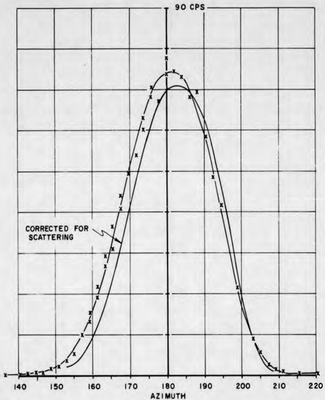
Figure 6.11 Detector A window characteristics corrected for scattering, 0° inclination, 2.685 meters, 1.6 amperes, 23 Oct 61.
