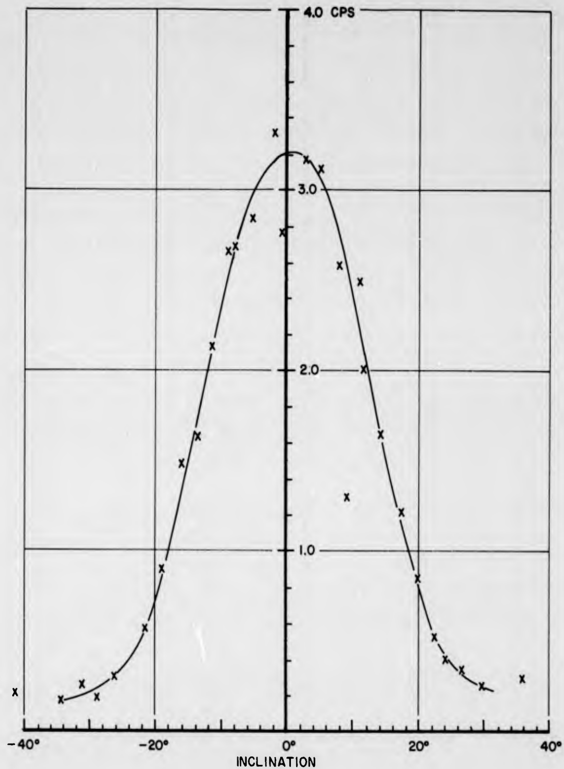
Figure 6.14 Detector A window characteristics, 180° azimuth, 2.685 meters, 0.8 ampere, 20 Oct 61.
