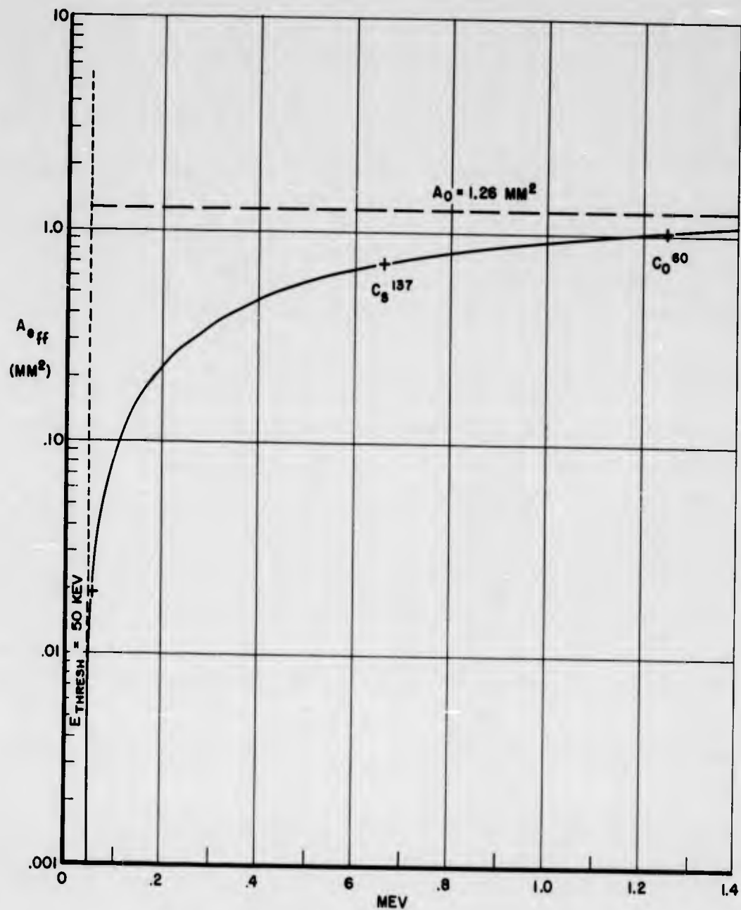
Figure 7.3 Effective area of Detector C (unshielded GM tube) as a function of photon energy.
