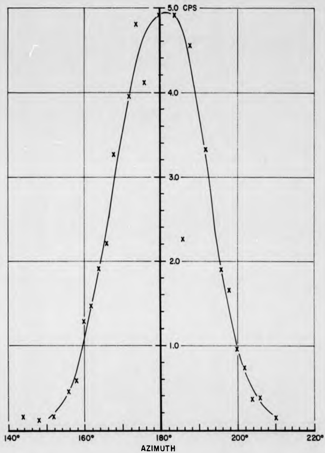
Figure 6.5 Detector A window characteristics, 0° inclination, 4.335 meters, 1.6 amperes, 25 Oct 61.
