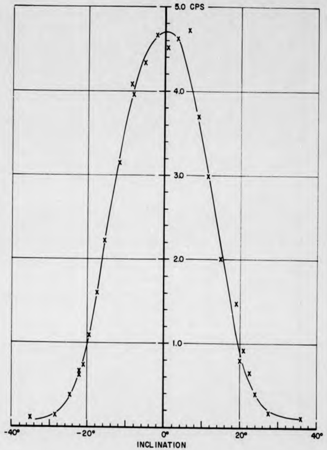
Figure 6.6 Detector A window characteristics, 180° azimuth, 4.335 meters, 1.6 amperes, 25 Oct 61.
