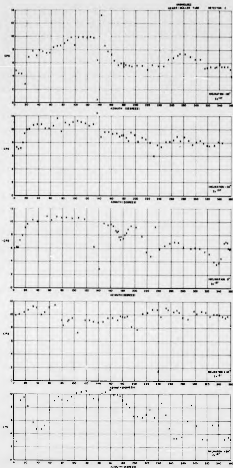
Figure 4.2 Response, Detector C, 0.66-Mev gammas.
