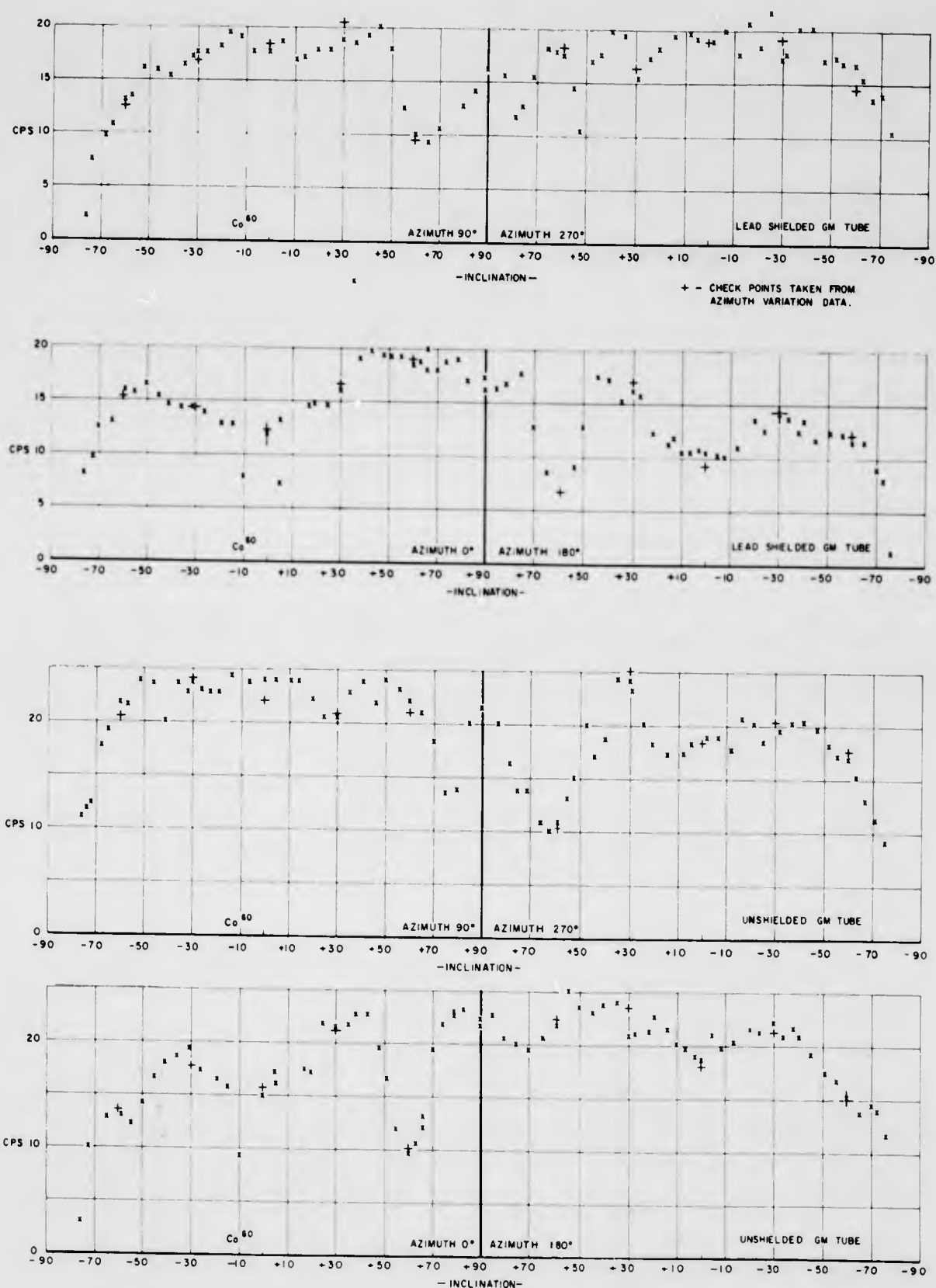
Figure 4.7 Response, Detectors C and D, 1.17- and 1.33 Mev gammas.
