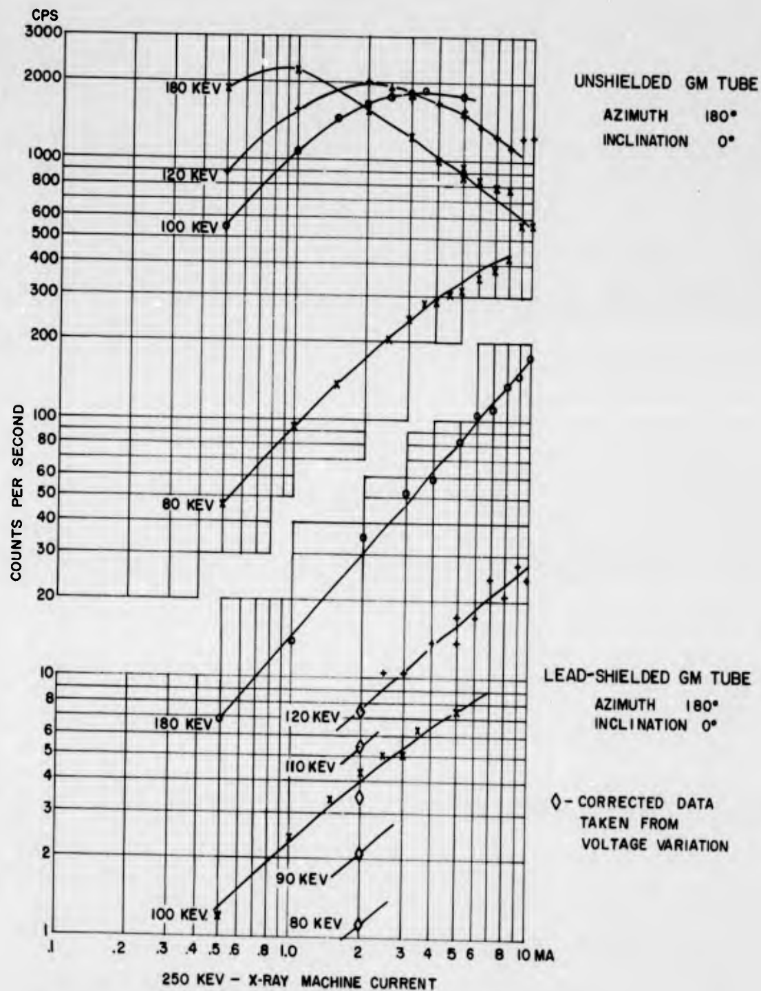
Figure 3.2 GM tube response curves.
