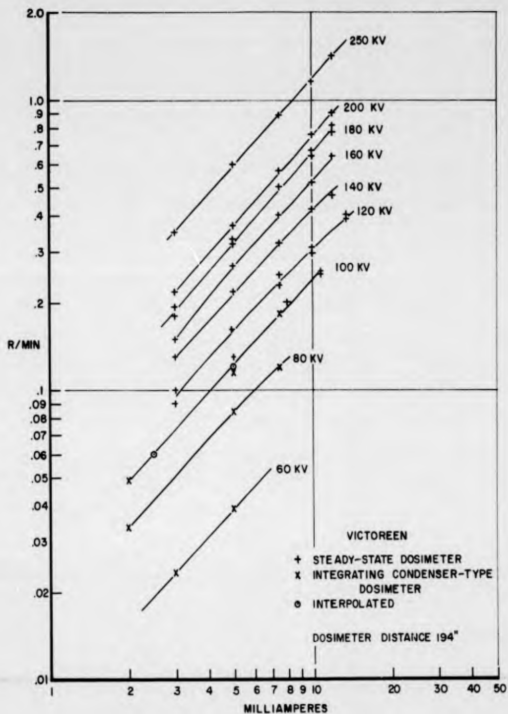
Figure 5.7 Dosimetric calibration of X-ray machine, 27 Nov 61.
