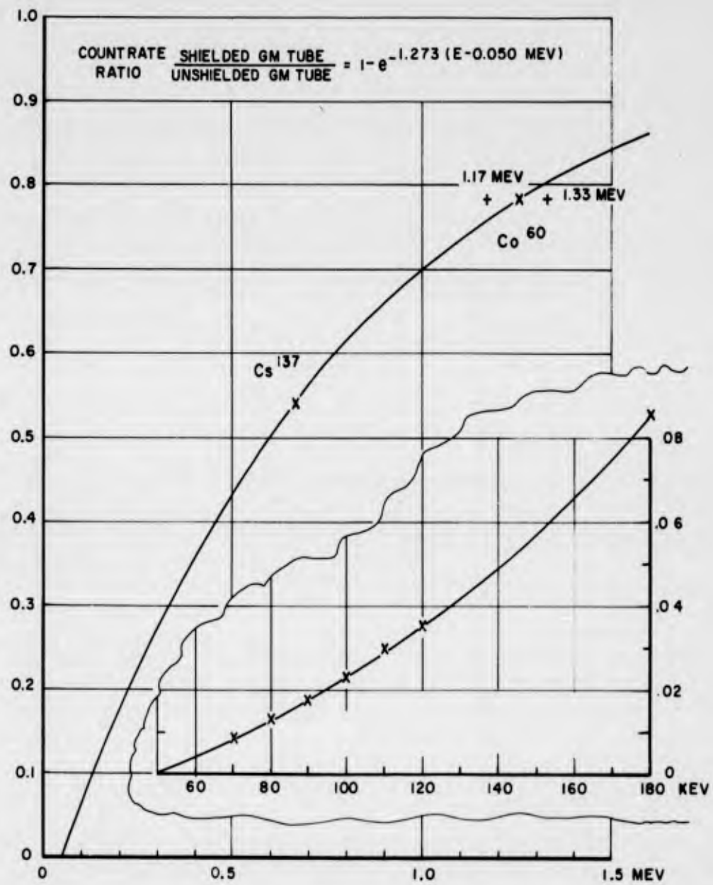
Figure 5.9 Count-rate ratio.
