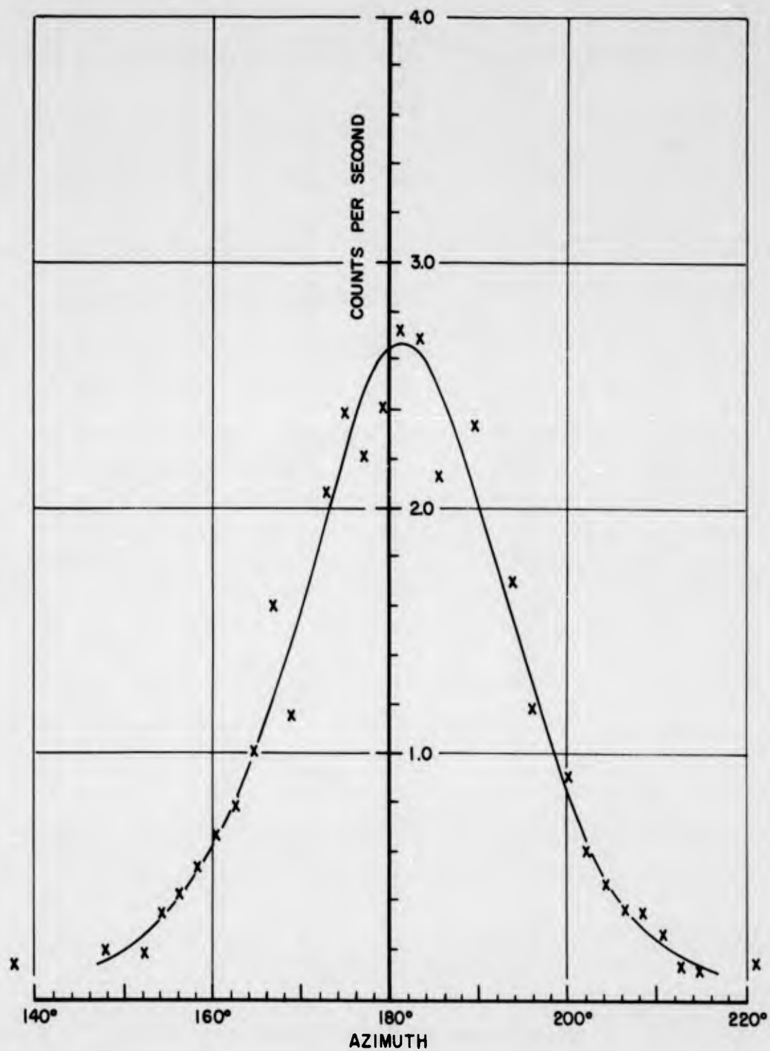
Figure 6.13 Detector A window characteristics, 0° inclination, 2.685 meters, 0.8 ampere, 23 Oct 61.
