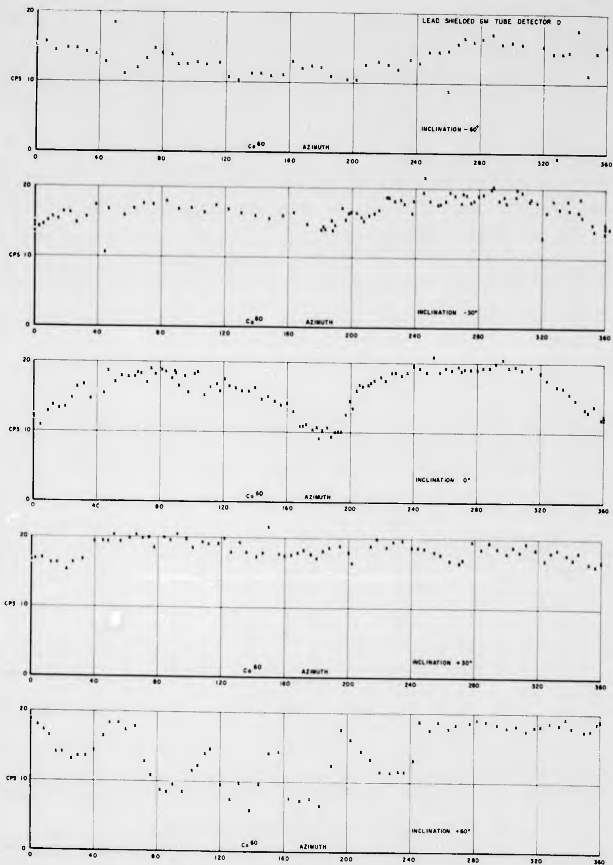
Figure 4.5 Response, Detector D, 1.17- and 1.33-Mev gammas.
