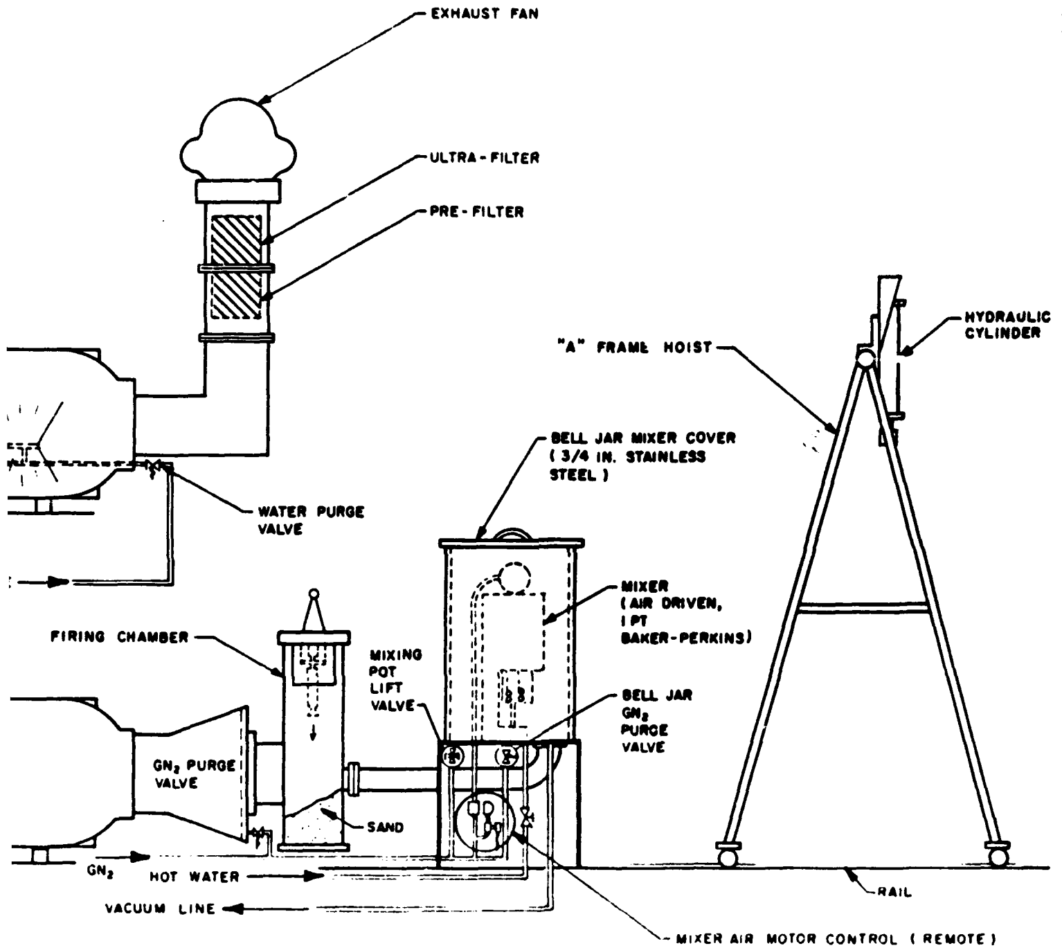
Figure 4. Toxic Propellant Mixing and Motor Firing Facility
