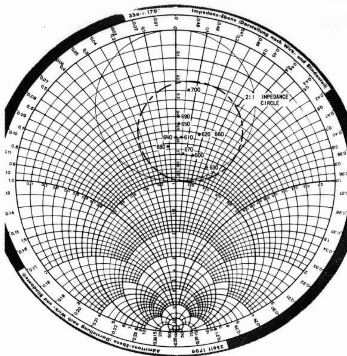
Figure 9. Impedance of a Log Periodic Dipole Array with Parasitic Elements ( \tau = 0.898 , s/l = 0.113 ).
