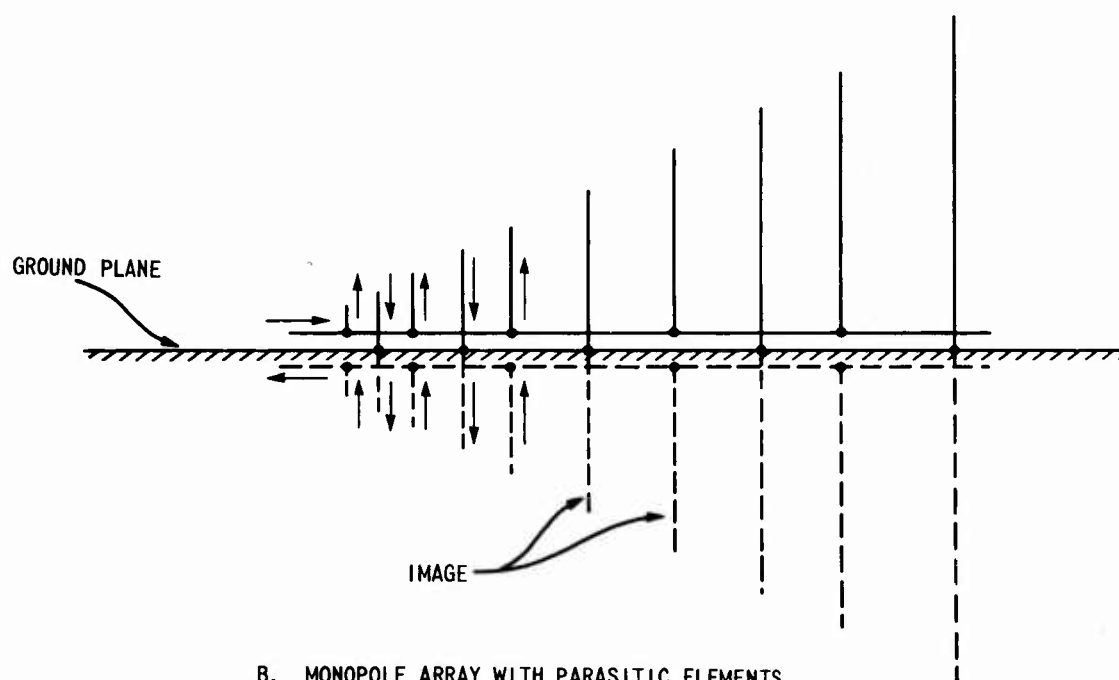
B. MONOPOLE ARRAY WITH PARASITIC ELEMENTS.
