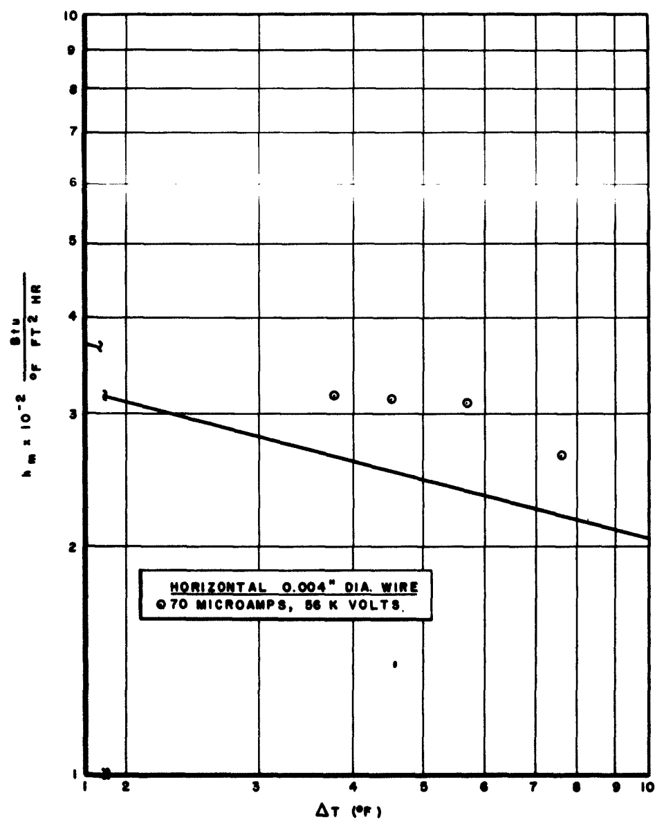
Figure 6. Effects of Corona Current with Wire 2 Inches from Plate
