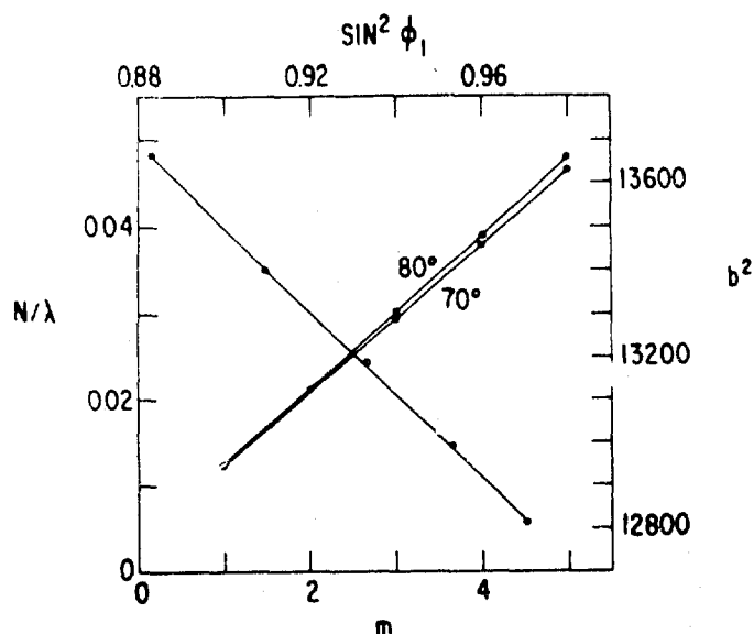
Figure 10. Experimental Data Illustrating Higher-Order \frac{1}{2} Fringe Method of Determining Film Thickness Per Monolayer and Refractive Index. BaCuH multilayers on chromium plated glass. Open circles: N/\lambda as function of fringe order, m [text Equation (5)] for angles of incidence 70 and 80 degrees. Closed circles: b^2(\sin^2 \phi) [text Equation (6)] for angles of incidence 70.0, 72.5, 75.0, 77.5, and 80.0 degrees. (Reproduced from the Journal of Colloid Science 8 by kind permission of Academic Press, Inc.)
