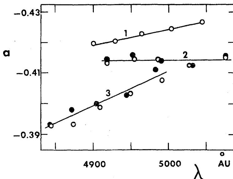
Figure 11. Apparent \frac{1}{2} Vibration Phase Change at Surface of "Clean" Chromium Reflector, Obtained by Extrapolation of Straight Line Relating Fringe Order, m , to N/\lambda [Equation (5)]. Abscissa: Average fringe wavelength for first- to fifth-order fringes. Ordinate: a , equal to -0.5(1 - \theta/\pi) , where \theta is phase change at "clean" surface. If \theta = 0 , a = -0.5 . Curve 1: For BaCuH stearate slide III; 2: BaCuH stearate checkerboard slide V; 3: BaCuH nonadecanoate slide II. See Table II.
