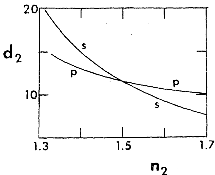
Figure 15. Plot of d_2 Versus n_2 for \frac{1}{4} Added Double Layer of Barium Stearate. Letters s and p indicate curves obtained from s fringe and p fringe equations. Each curve represents the solutions d_2(n_2) that are compatible with a constant fringe shift, 52.5 ÅU for the s step and 26.25 ÅU for the p step. (Adapted from Mattuck, Figure 2. 4 Permission to reproduce the diagram was kindly granted by the Editors of the Journal of the Optical Society of America.)
