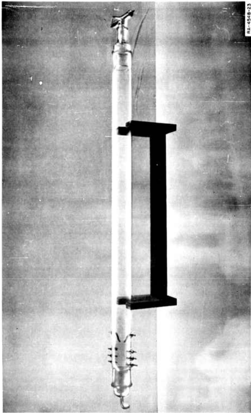
FIG. 22 ONE-METER PLASMA-SWITCH TUBE
