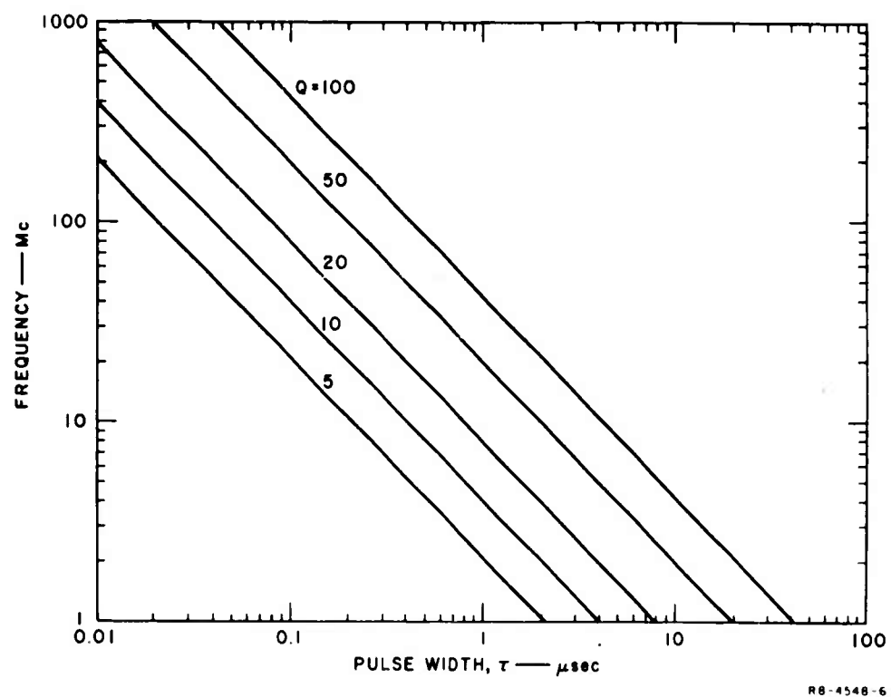
FIG. 6 RING TRANSMITTER: PULSE WIDTHS TO 10-PERCENT POWER LEVEL
