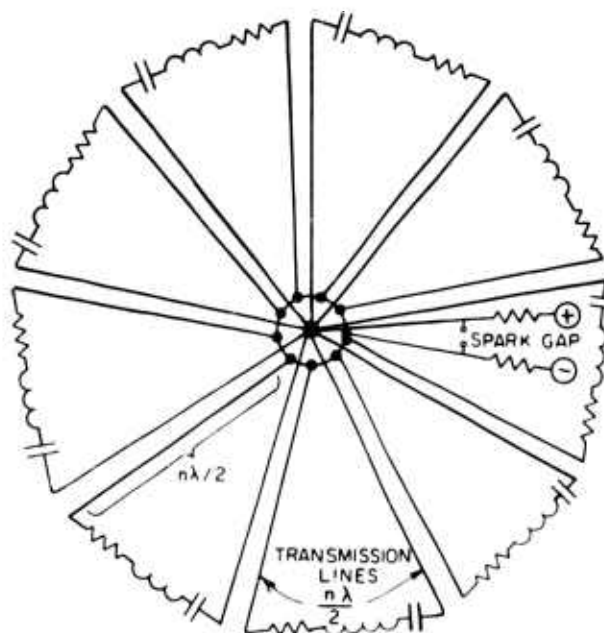
FIG. 9 IMPROVED RING TRANSMITTER
