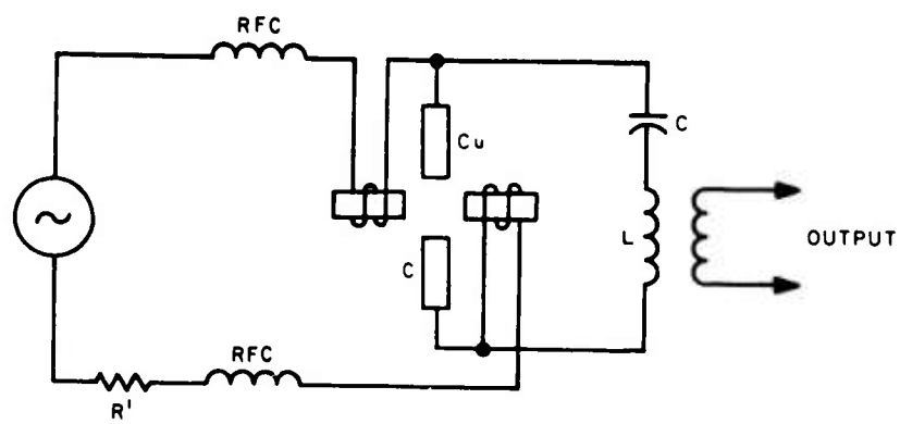
FIG. 35 POULSEN ARC TRANSMITTER
