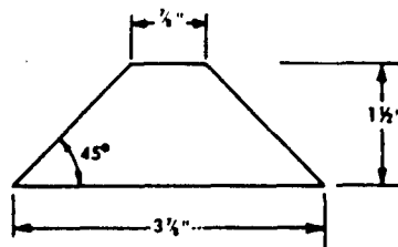
Cross Sections
