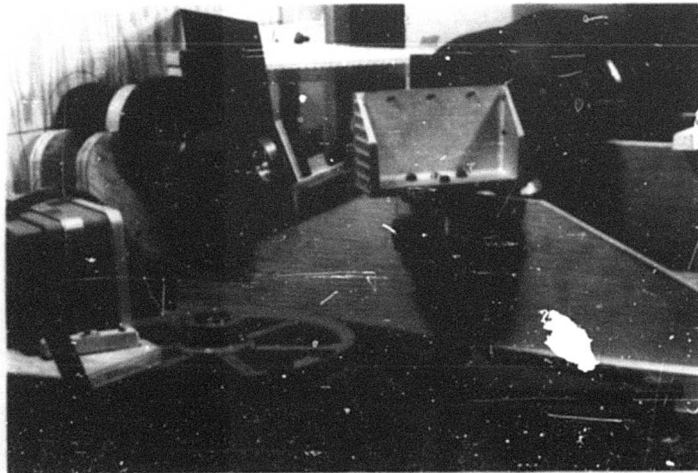
Fig. 6. Lens and beamsplitter for triggering flash in phase with mirror rotation
