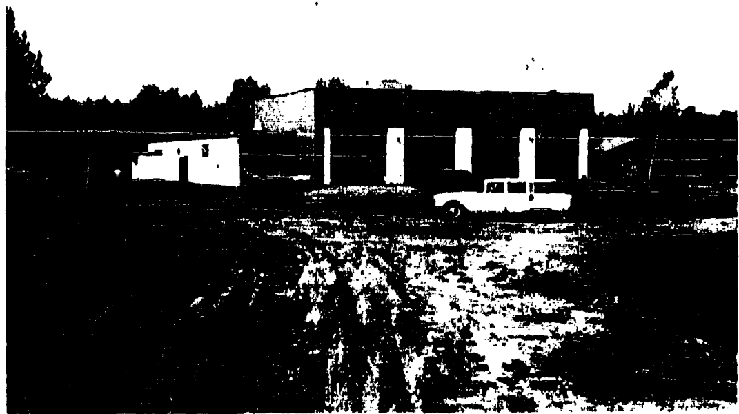
Fig. 17 Avco-Everett Research Laboratory's facility for the development of MHD generators. The facility is located on a 58 acre tract on the Merrimac River near Haverhill, Mass., and was completed last September. It is valued at one half million dollars. The Mark V, 20 megawatt MHD generator is under construction for the Advanced Research Projects Agency in the taller part of the structure. It should be mentioned that the test cell is considerably over-size for a generator of the Mark V capacity. The remainder of the building houses auxiliary equipment such as water pumps, fuel pumps, magnet pre-exciter, control room, offices and shop.
