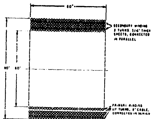
Fig. 8(b). Cross section of energy-storage transformer
