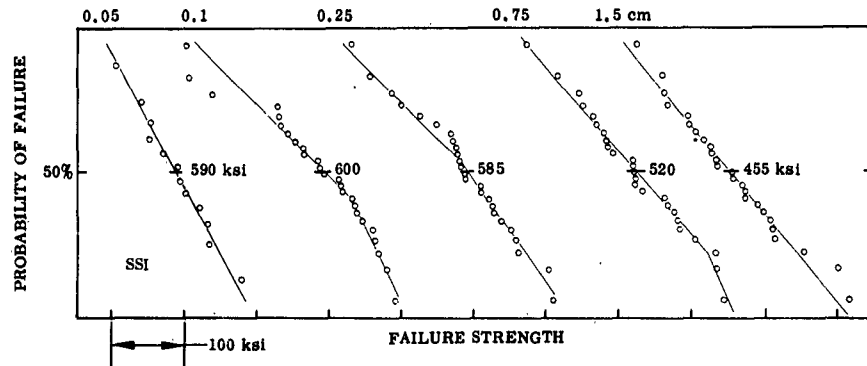
FIGURE 11. GAUSSIAN FAILURE DISTRIBUTIONS AT DIFFERENT GAGE LENGTHS
