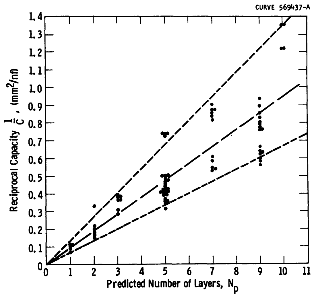
Fig. 1—Reciprocal capacity vs predicted number of layers
