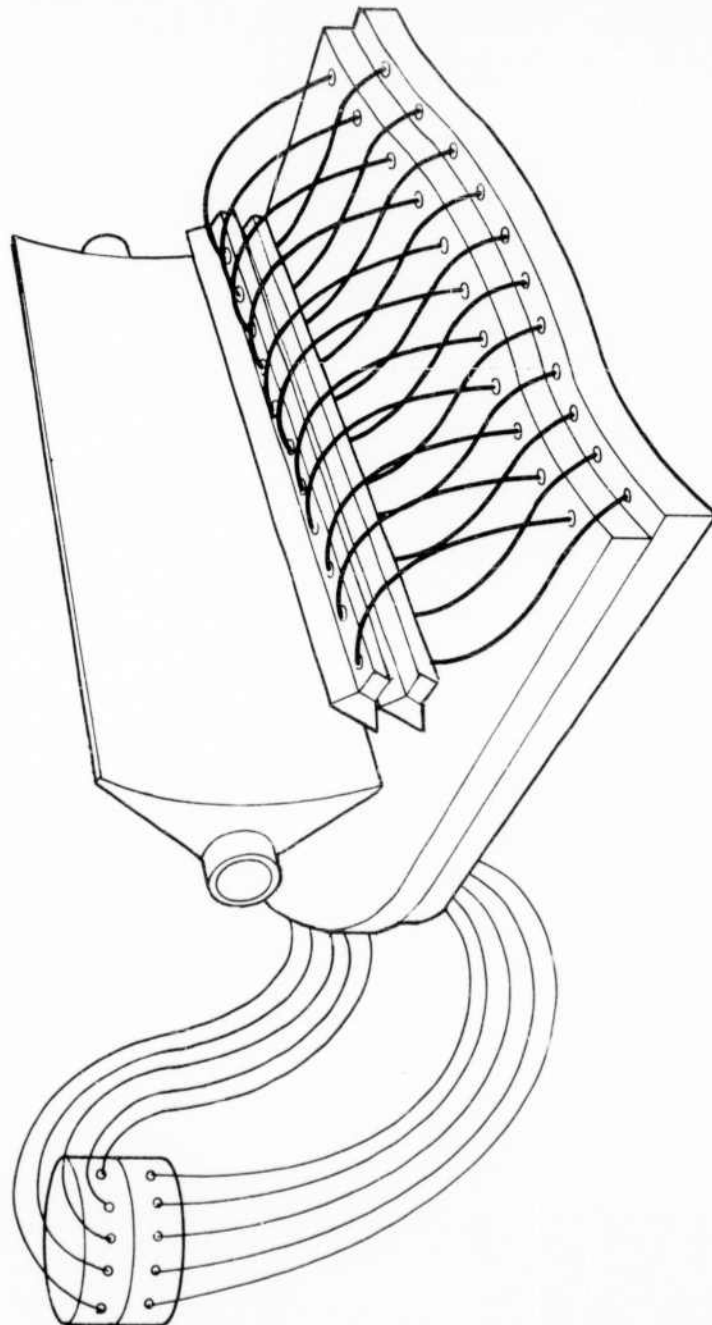
Figure 9-1. Possible Antenna Configuration for Amplitude Sensing Elevation Monopulse System
