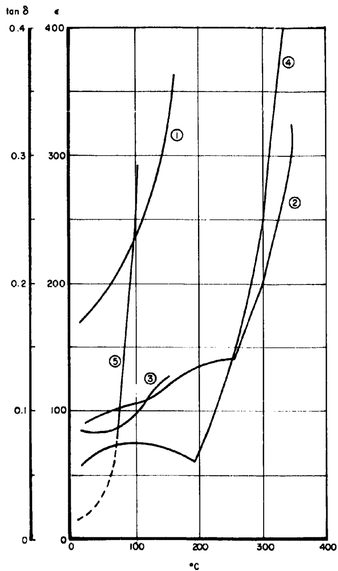
Figure 2. Dielectric Constant and Loss Tangent of Lead Titanate Single Crystals
