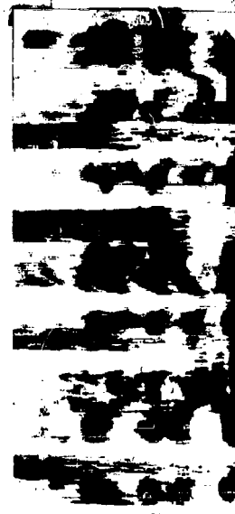
Spectrogram of Speaker 4
