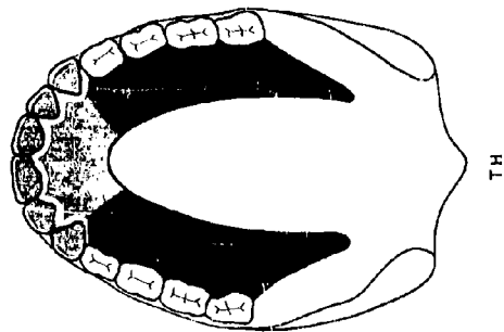
Figure 3. Diagram of a human mouth showing the tongue in a retracted position.
