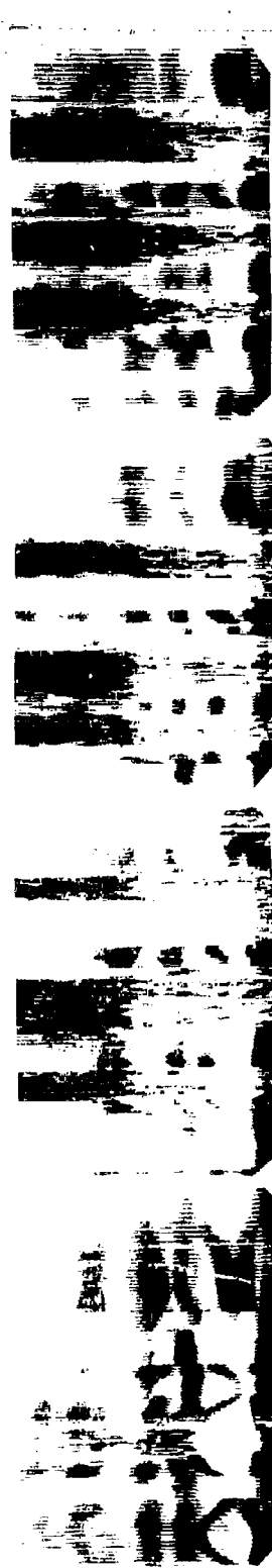
Speaker 2 Spectrogram of "... of Mike Shiplop..."
