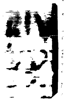
Spectrogram of "...ness soundness of rottenness..." by Speaker 2 Figure 60
