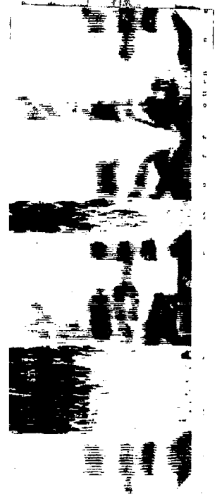
Spectrogram of "...ness soundness of rottenness..." by Speaker 2 Figure 56
