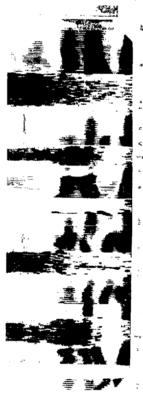
Spectrogram of "...ness soundness of rottenness..." by Speaker 2 Figure 56
