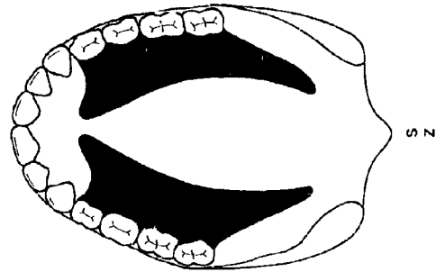
Figure 4. Diagram of a human mouth showing the tongue in a retracted position.
