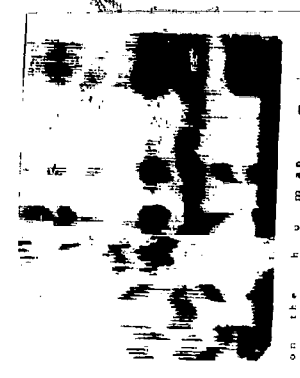
Spectrogram of "...ness soundness of rottenness..." by Speaker 2 Figure 61
