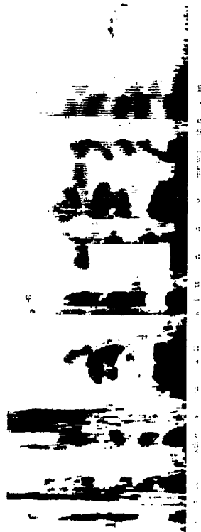
Spectrogram of the word "moon" with time axis.
