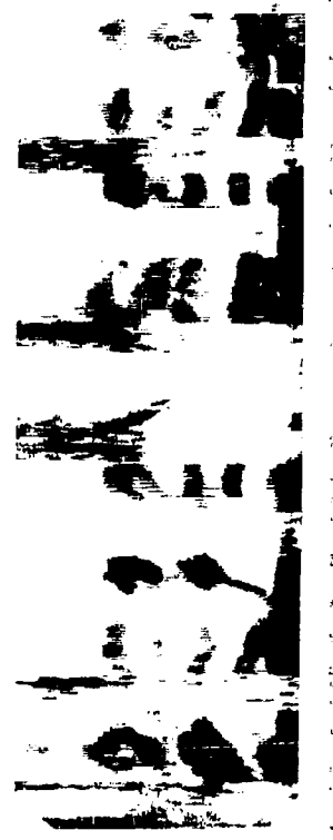
Spectrogram of "...on the human m..." by Speaker 2 Figure 57
