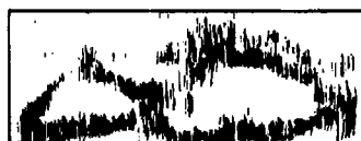
Southern Spectrogram of Southern, English, and General American Speech Figure 9
