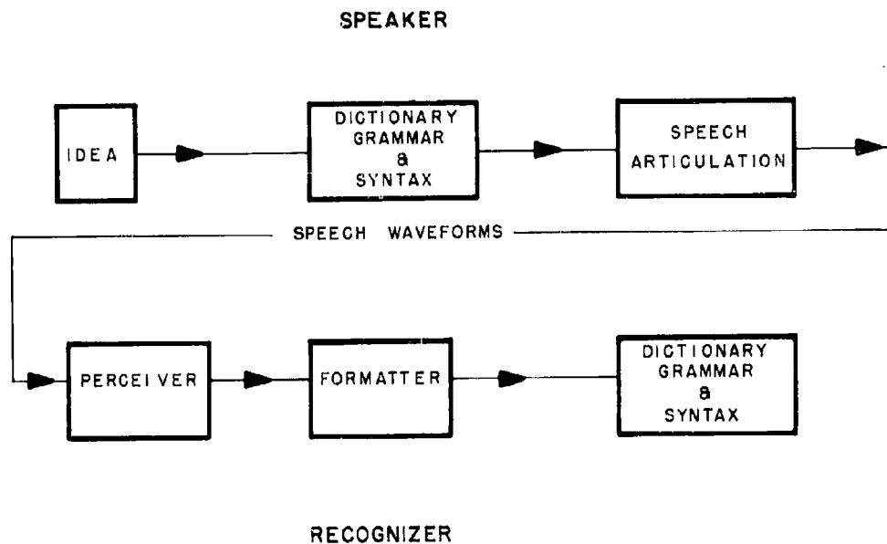
Diagram of Speech Production and Perception Process
