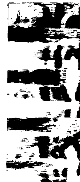
Spectrogram of Speaker 6
