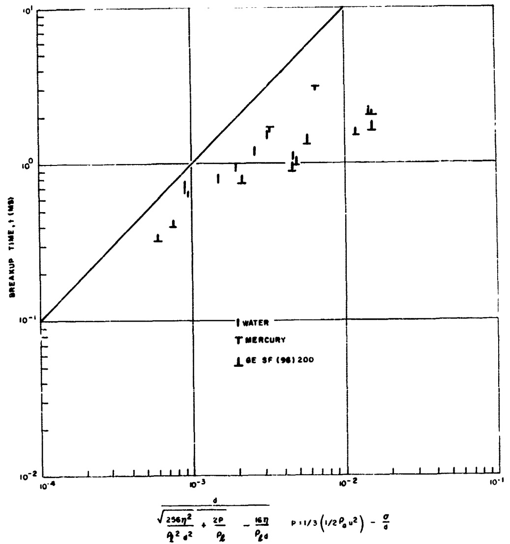
Figure 10. Comparison of Experimental Bag Breakup Times with Equation (5.10)
