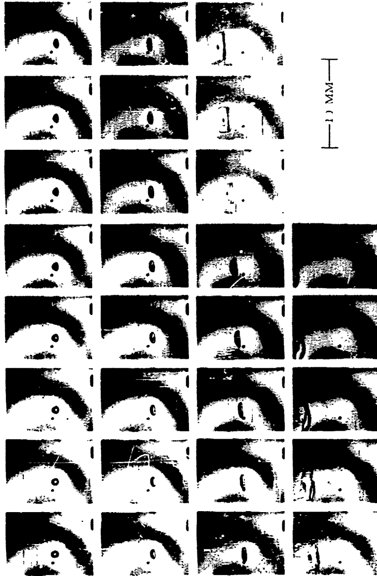
Test 234 Liquid-Water Relative Velocity 65 ft/sec Drop Size 0.7 MM Time per Frame 0.0766 msec
