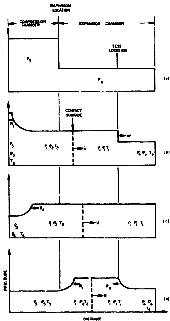
Figure A1. Shock Tube Pressure Diagrams.
