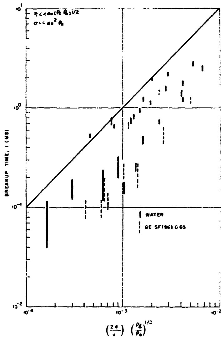
Figure 22. Comparison of Special Case of Gordon Theory with Experimental Breakup Times.
