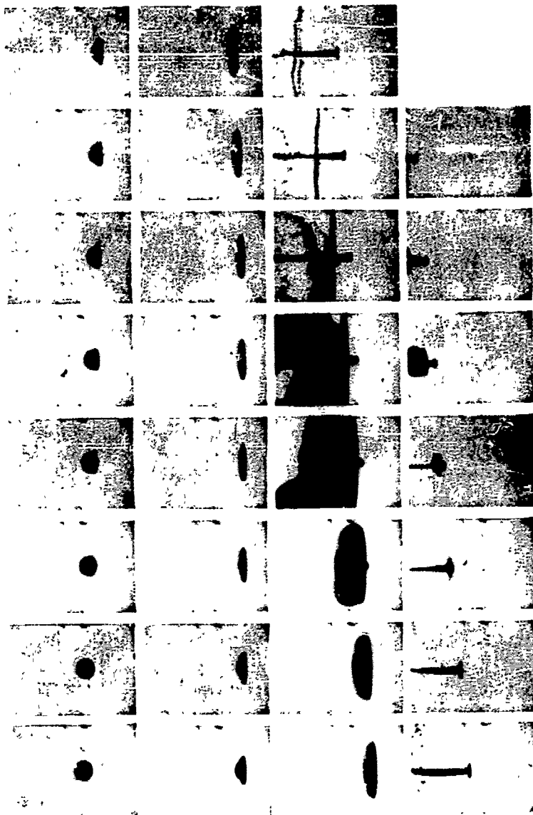
Test 164 Liquin Mercury Relative Velocity 173 ft/sec Drop Size 1.2 MM Time per Frame 0.1571 msec
