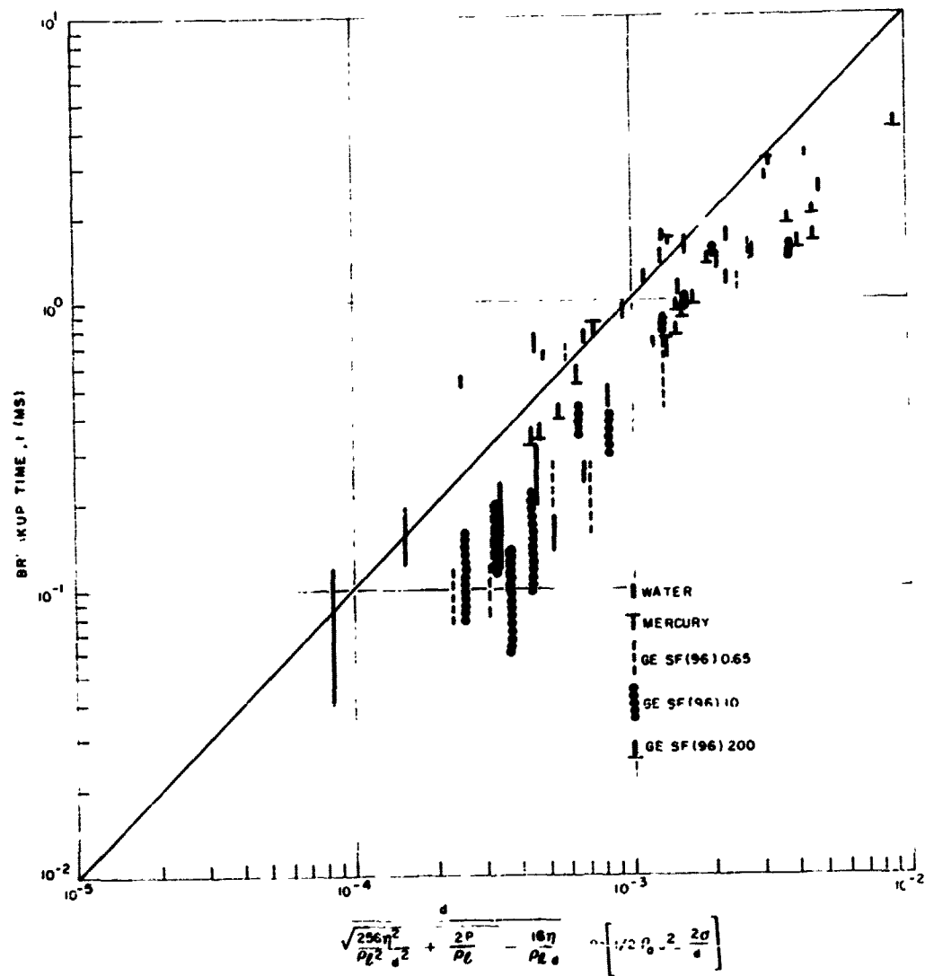
Figure 16. Comparison of Experimental Drop Breakup Times with Equation (46.)
