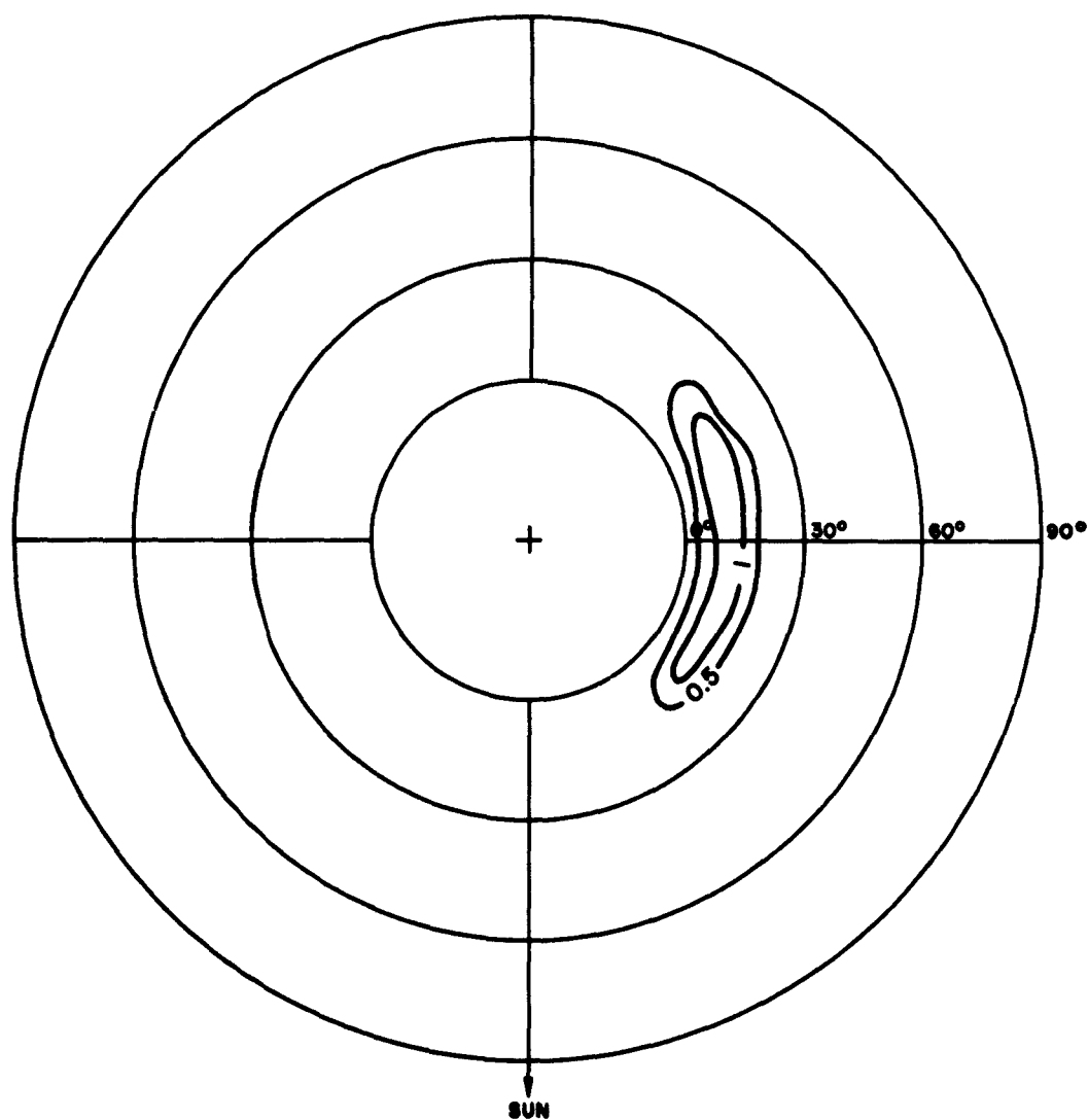
Figure 12. Isoradiance Plot (Means) Filter 2 Insolation Angle 50° Clouds All Values are in Microwatt \text{cm}^{-2} \text{ster}^{-1} As Viewed Through the Filter
