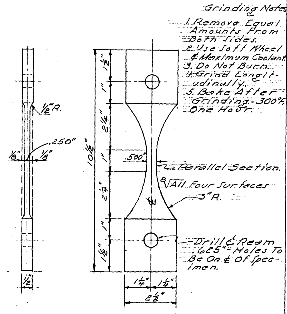
Transverse Weld Fatigue Specimen From 1/2" Plate
