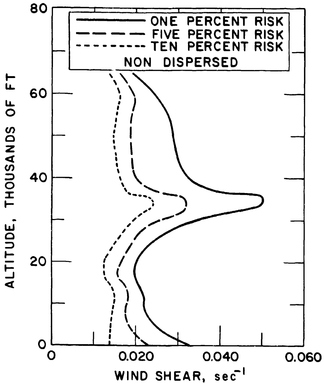
Figure 14. Design Wind Shear Envelope, 3000 Foot Shear Layer
