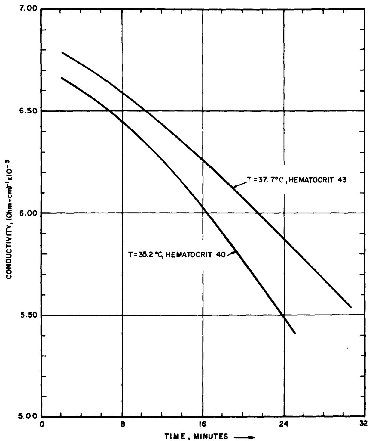
Figure 8. Variation of electrical conductivity in quiescent human blood with time.
