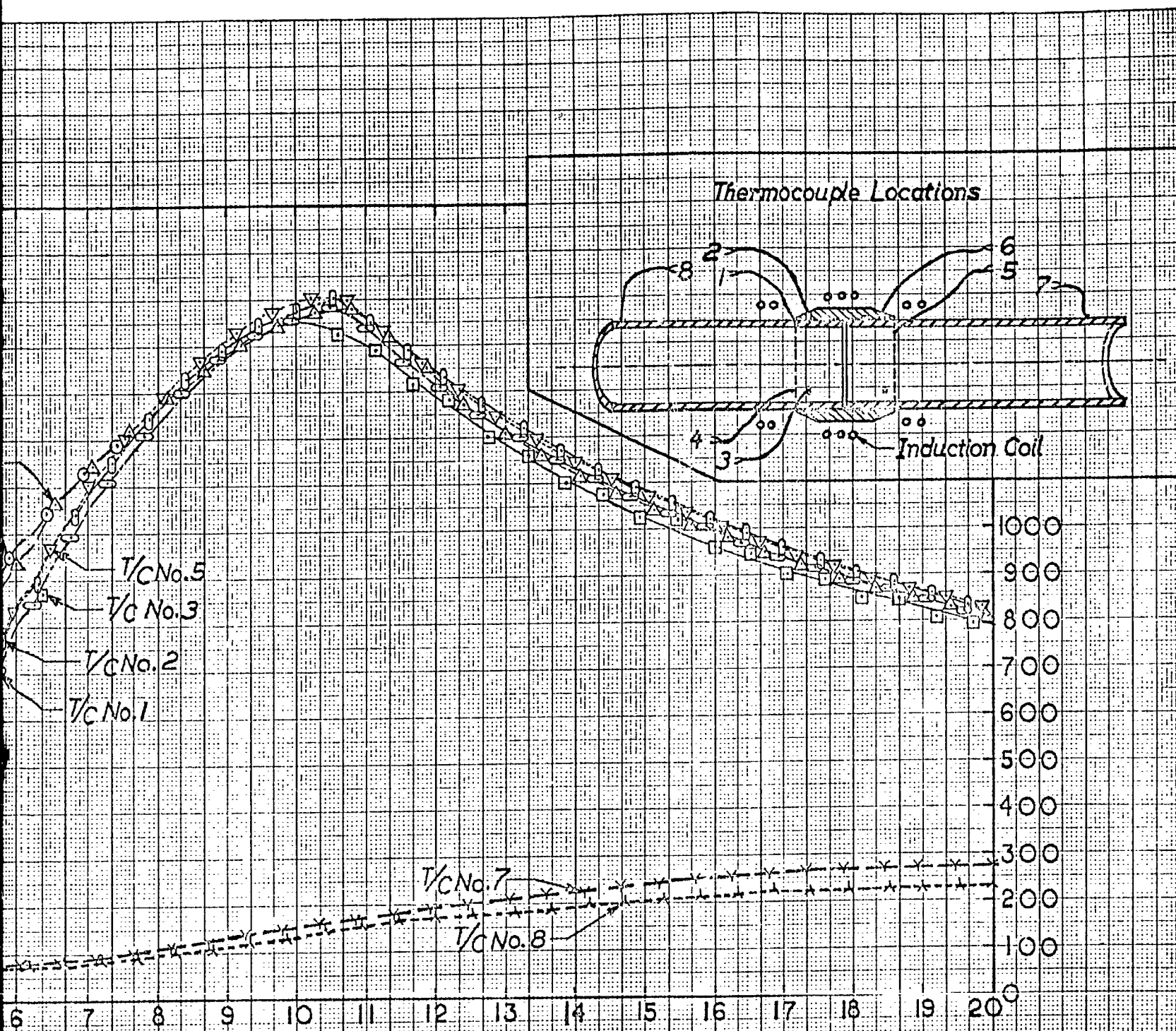
TEMPERATURE CYCLE FOR 3 INCH DIAMETER TYPE 347 STAINLESS STEEL BRAZED FITTING.
