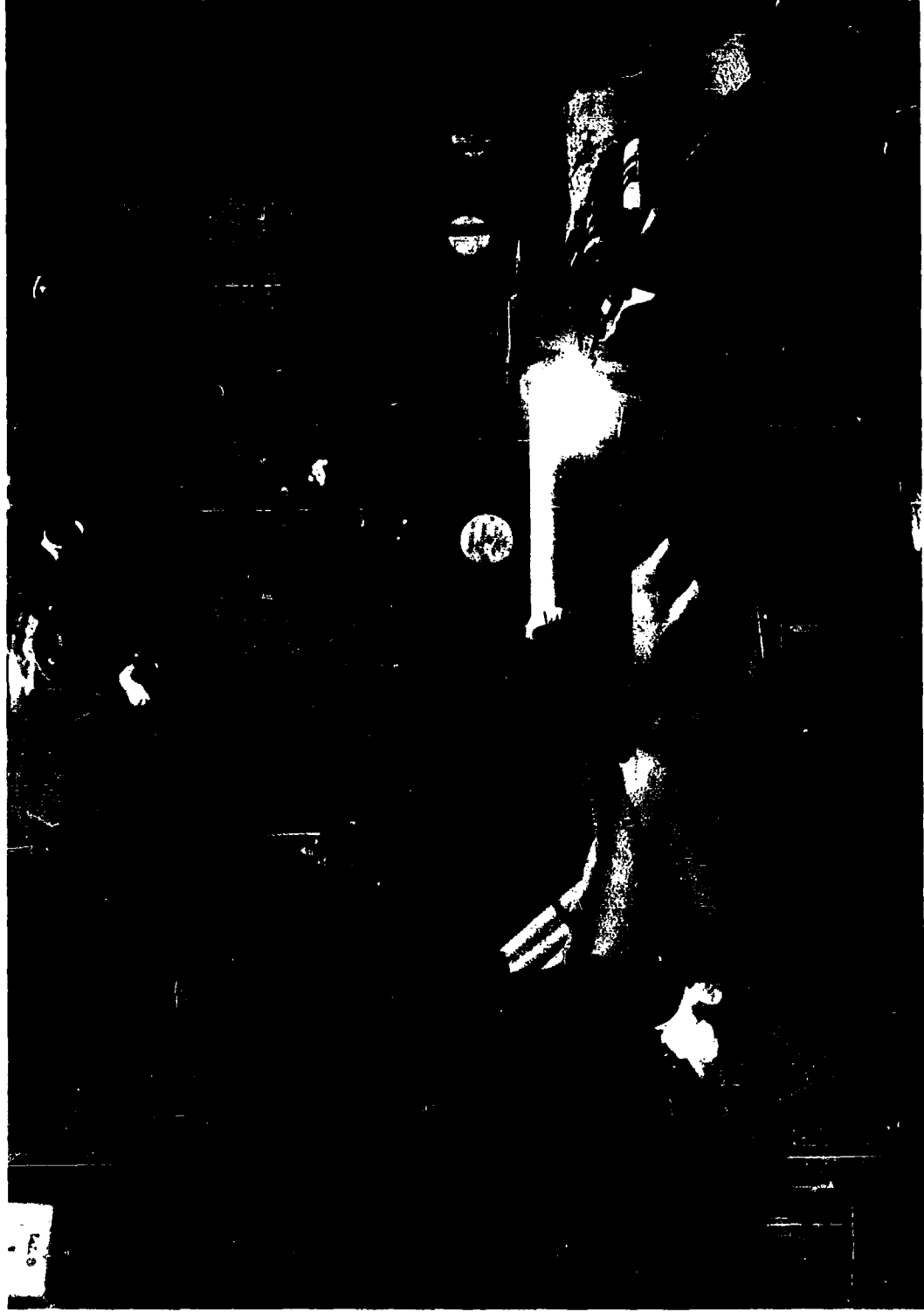
Figure 38. General View of Aluminum Tube Welding with "Bread Board" Tool Showing Hand Control of Current.
