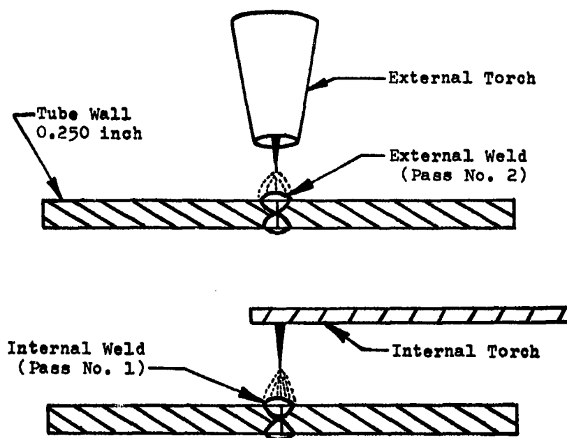
FIGURE 21 SCHEMATIC OF INTERNAL-EXTERNAL WELDING ARRANGEMENT
