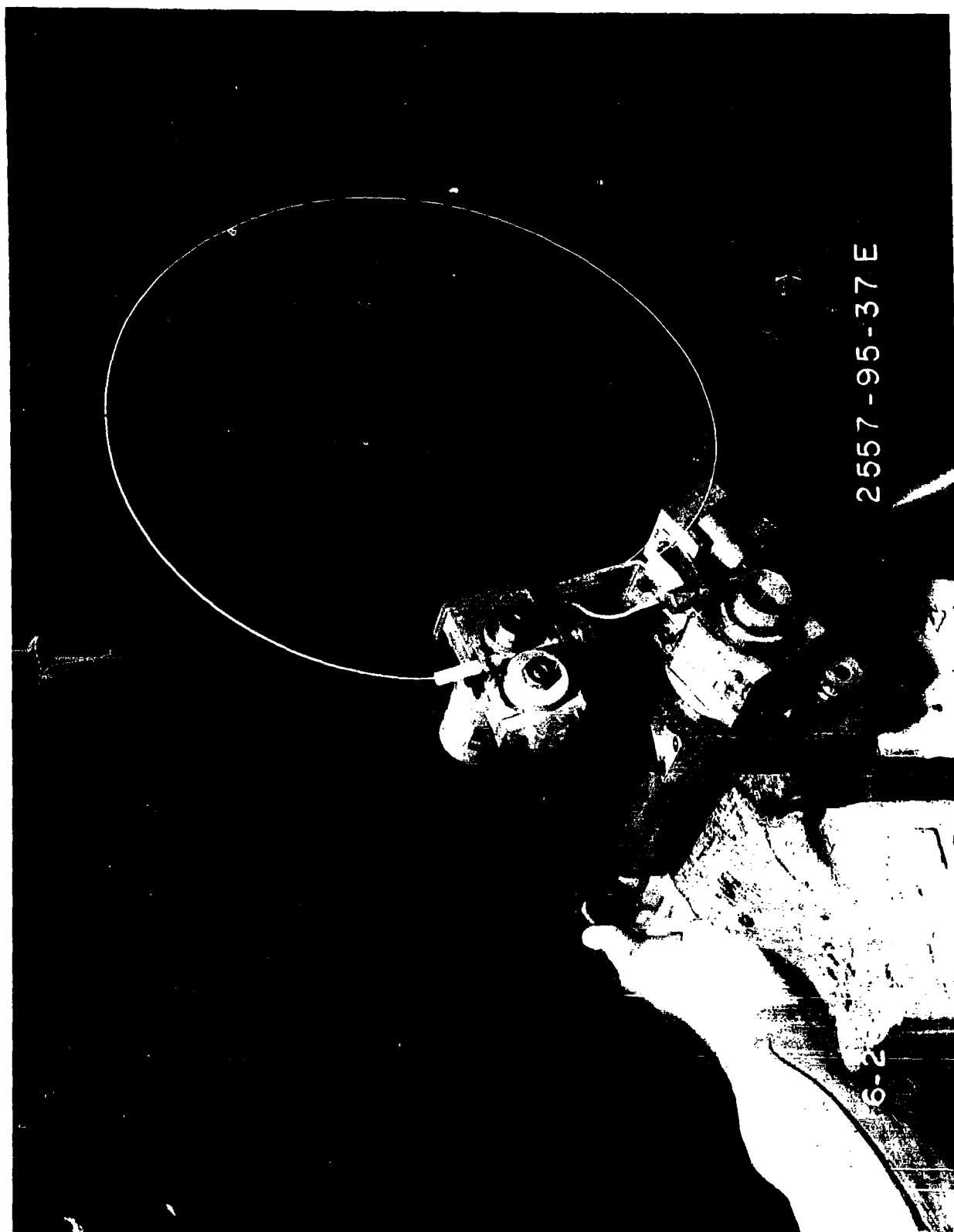
Aluminum Tube Welder and Wire Feed Mechanism
