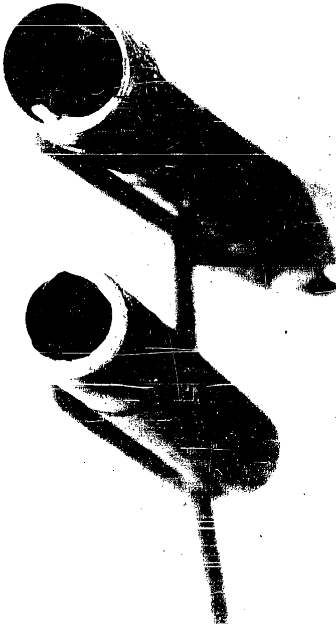
FIGURE 26. FRACTURED SURFACES SHOWING FATIGUE FAILURE MARKINGS. WELDED JOINT SPECIMEN OF 1/4 INCH DIAMETER AT 350 CRI STAINLESS STEEL TUBING TESTED IN STRESS REVERSAL ENDING AT 600 P.
