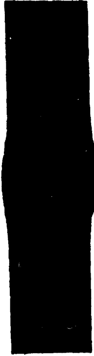
(a) Cross-Section Through Weld Joint (Note Internal and External Welds)
