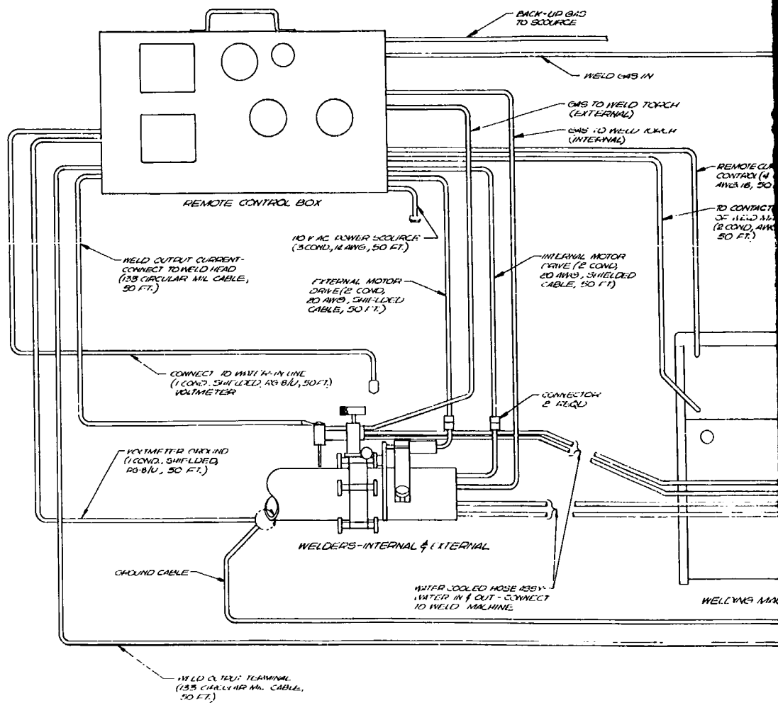
INTERCONNECTING DIAGRAM of REMOTE CONTROL NO SCALE
