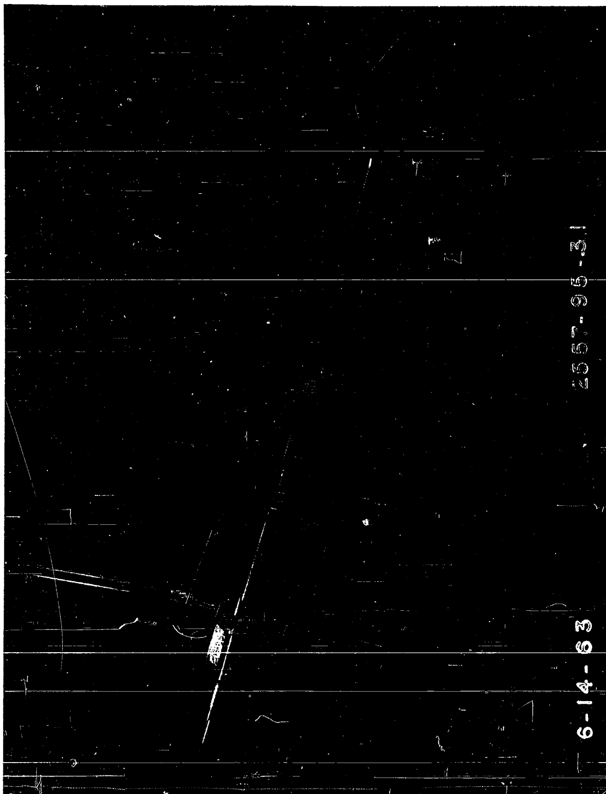
Figure 16. Section for Pressing 1/4 Inch Diameter M 390 Stainless Steel Tube Joint
