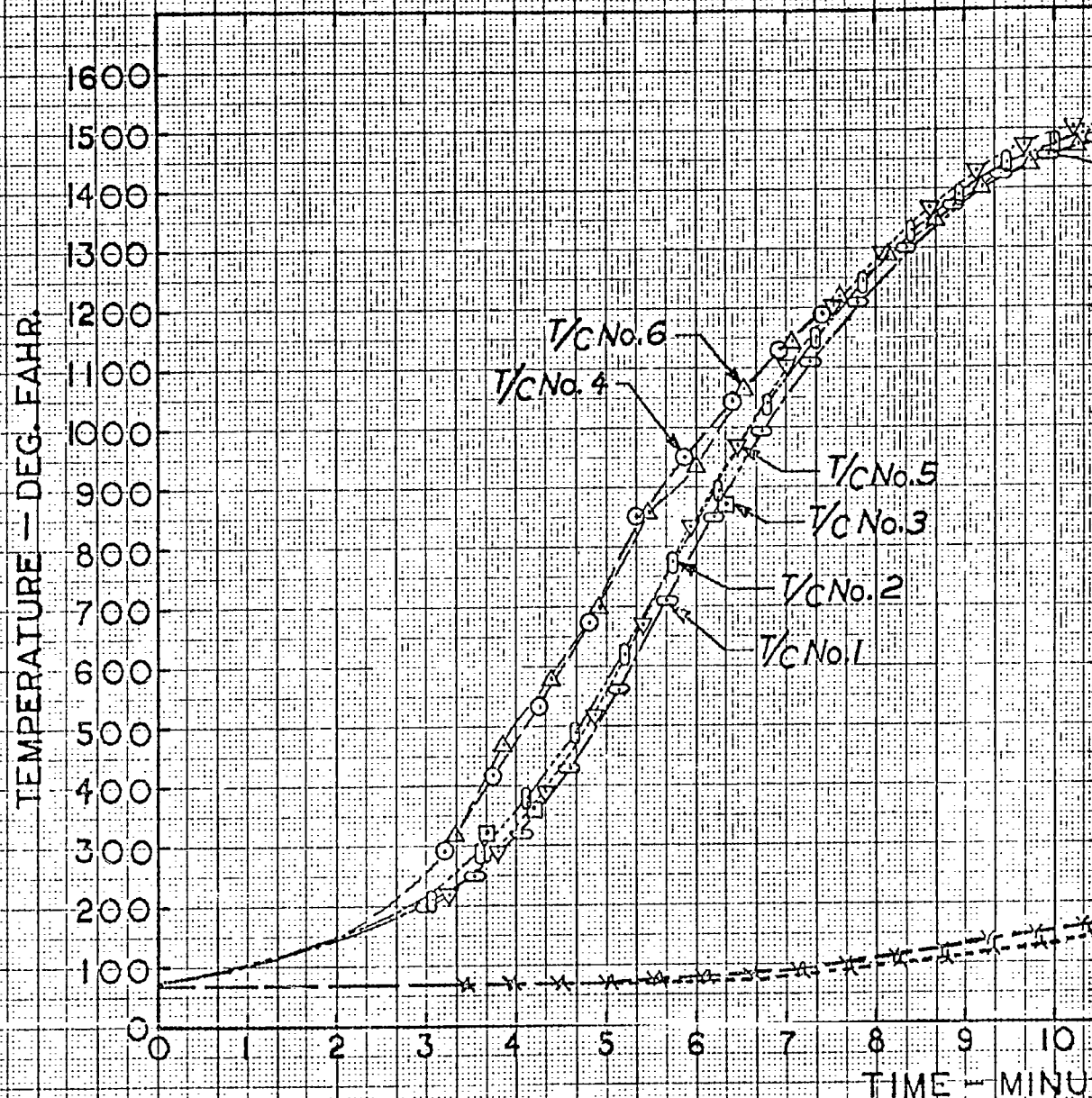
FIGURE 47. TEMPERATURE CYCLES AISI TYPE 347 STAINLESS STEEL
