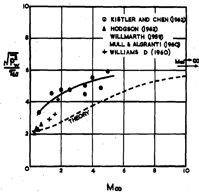
Fig.6 Wall pressure fluctuations in a turbulent boundary layer; M_\infty = freestream Mach number
