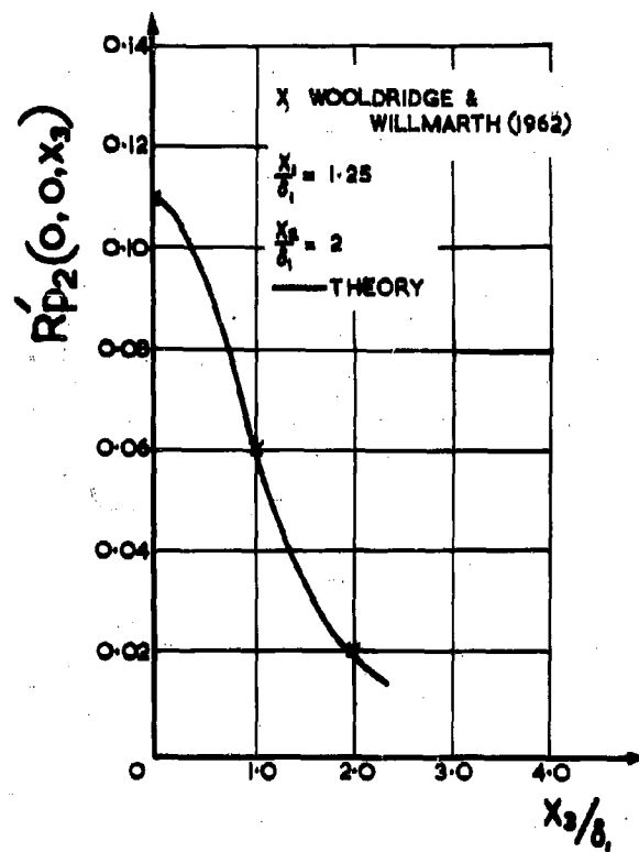
Fig.2 Correlation coefficient R'_{p_2} ; variation with x_3/\delta_1
