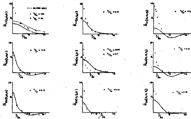
Fig.4 Comparison between theoretical and experimental velocity correlations (experimental points Grant (1958) - big eddy model)
