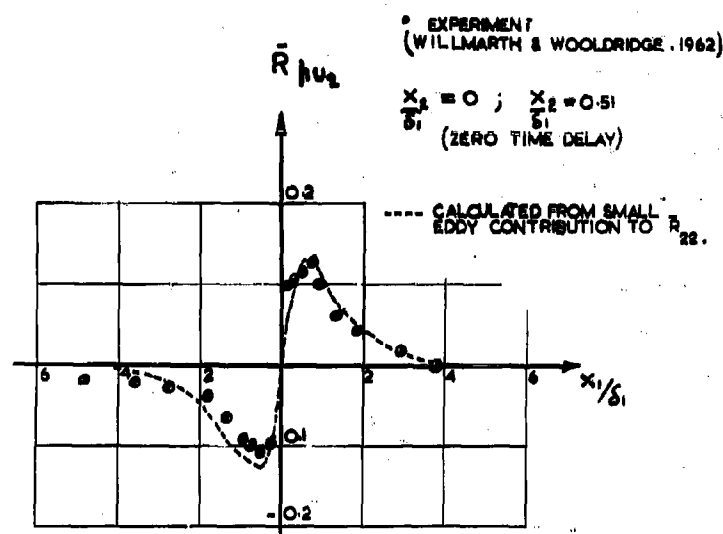
Fig.1 Comparison between calculated and measured correlation coefficient \bar{R}_{pu_2}
