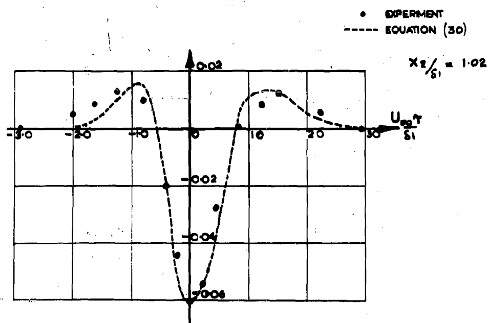
Fig. 3 Comparison between measured (Willmarth and Wooldridge 1962) and assumed values for the correlation coefficient R_p u_2 / x_1 with zero time delay
