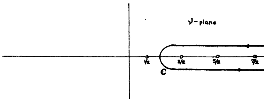
Fig. 3-2 Contour for Watson transformation
