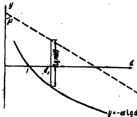
Fig. 72. Method of rectifying the plot of the density of the gamma distributions in coordinates d; \lg n . Here the parameter is \beta = \text{tg } \mu .
