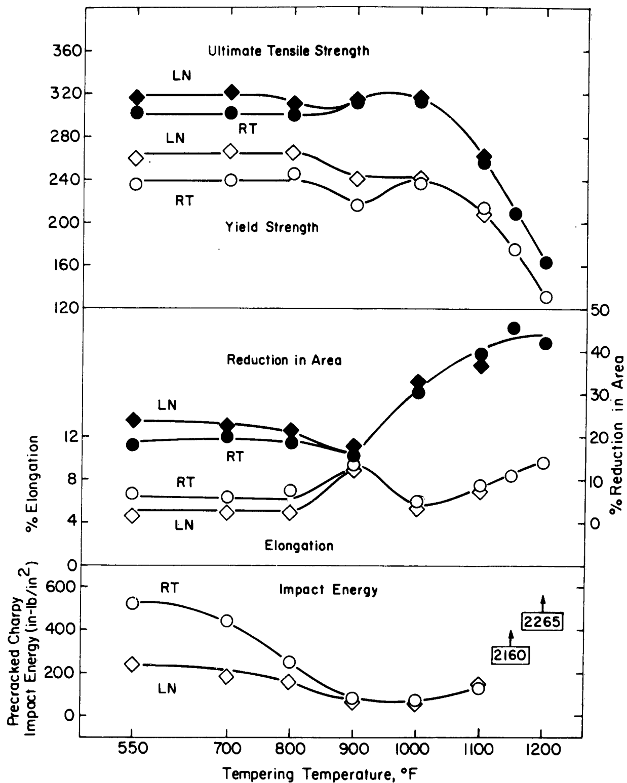
Fig.9—Mechanical properties of H II as a function of tempering temperature ( T^T ) for process M. ( T^A=1850^\circ\text{F} , T^Q=\text{RT} or LN).
