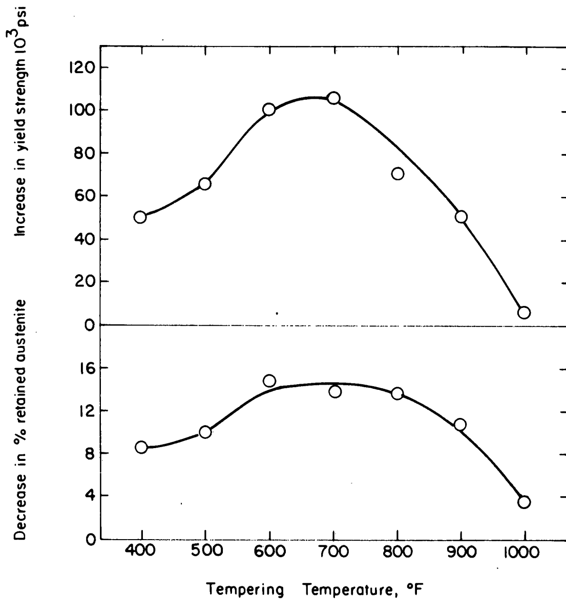
Fig.24-Effect of refrigeration treatment (LN) on yield strength and retained austenite content of H 11 subjected to process AB. ( T^A=1850^{\circ}\text{F} T^B=900^{\circ}\text{F} deformation 50% T^B=550^{\circ}\text{F} t_f=4 hours T^Q=\text{RT or LN} ).
