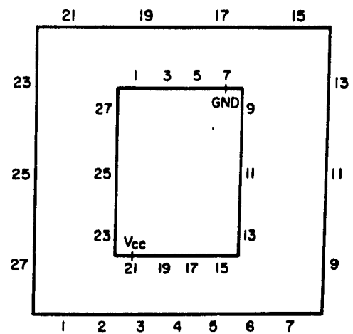
POSITION (4) (90° CL ROTATION OF ICP)
