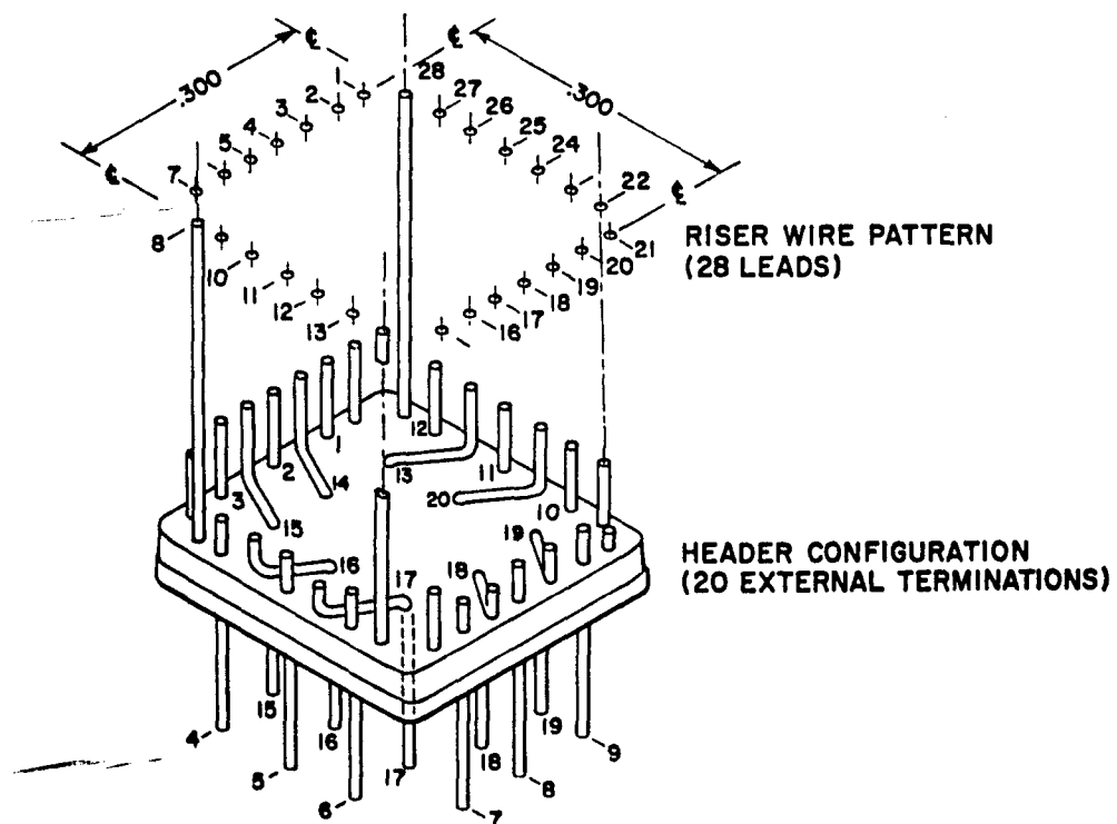
Figure 4-3. 28/20 Integrated Circuit Module (ICM): Exploded View Showing Internal Construction
