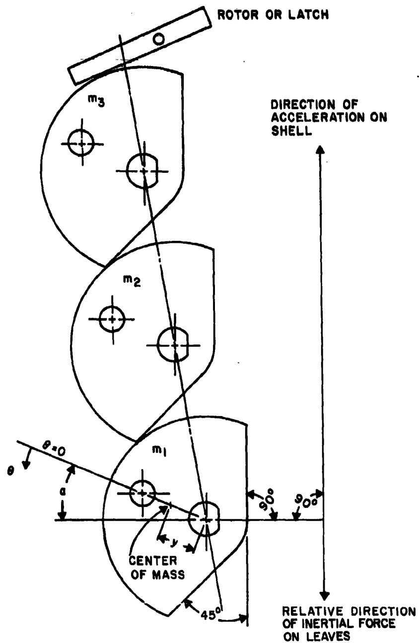
Figure 1. Leaf arrangement in setback mechanism.
