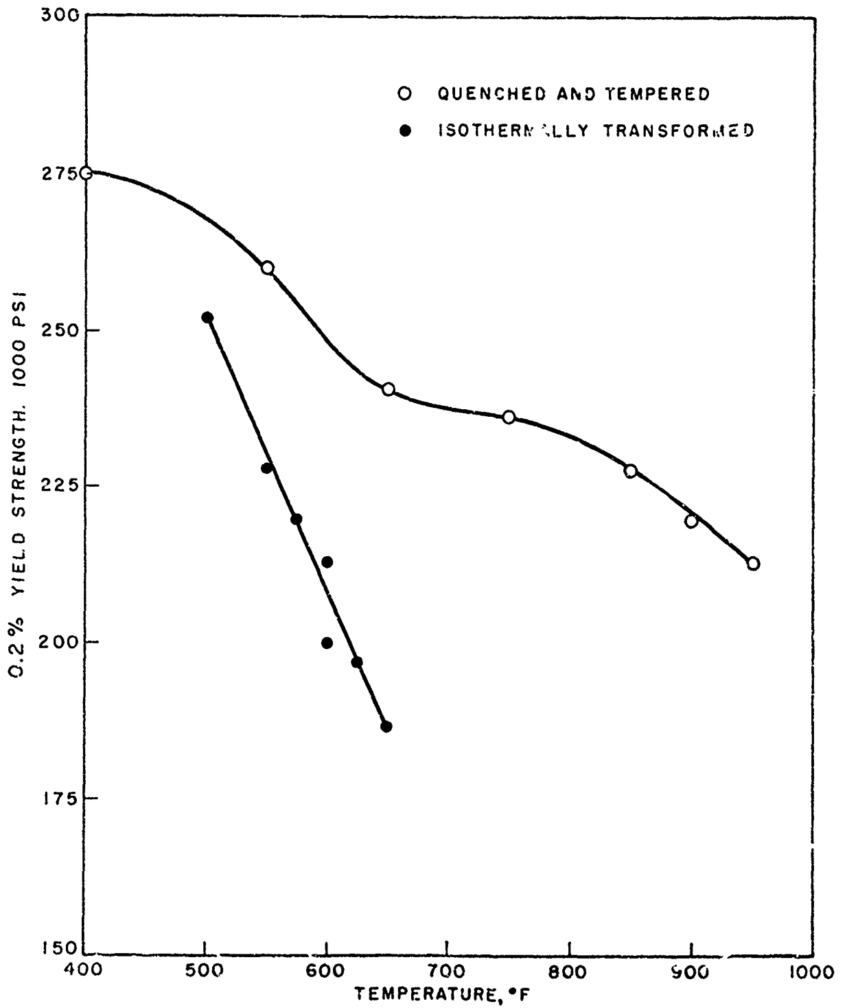
FIG. 1 - THE 0.2% YIELD STRENGTH AS A FUNCTION OF TEMPERING OR ISOTHERMAL TRANSFORMATION TEMPERATURE FOR THE 1Cr-1Mo STEEL.
