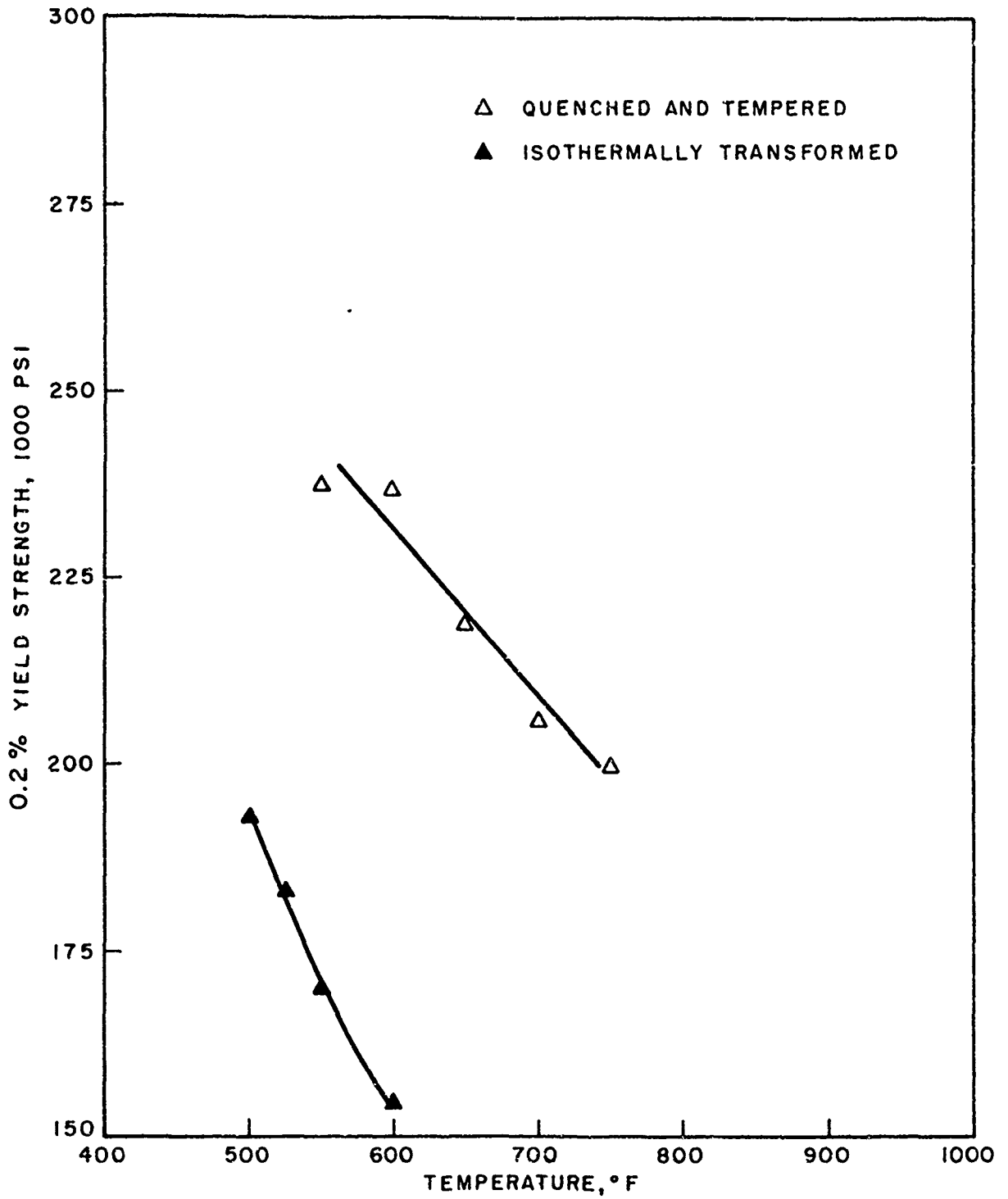
FIG. 6 - THE 0.2% YIELD STRENGTH AS A FUNCTION OF TEMPERING OR ISOTHERMAL TRANSFORMATION TEMPERATURE FOR THE 9Ni-4Co STEEL.
