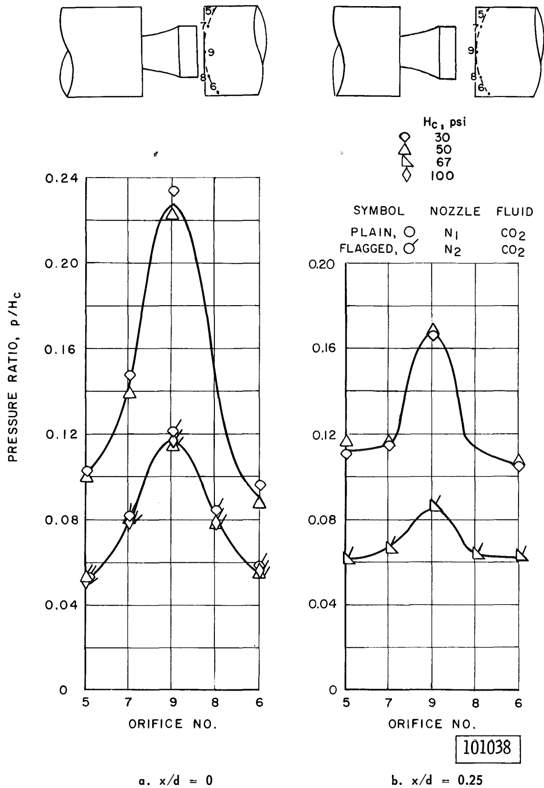
Fig. 8 Lower Stage Static Pressure Distribution, C_{2a} Configuration
