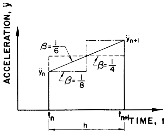
FIG. V-4.12 CONSISTENT VARIATIONS OF ACCELERATION WITH \beta IN A TIME INTERVAL
