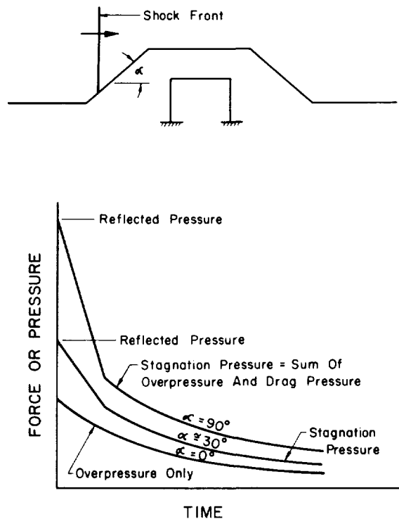
FIG. V-2.7 PRESSURES ACTING ON WINDWARD FACE OF SOIL MOUNDED OVER A STRUCTURE
