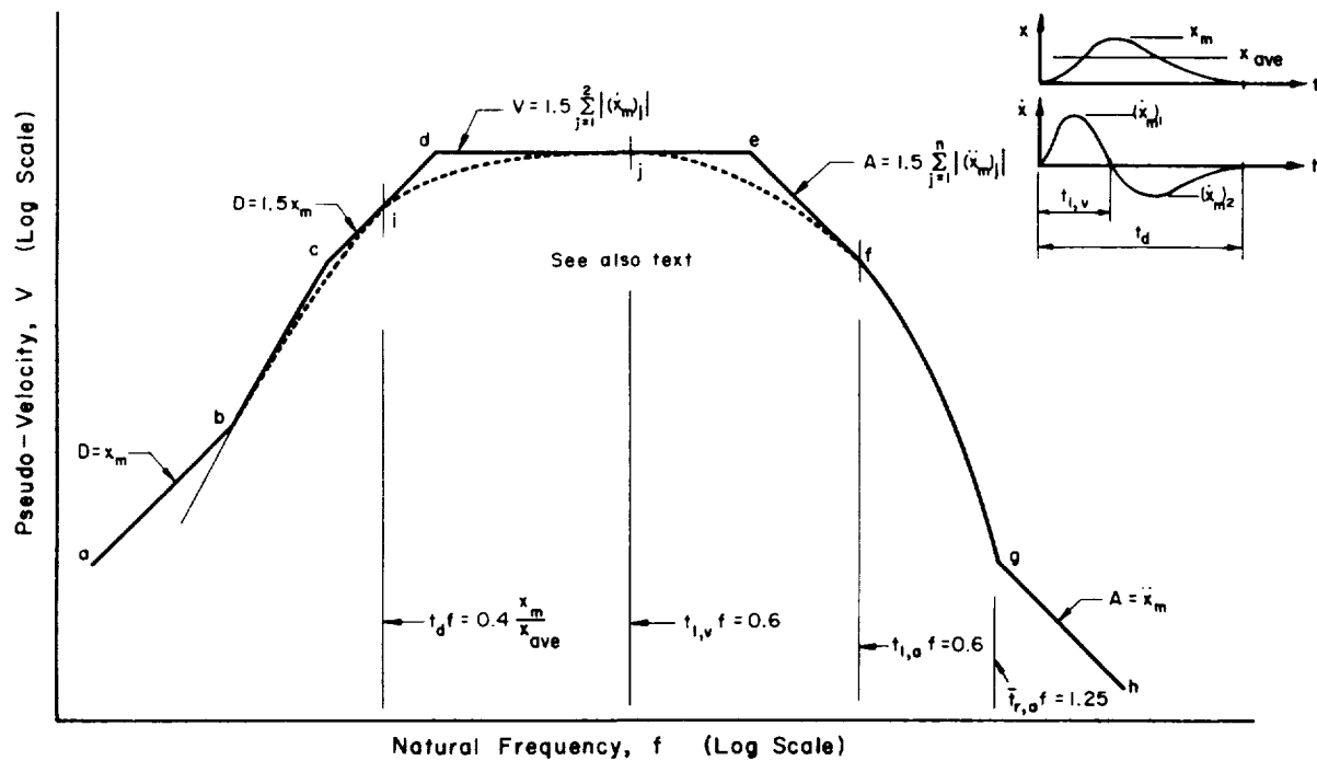
FIG. X-4.20b DESIGN SPECTRUM FOR THE ABSOLUTE MAXIMUM DEFORMATION OF SYSTEMS SUBJECTED TO A HALF-CYCLE DISPLACEMENT PULSE—UNDAMPED ELASTIC SYSTEMS; CONTINUOUS INPUT ACCELERATION FUNCTIONS
