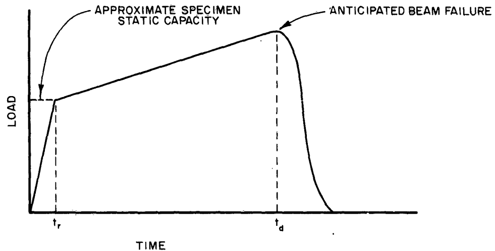
FIG. 3.2. SHAPE OF LOAD PULSE USED IN EXPERIMENTAL STUDY
