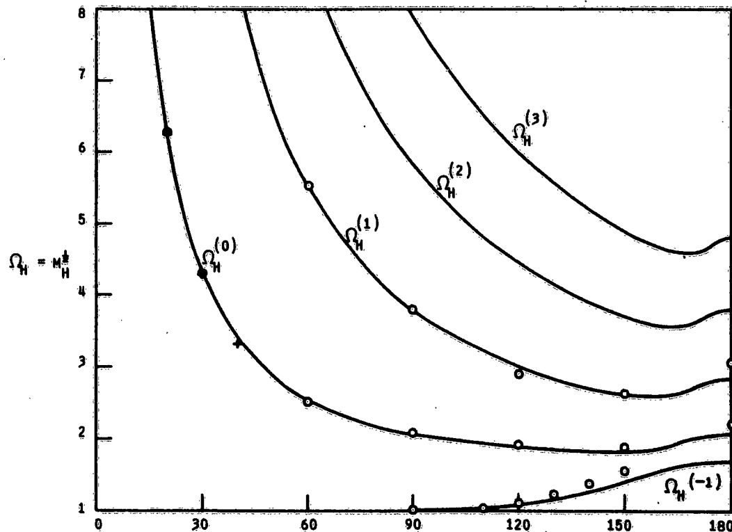
Figure 4. DEPENDENCE OF NATURAL FREQUENCY, \Omega = \omega R/\sqrt{E/\rho} , ON SEMI-ANGLE, \alpha , FOR THE FIVE LOWEST BRANCHES OF THE UPPER FAMILY, \Omega_H . ○ AND + DENOTE POINTS GIVEN BY THE APPROXIMATION (46) FOR HIGH \lambda -VALUES AND (61) FOR SHALLOW SHELLS, RESPECTIVELY.
