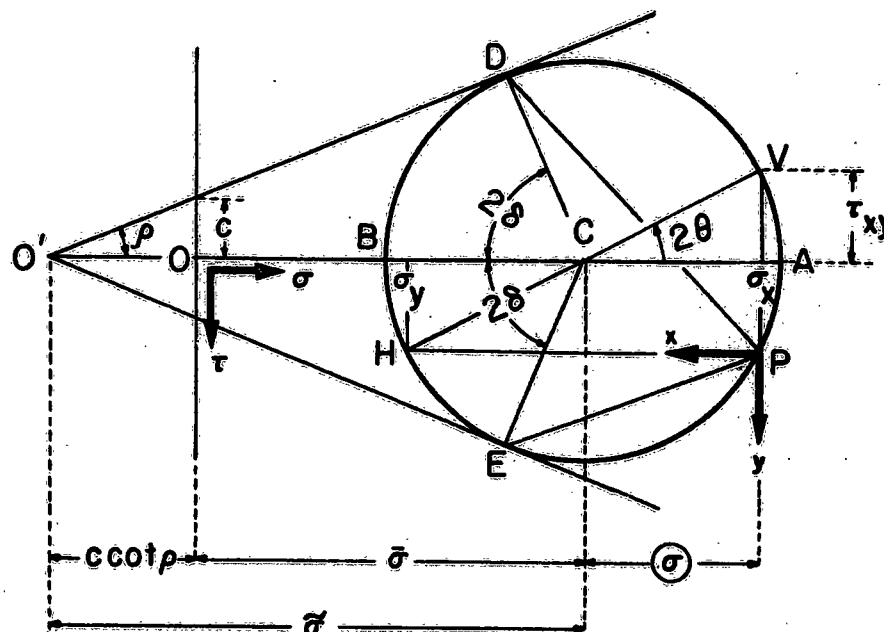
FIG. 3.—STRESS CHARACTERISTIC DIRECTIONS
