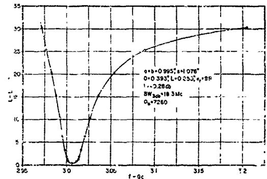
Figure 5-2. Maximally Flat Dielectric-Resonator Filter, a = b = 0.995''
