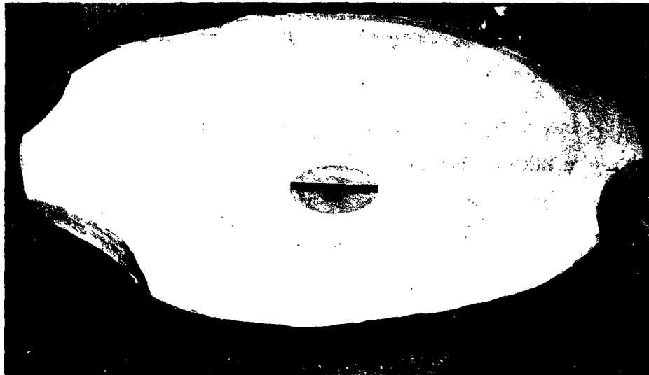
Figure 100. Female Mold Used to Form Inflatable Lenticular Antenna Model Surface
