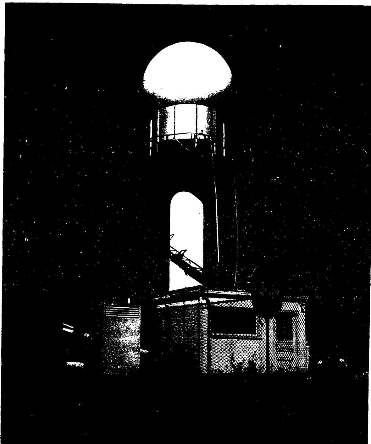
Figure 54. Seventeen-Foot-Diameter Monolithic Foam Radome Utilizing Bonded Joints
