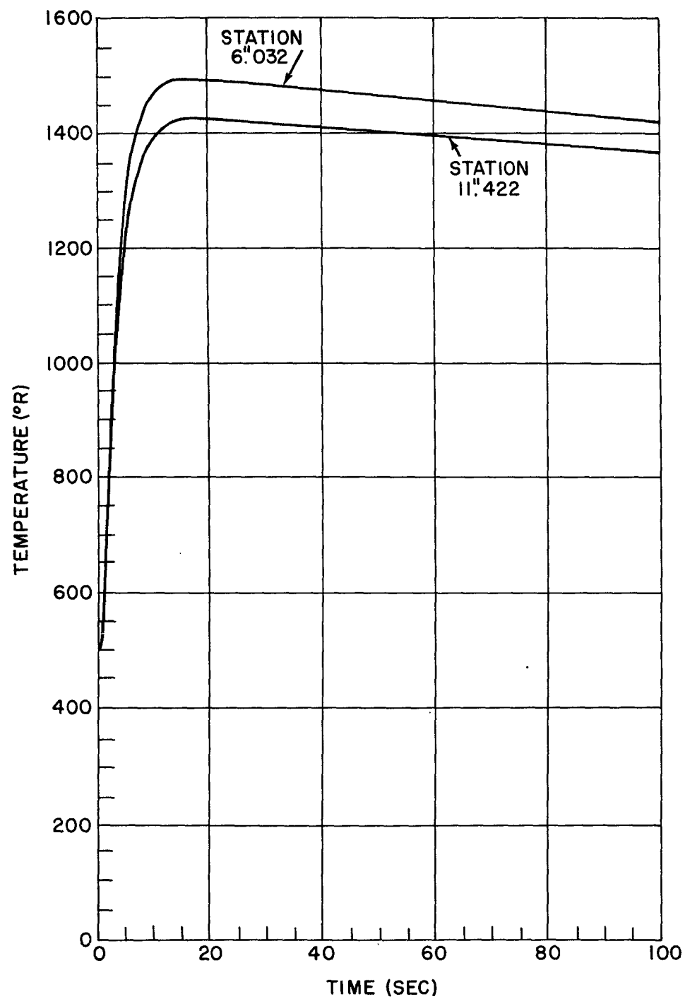
FIG.10 NOSE CONE TEMPERATURE AS A FUNCTION OF TIME
