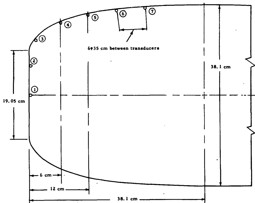
FIG. 5. Pressure Transducer Stations in Bare-Body Nose.
