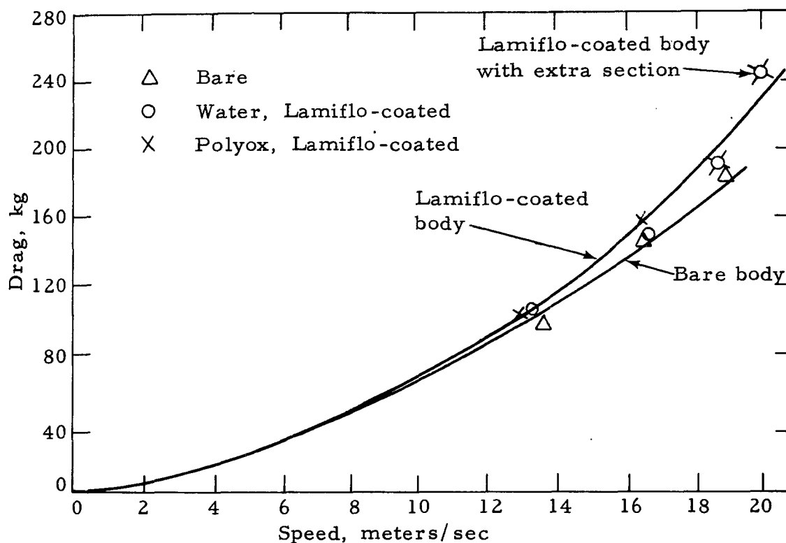
FIG. 8. Drag Versus Speed of Lamiflo-Coated and Bare Body.
