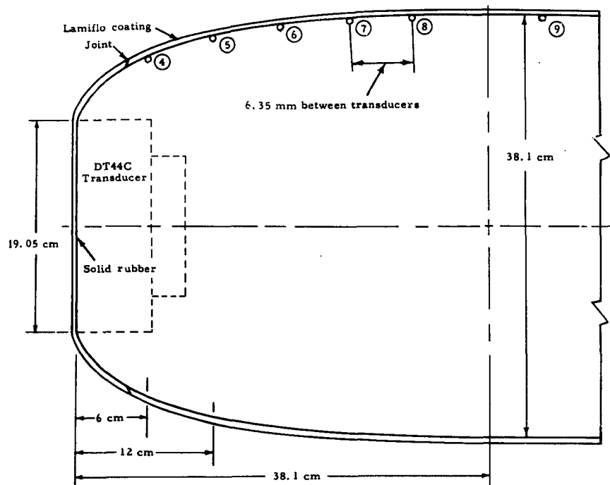
FIG. 4. Pressure Transducer Stations in the Lamiflo-Body Nose.
