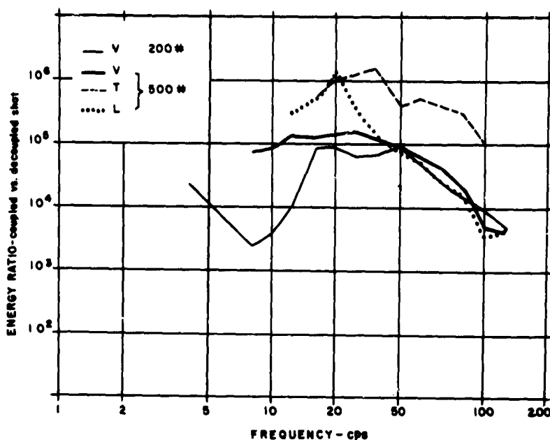
FIGURE 22. OBSERVED ENERGY RATIOS FOR A 200-lb PAIR AND A 500-lb PAIR OF COUPLED AND DECOUPLED SHOTS (CAVITY RADIUS = 15 FEET) RECORDED AT A DISTANCE OF 1.1 km [87]
