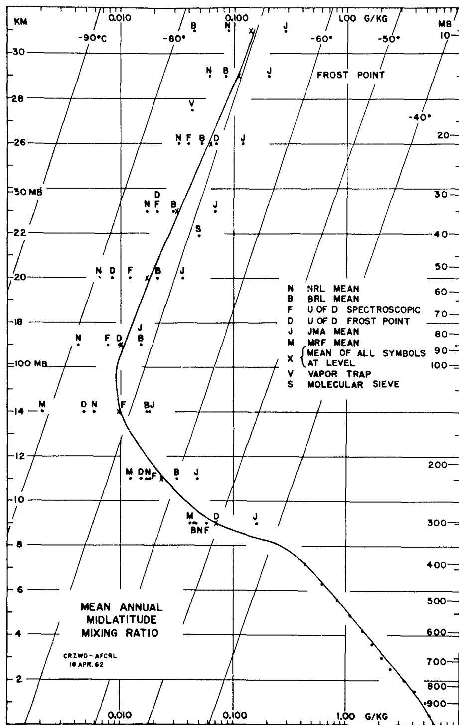
Fig. 5. — The Gutnick model for stratospheric water vapor.
