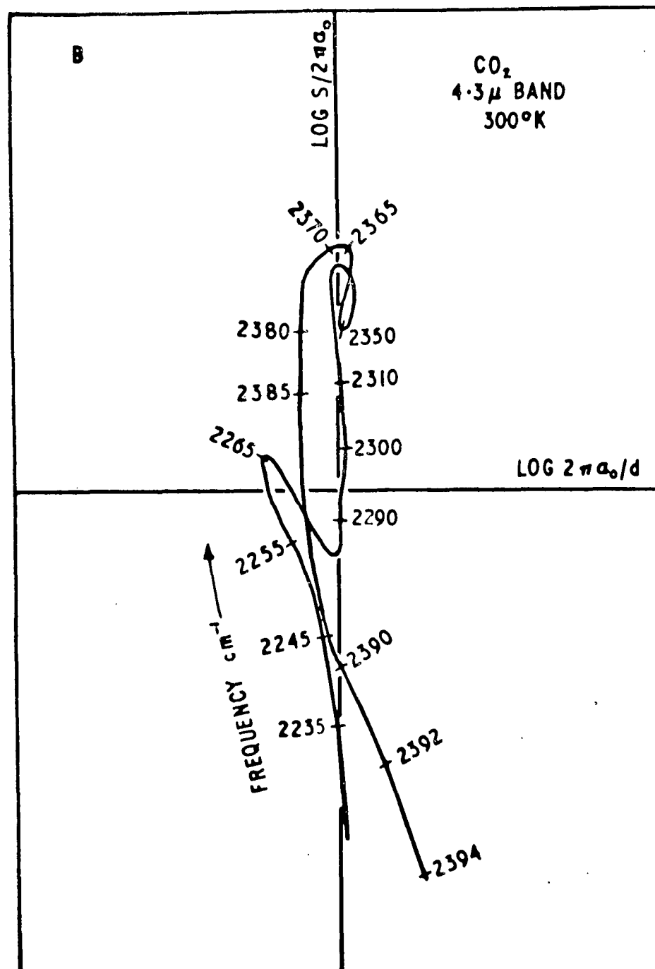
Fig. 11. — Generalized coefficients for the 4.3 micron CO 2 band.
