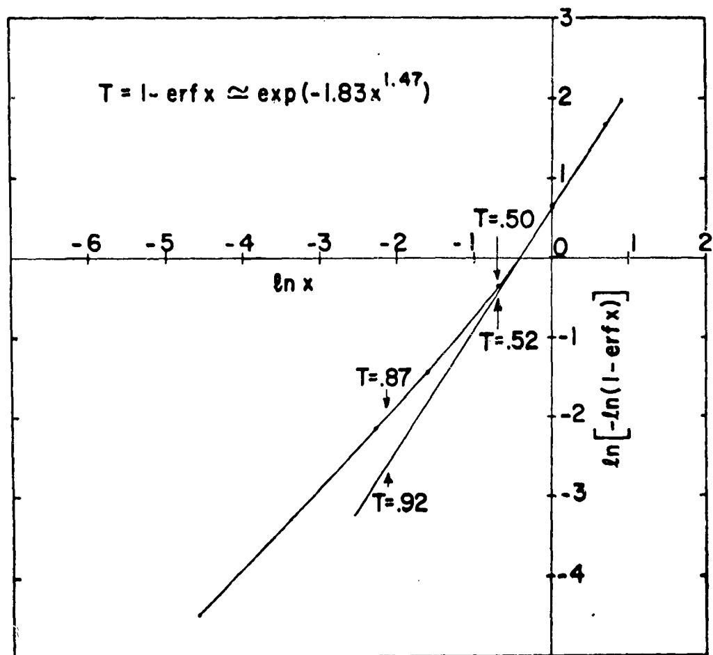
Fig. 21. — The exponential approximation to the Elsasser error function.
