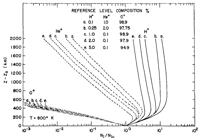
Fig. 9b. Dependence of the vertical profiles of the ionic constituents O^+ , He^+ , and H^+ on reference-level composition for T = 800^\circ K .
